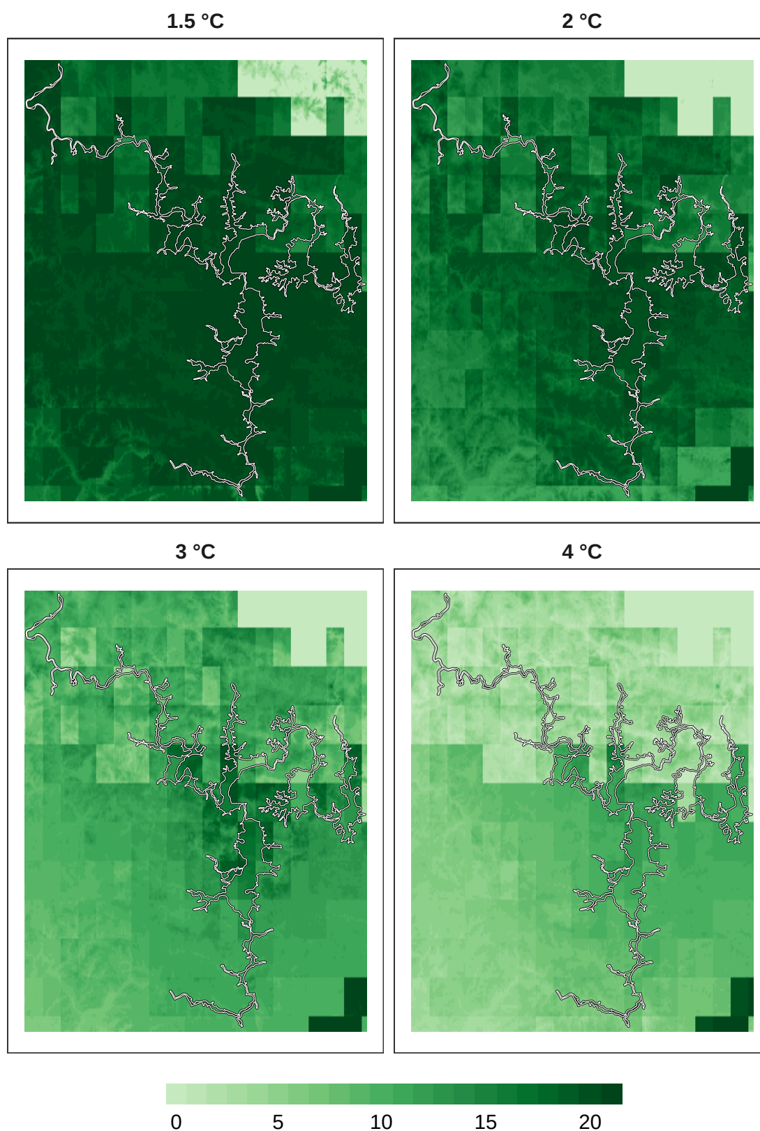
Figure 3: Number of models in agreement for overall biodiversity refugia at 1 km resolution.
