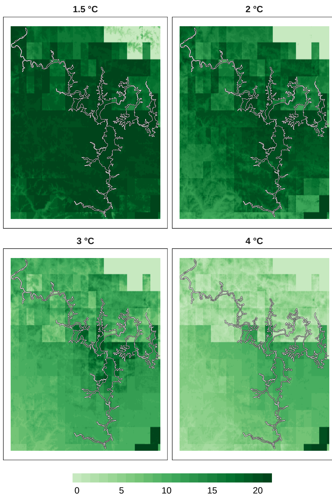
Figure 4: Number of models in agreement for mammal refugia at 1 km resolution.
