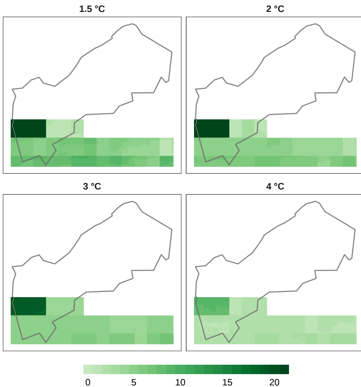
Figure 14: Number of models in agreement for pollinator refugia at 1 km resolution.
