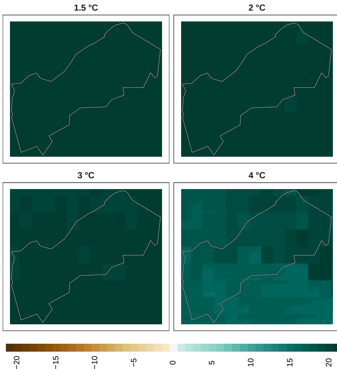
Figure 19: Adaptation effort for reptiles at 1 km resolution.
