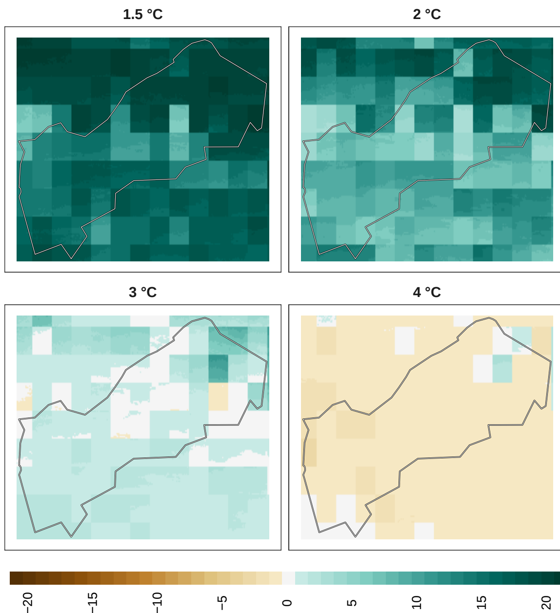
Figure 20: Adaptation effort for insects at 1 km resolution.
