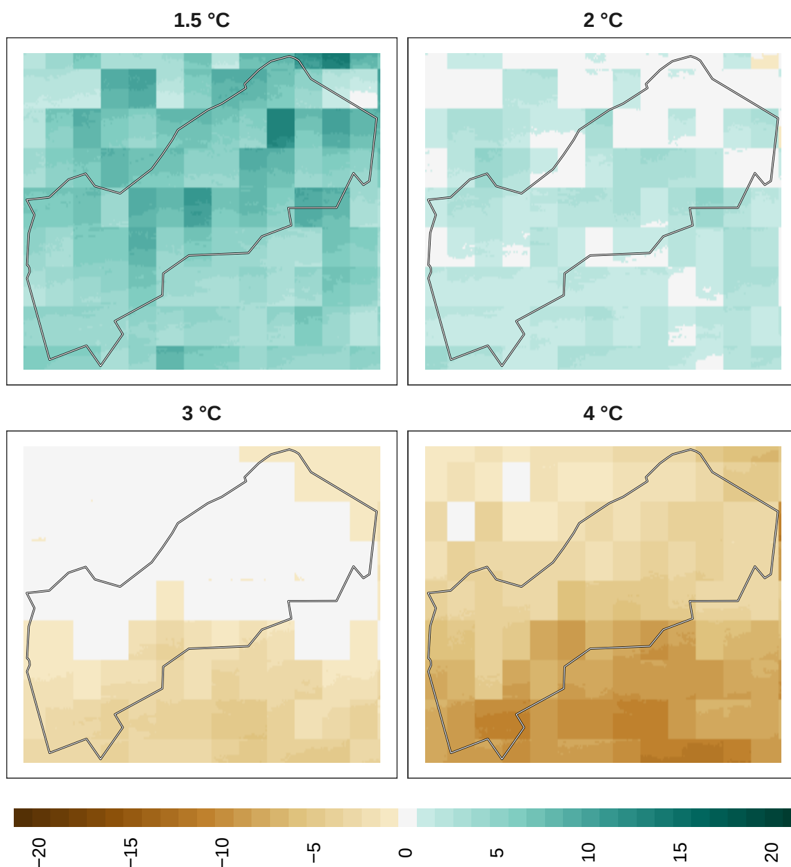
Figure 16: Adaptation effort for plants at 1 km resolution.
