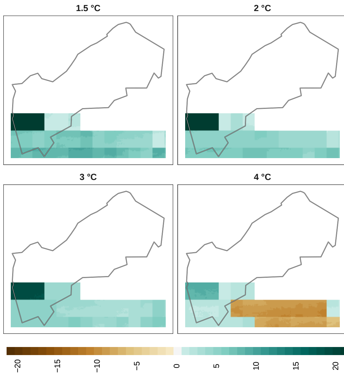
Figure 21: Adaptation effort for pollinators at 1 km resolution.
