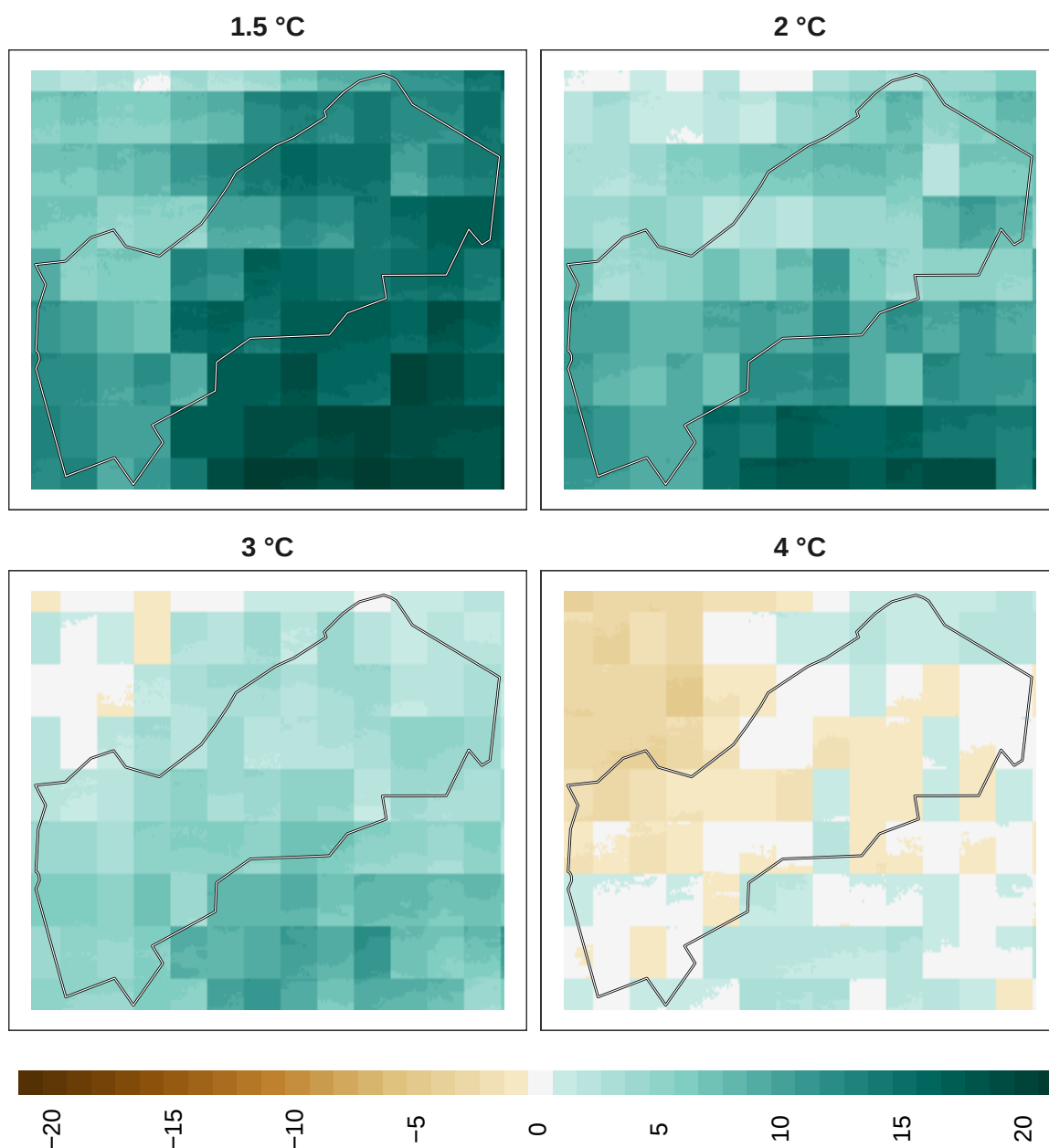
Figure 17: Adaptation effort for birds at 1 km resolution.
