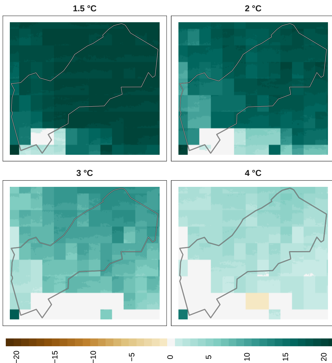
Figure 18: Adaptation effort for mammals at 1 km resolution.
