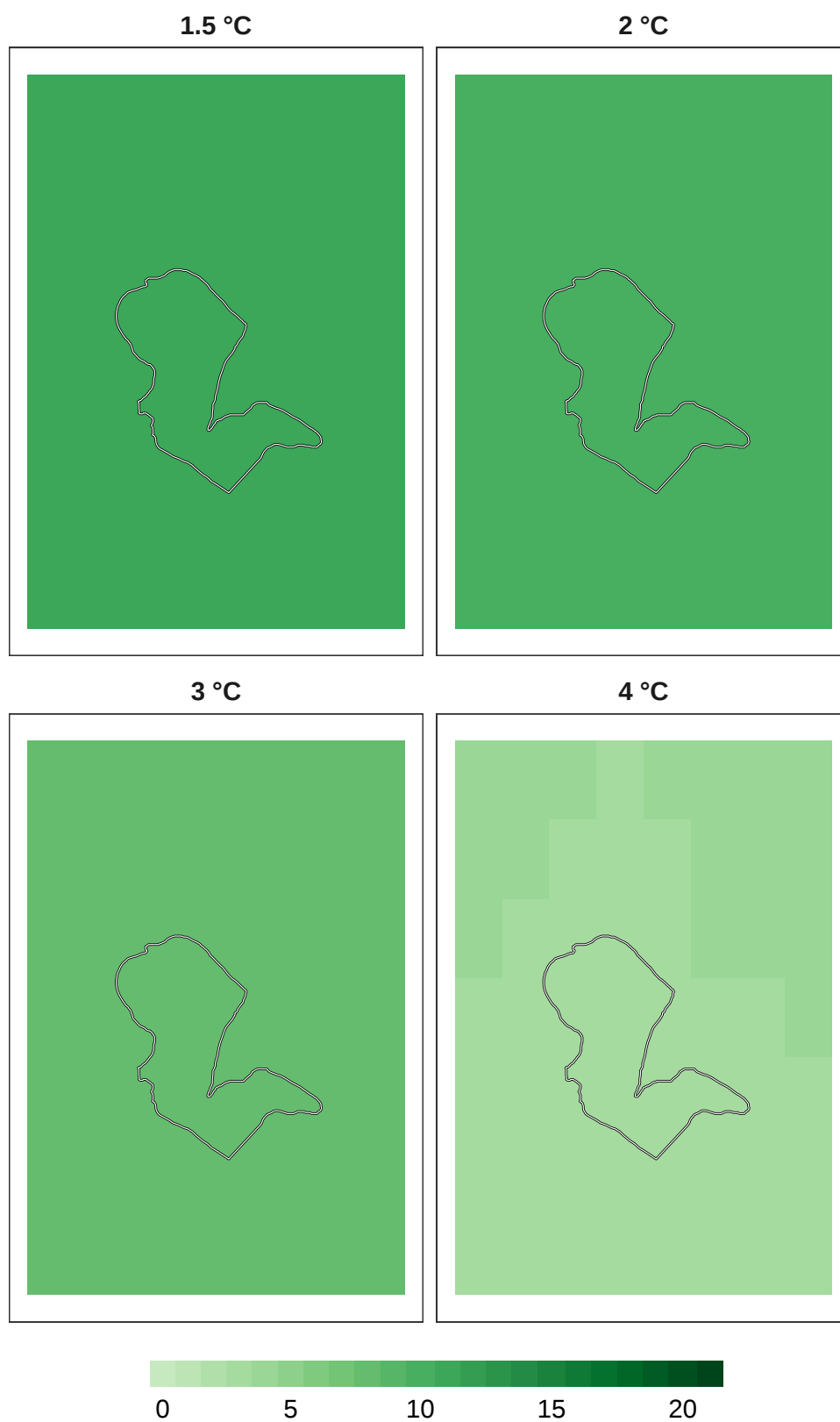
Figure 11: Number of models in agreement for reptile refugia at 1 km resolution.
