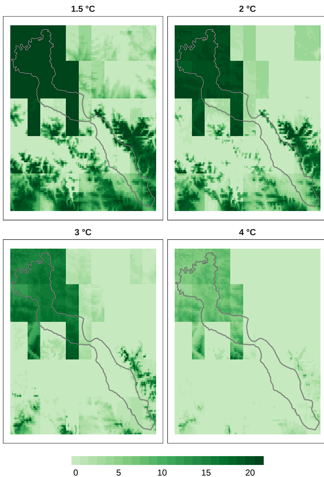
Figure 4: Number of models in agreement for plant refugia at 1 km resolution.
