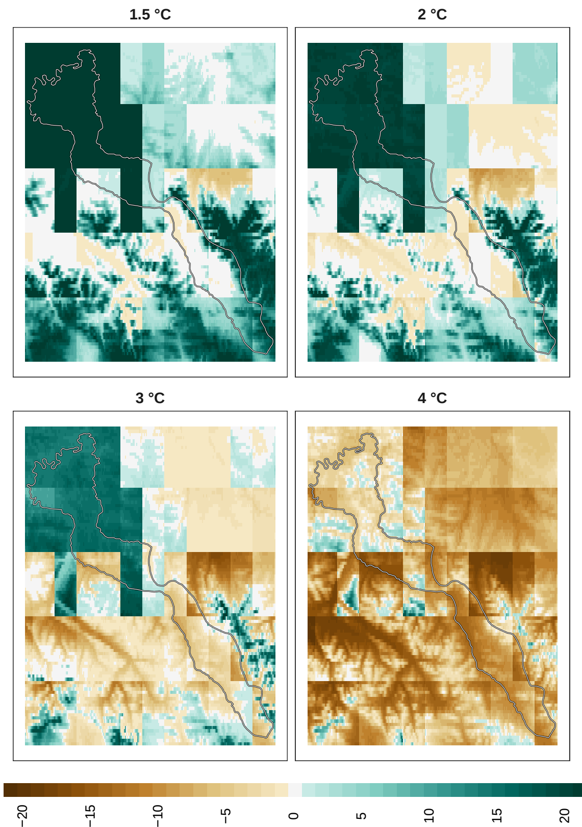
Figure 6: Adaptation effort for plants at 1 km resolution.
