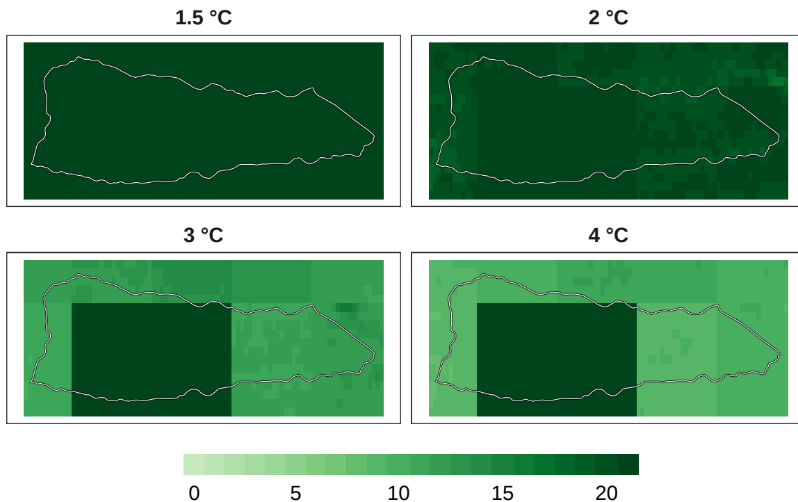
Figure 3: Number of models in agreement for overall biodiversity refugia at 1 km resolution.
