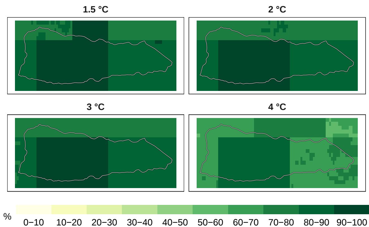
Figure 2: Percent mammals remaining at 1 km resolution.
