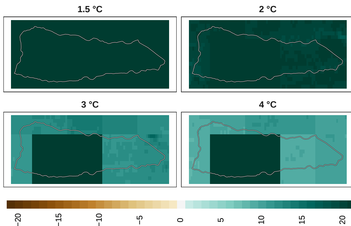
Figure 5: Adaptation effort for overall biodiversity at 1 km resolution.
