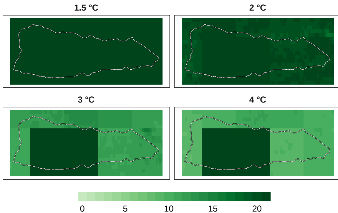
Figure 4: Number of models in agreement for mammal refugia at 1 km resolution.
