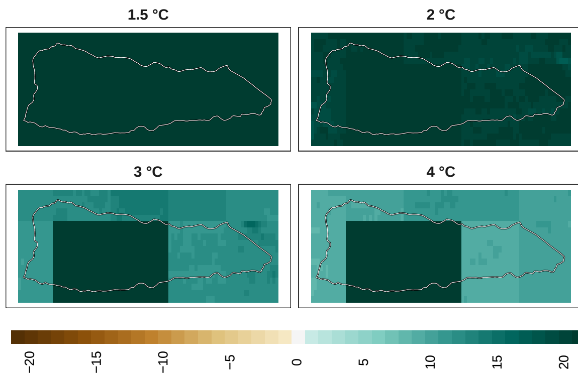
Figure 6: Adaptation effort for mammals at 1 km resolution.
