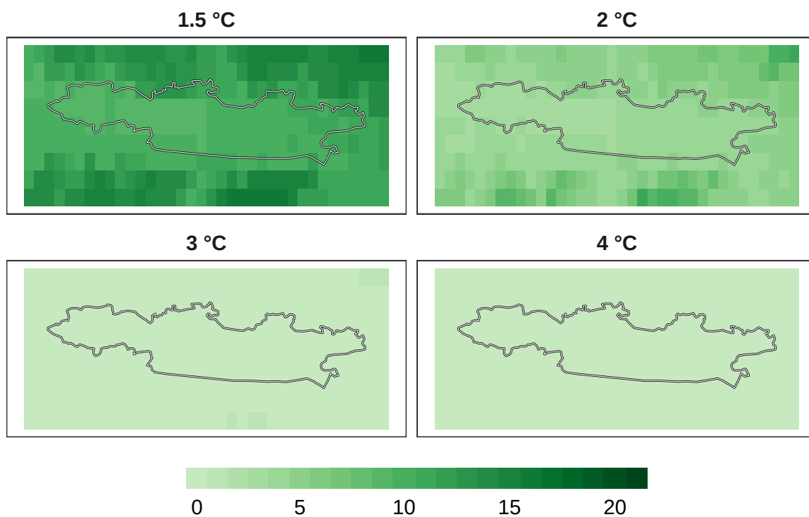
Figure 8: Number of models in agreement for overall biodiversity refugia at 1 km resolution.
