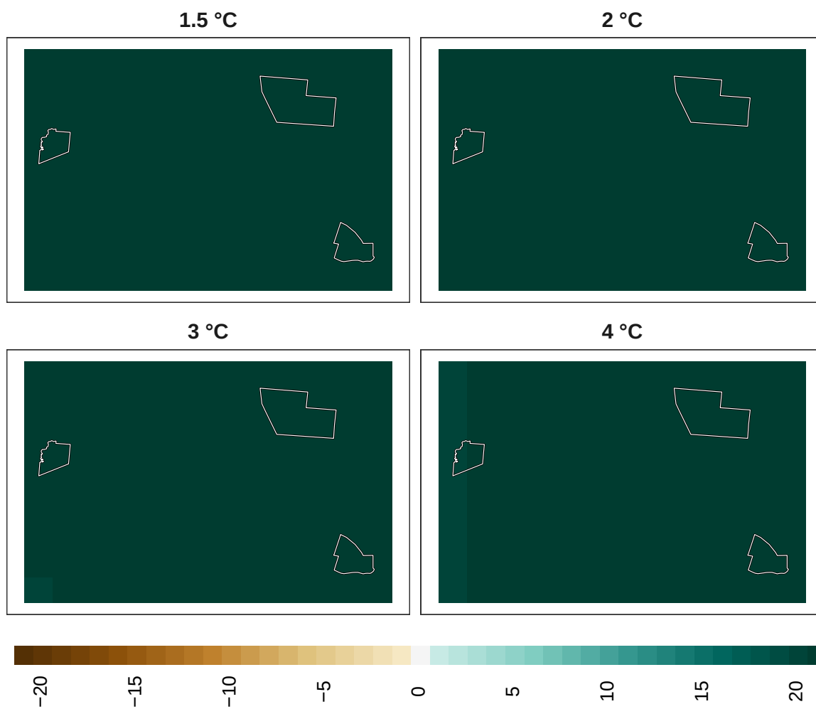
Figure 13: Adaptation effort for birds at 1 km resolution.
