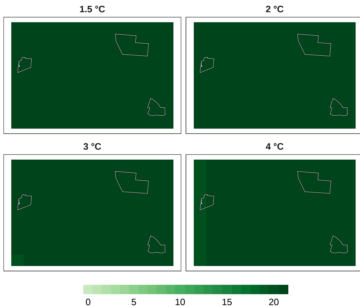
Figure 8: Number of models in agreement for bird refugia.
