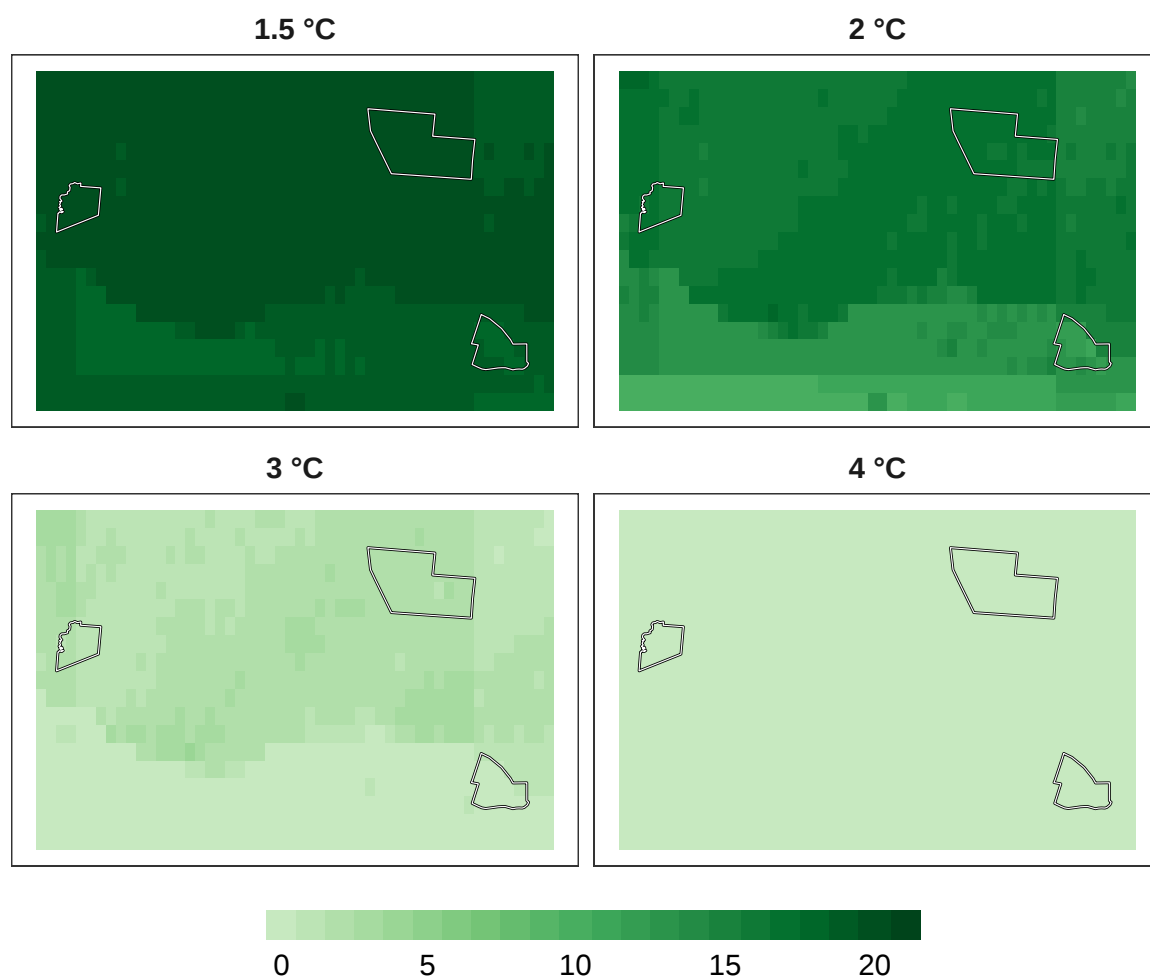
Figure 9: Number of models in agreement for mammal refugia at 1 km resolution.
