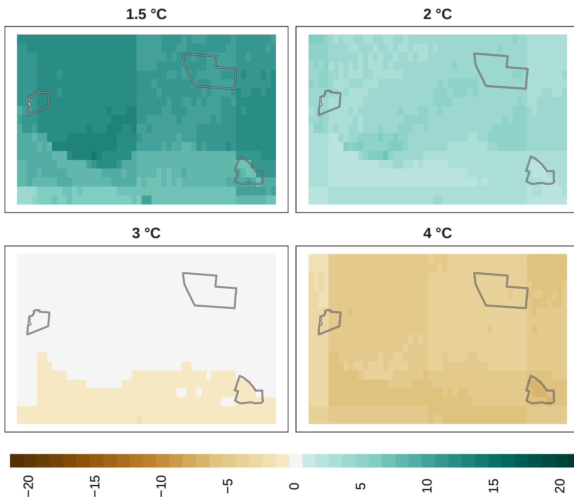
Figure 12: Adaptation effort for plants at 1 km resolution.
