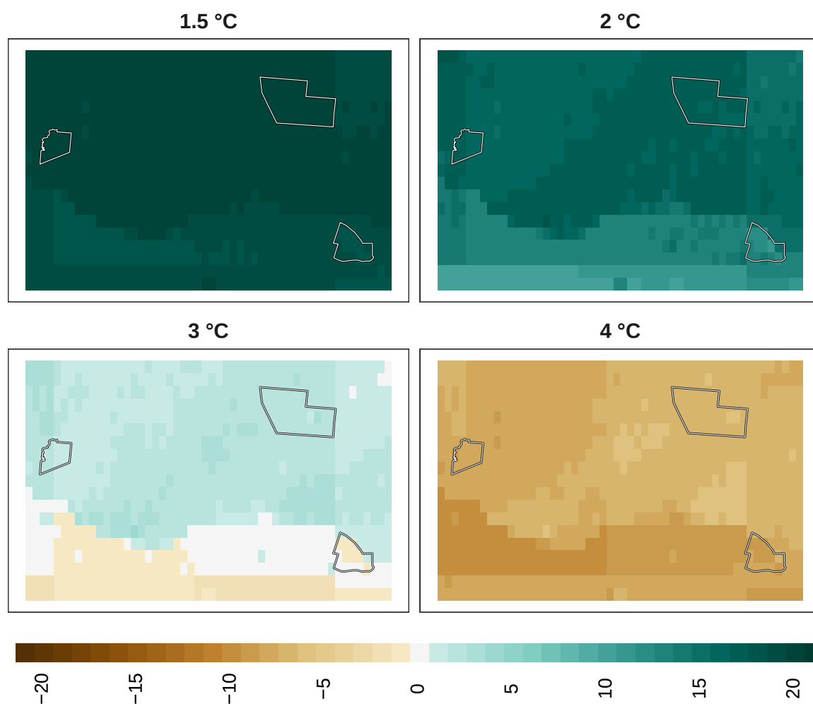
Figure 14: Adaptation effort for mammals at 1 km resolution.
