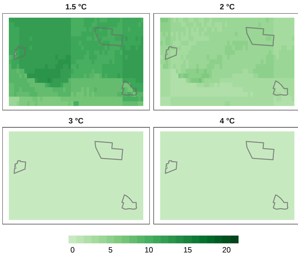
Figure 6: Number of models in agreement for overall biodiversity refugia at 1 km resolution.
