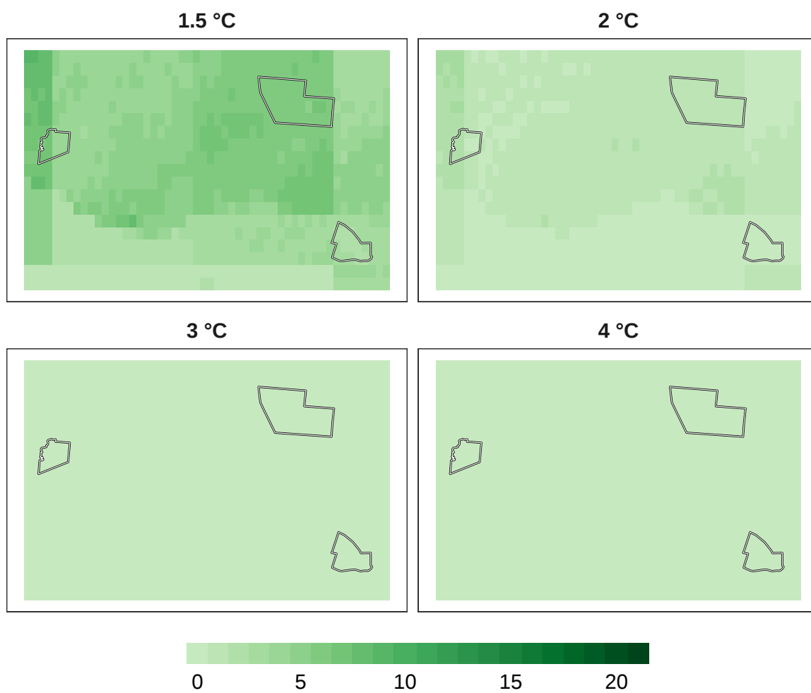
Figure 10: Number of models in agreement for insect refugia at 1 km resolution.
