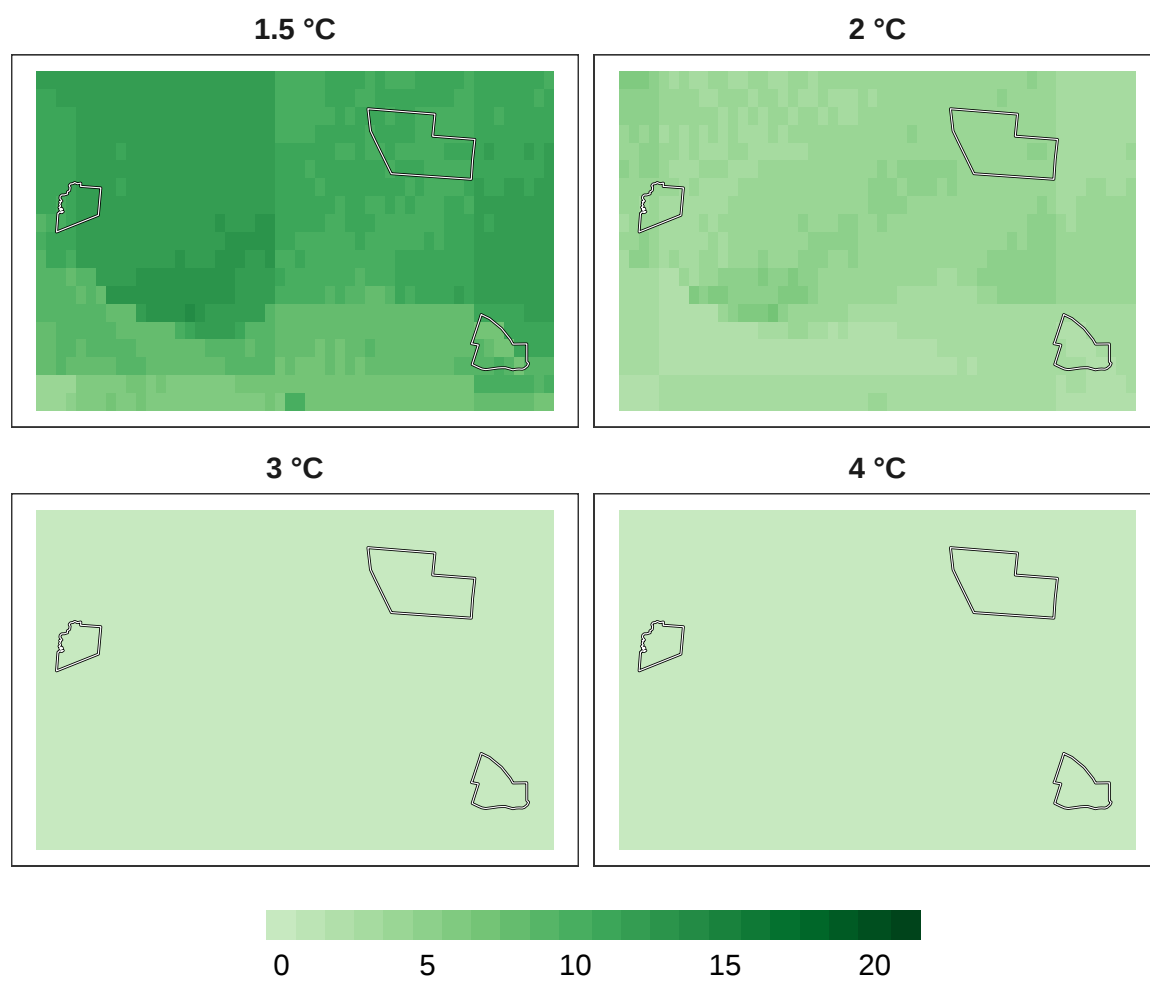
Figure 7: Number of models in agreement for plant refugia at 1 km resolution.
