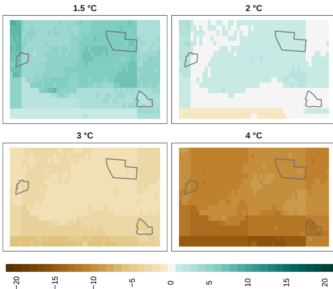
Figure 15: Adaptation effort for insects at 1 km resolution.
