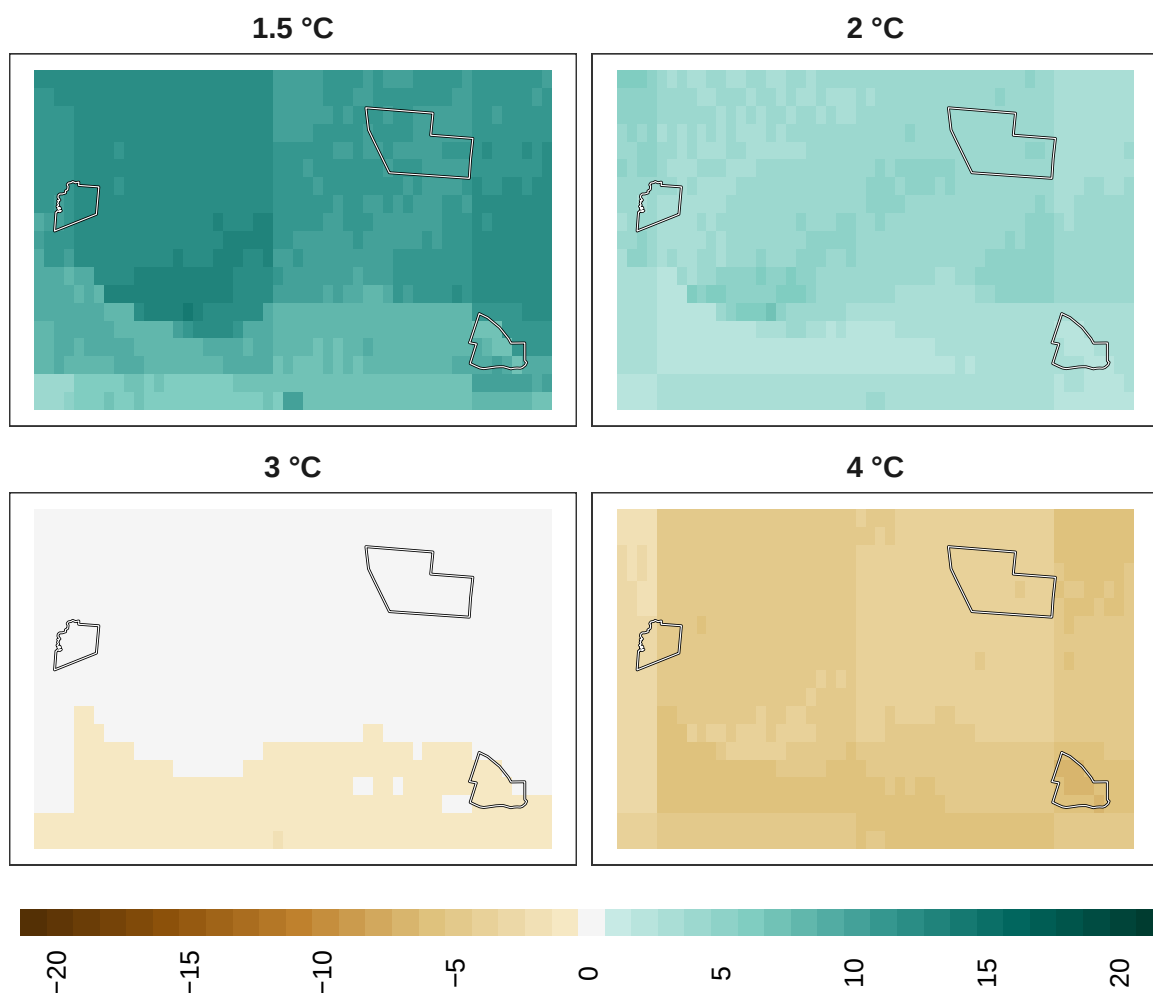
Figure 11: Adaptation effort for overall biodiversity at 1 km resolution.
