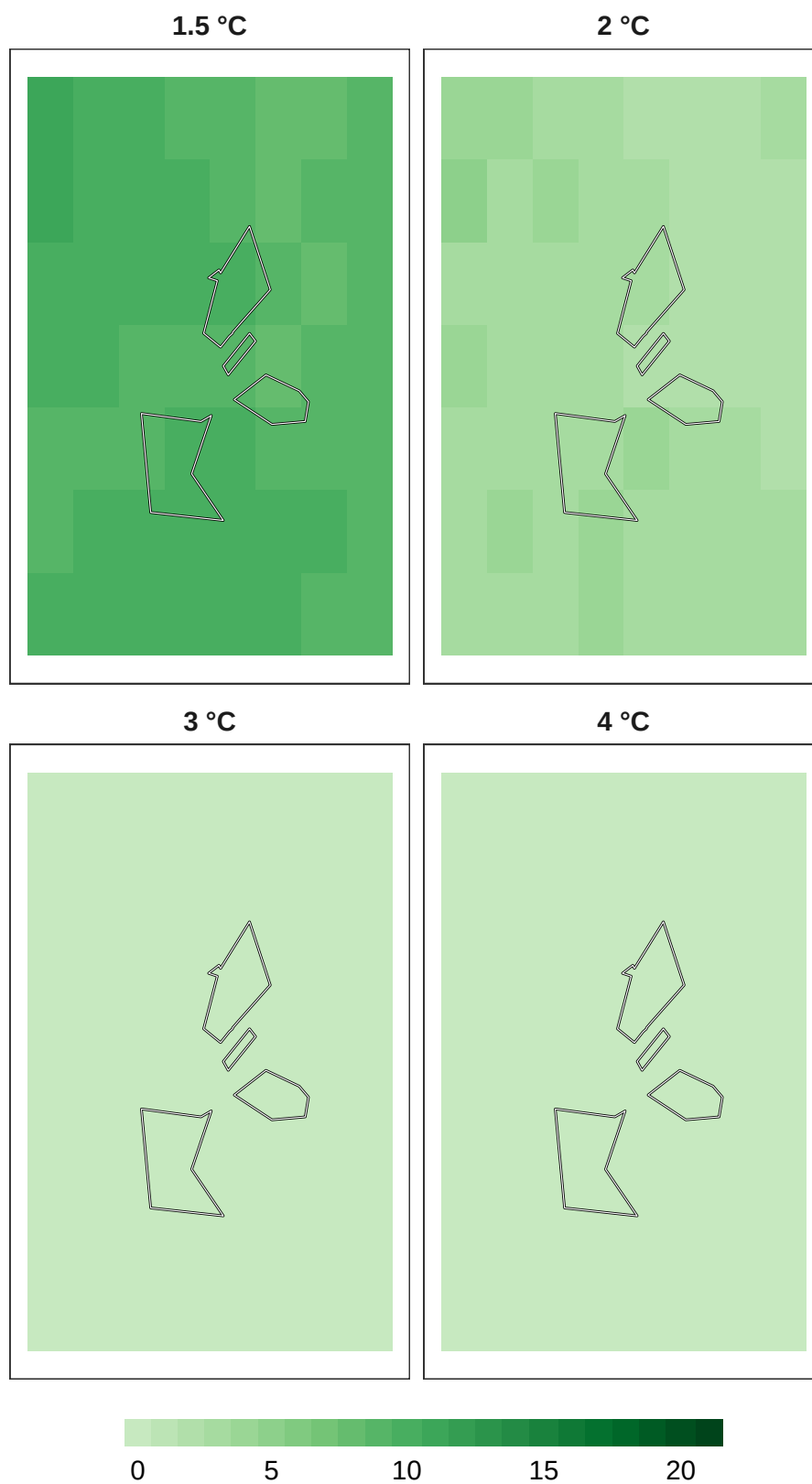
Figure 7: Number of models in agreement for plant refugia at 1 km resolution.
