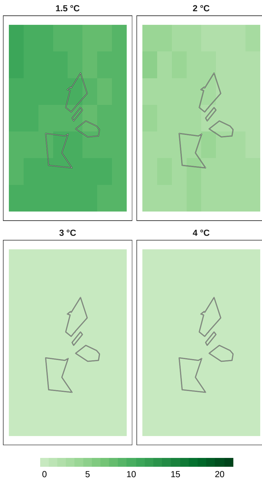
Figure 6: Number of models in agreement for overall biodiversity refugia at 1 km resolution.
