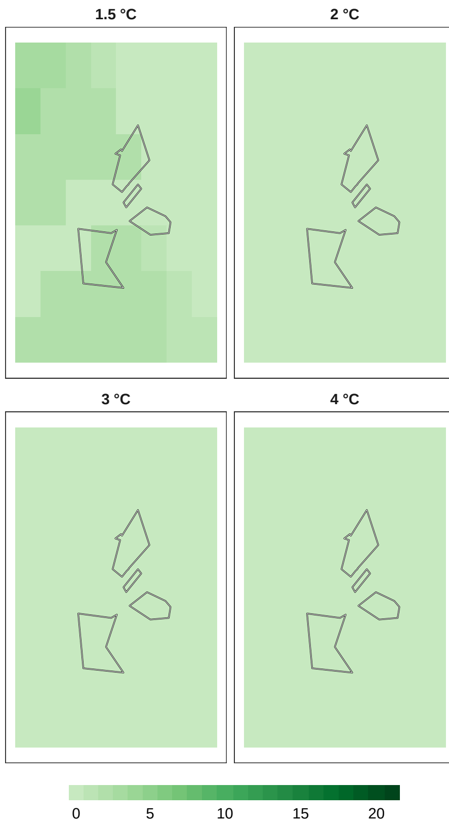
Figure 9: Number of models in agreement for mammal refugia at 1 km resolution.
