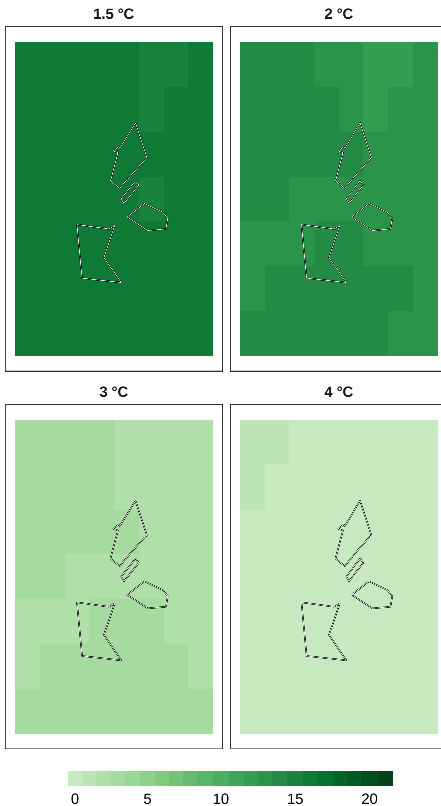
Figure 8: Number of models in agreement for bird refugia.
