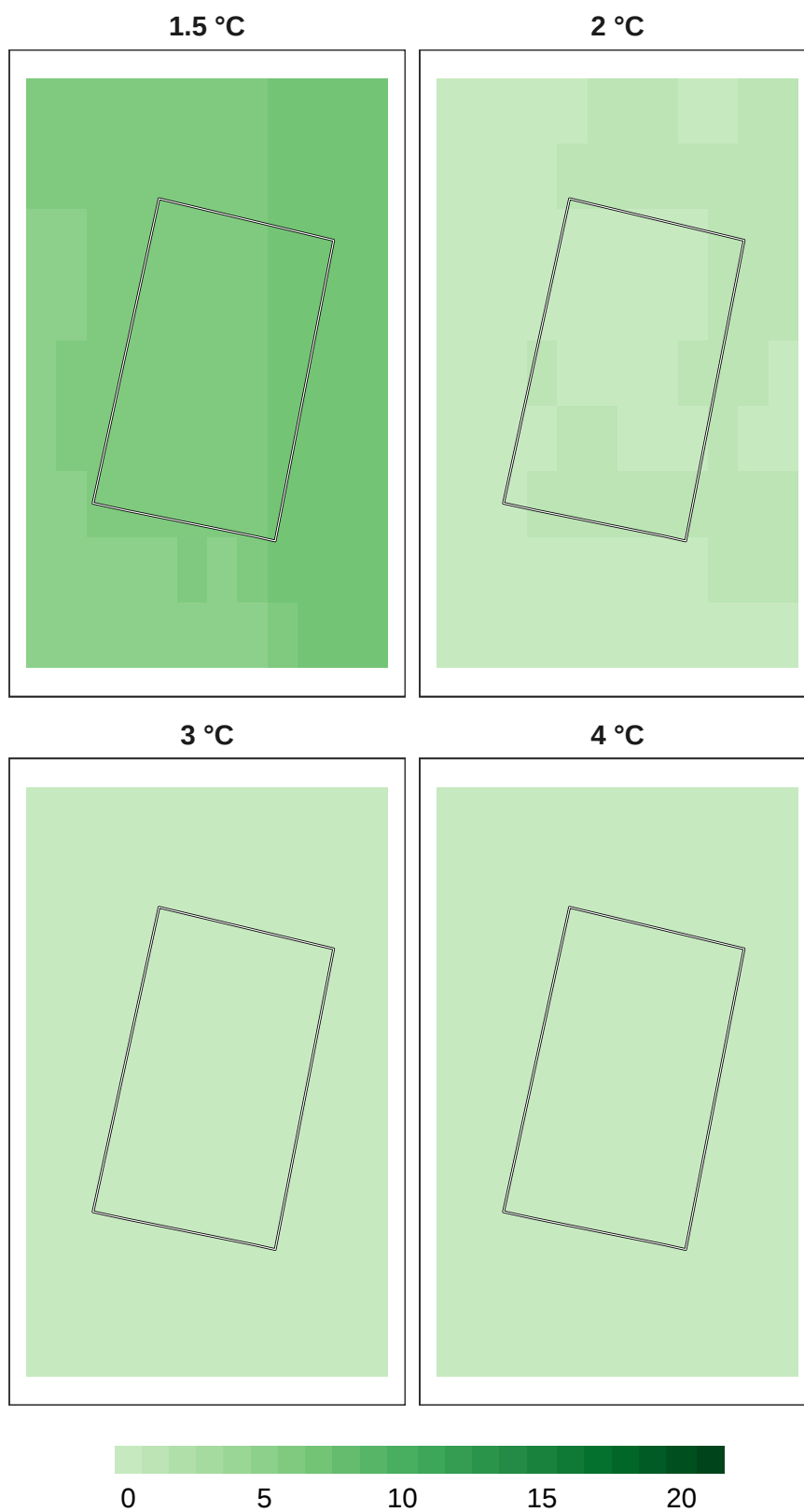
Figure 9: Number of models in agreement for insect refugia at 1 km resolution.
