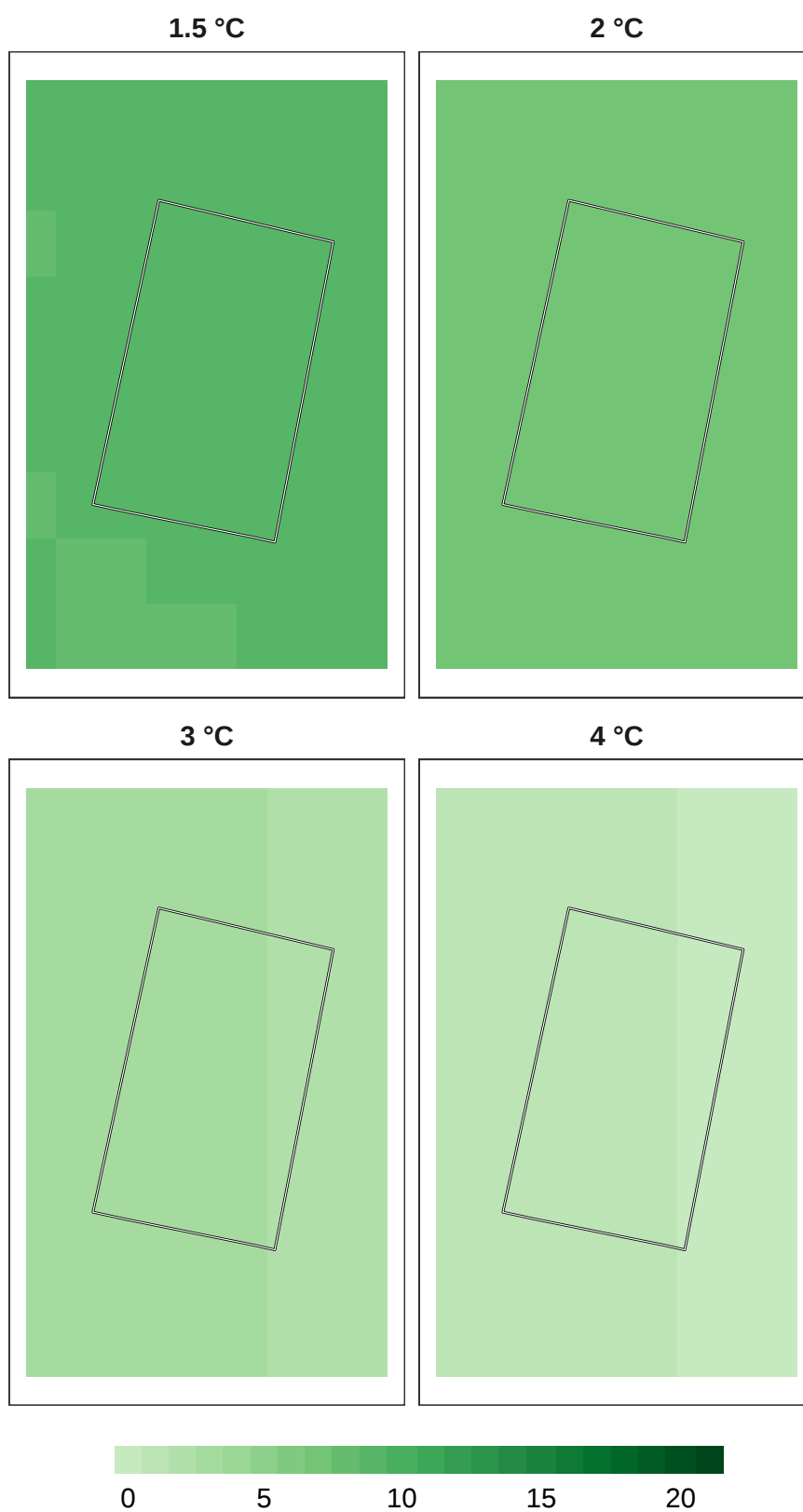
Figure 10: Number of models in agreement for pollinator refugia at 1 km resolution.
