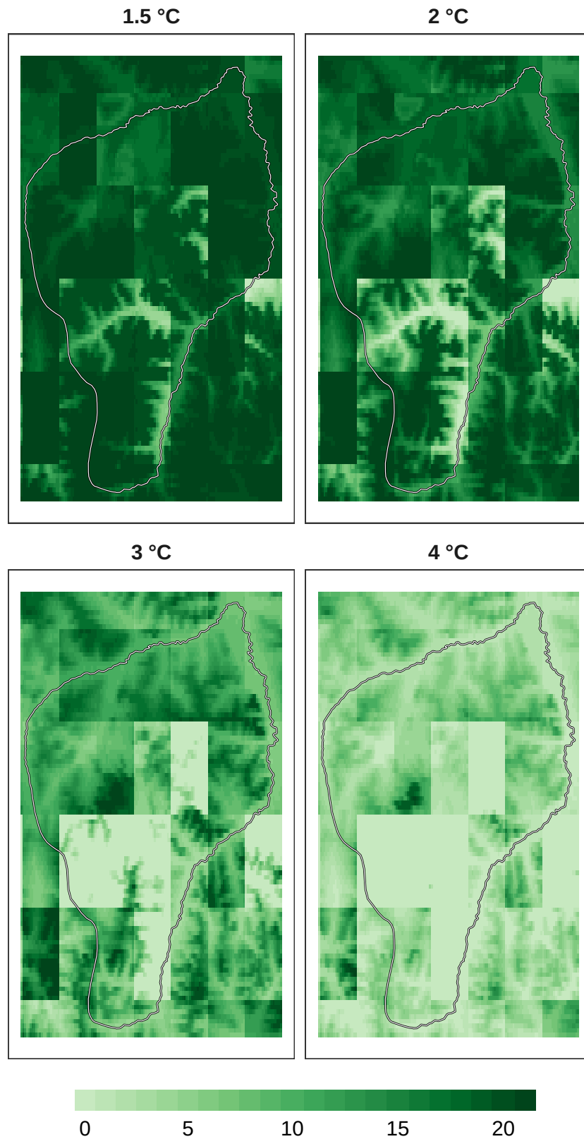
Figure 4: Number of models in agreement for overall biodiversity refugia at 1 km resolution.
