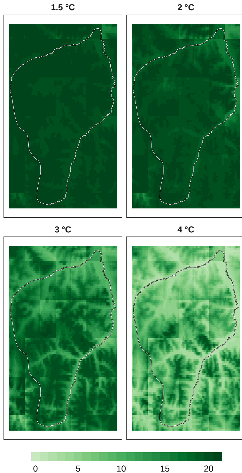
Figure 5: Number of models in agreement for plant refugia at 1 km resolution.
