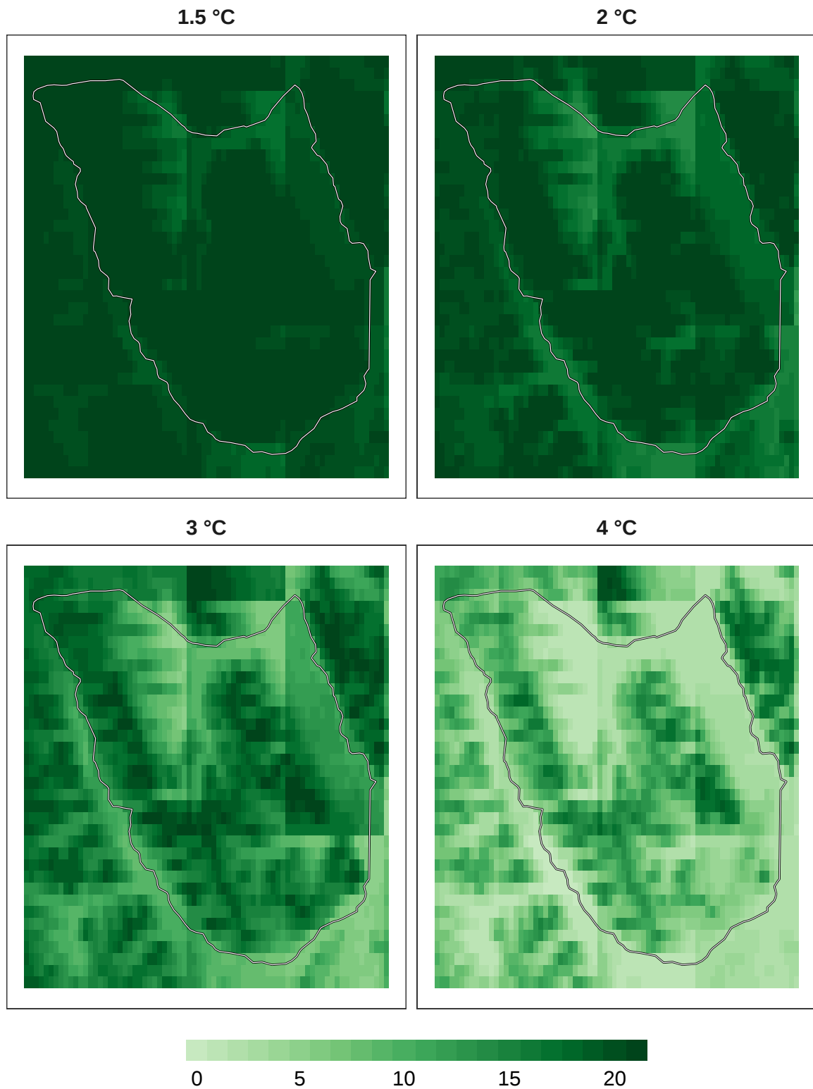
Figure 5: Number of models in agreement for plant refugia at 1 km resolution.
