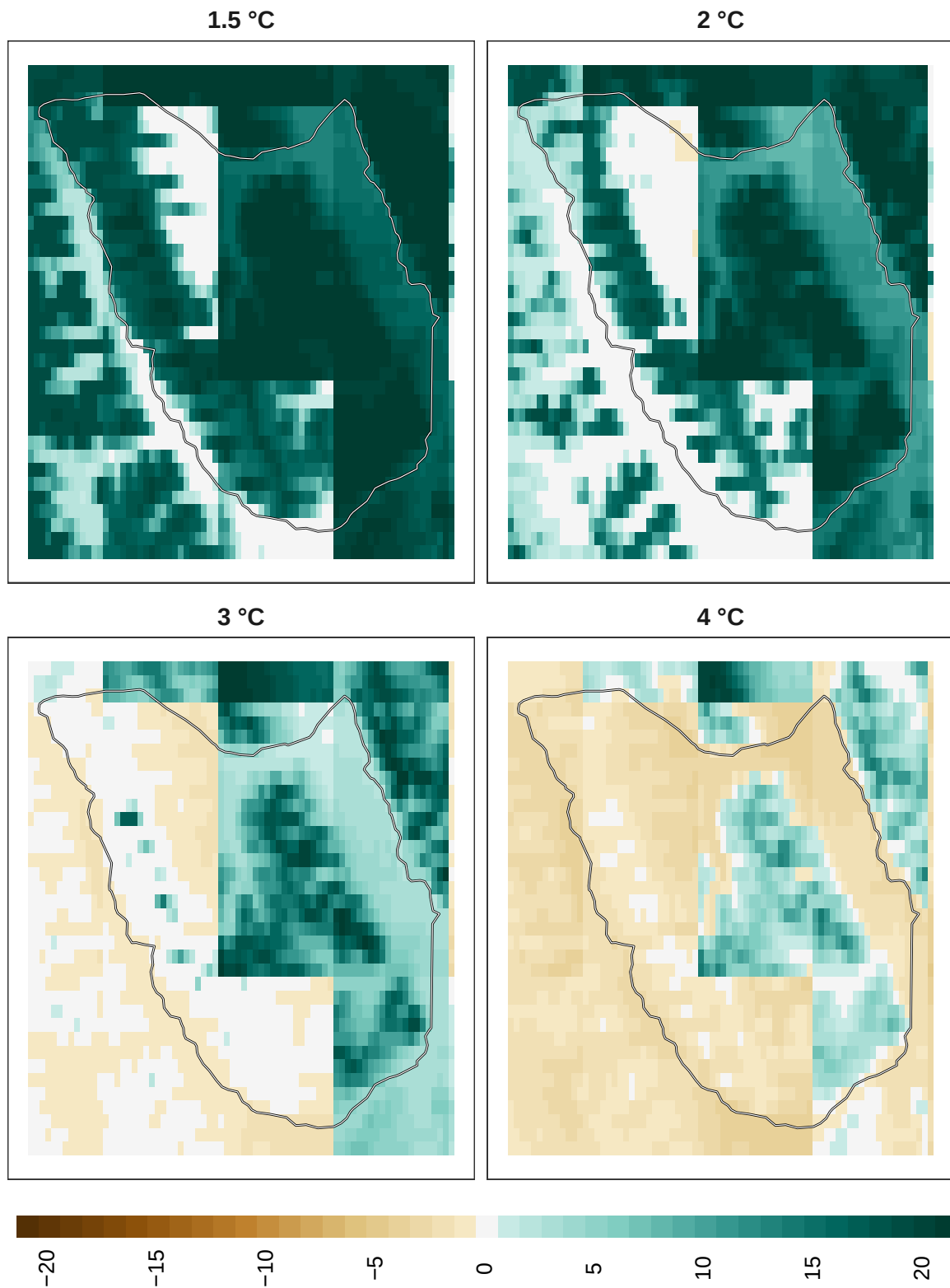
Figure 7: Adaptation effort for overall biodiversity at 1 km resolution.
