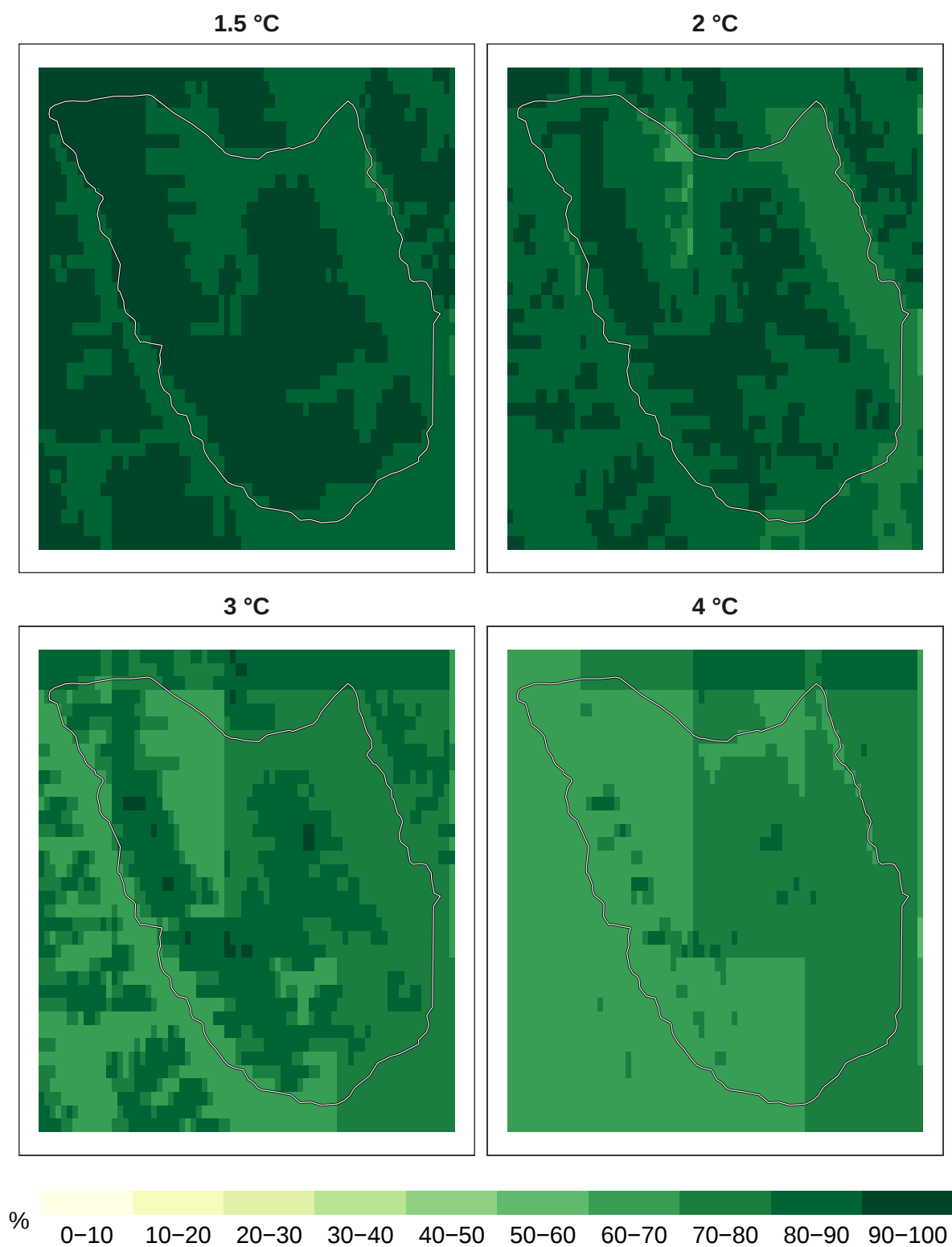
Figure 3: Percent mammals remaining at 1 km resolution.
