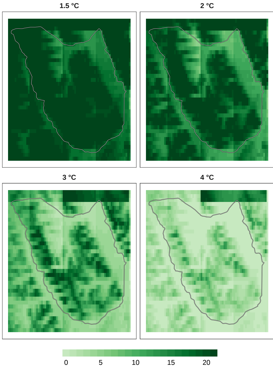
Figure 6: Number of models in agreement for mammal refugia at 1 km resolution.
