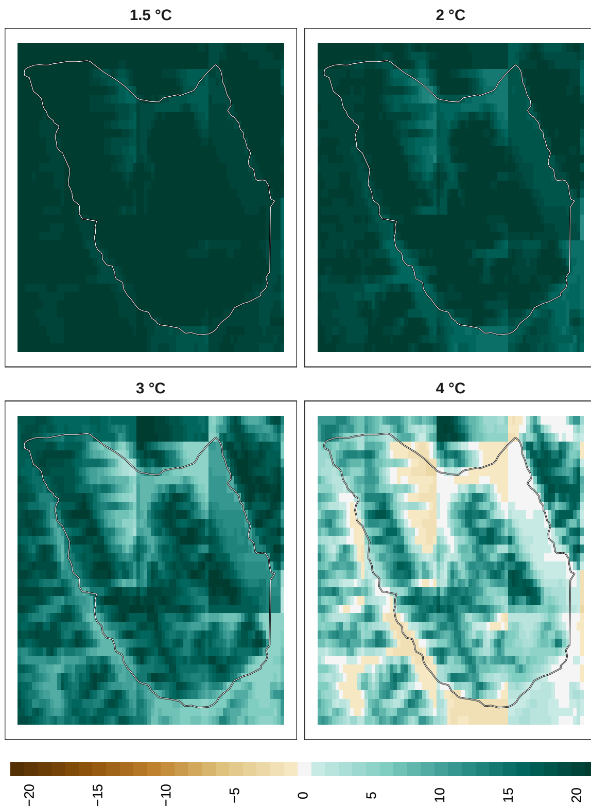
Figure 8: Adaptation effort for plants at 1 km resolution.
