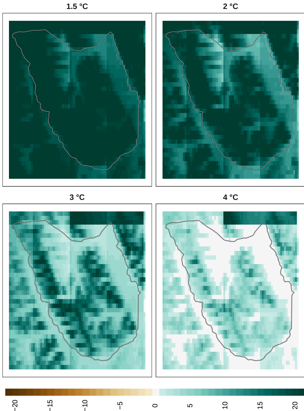
Figure 9: Adaptation effort for mammals at 1 km resolution.
