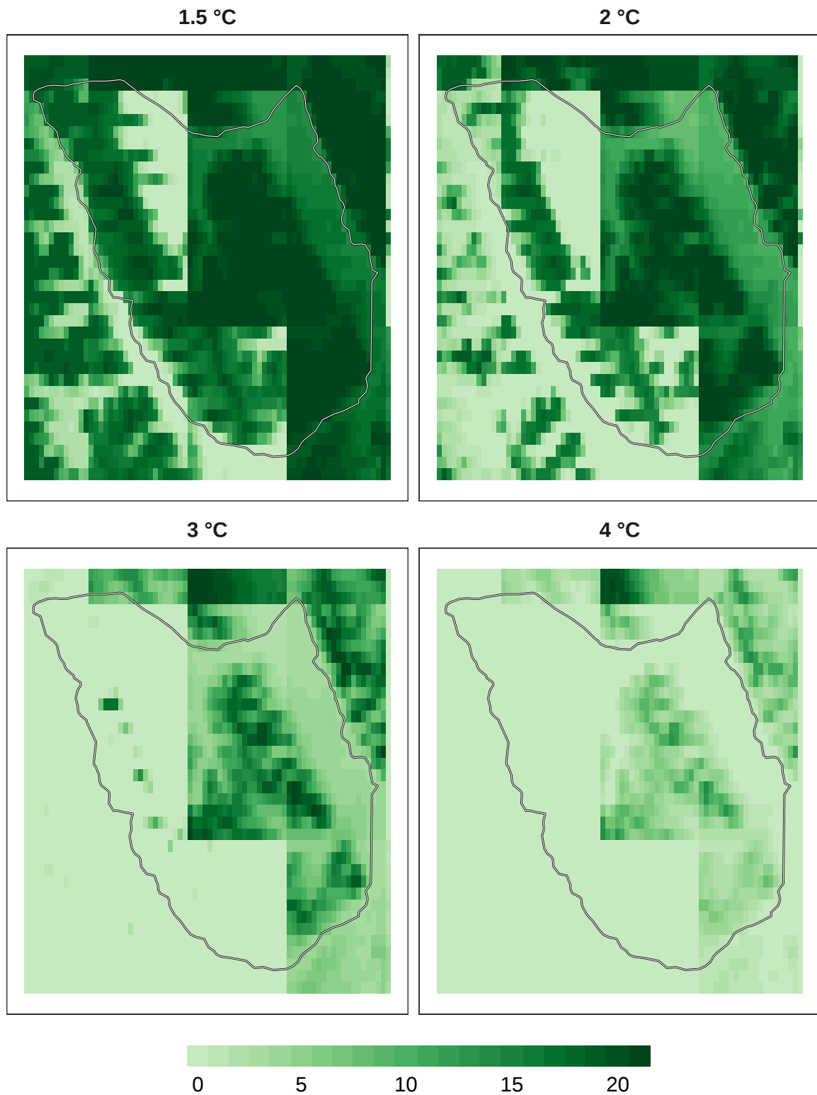
Figure 4: Number of models in agreement for overall biodiversity refugia at 1 km resolution.
