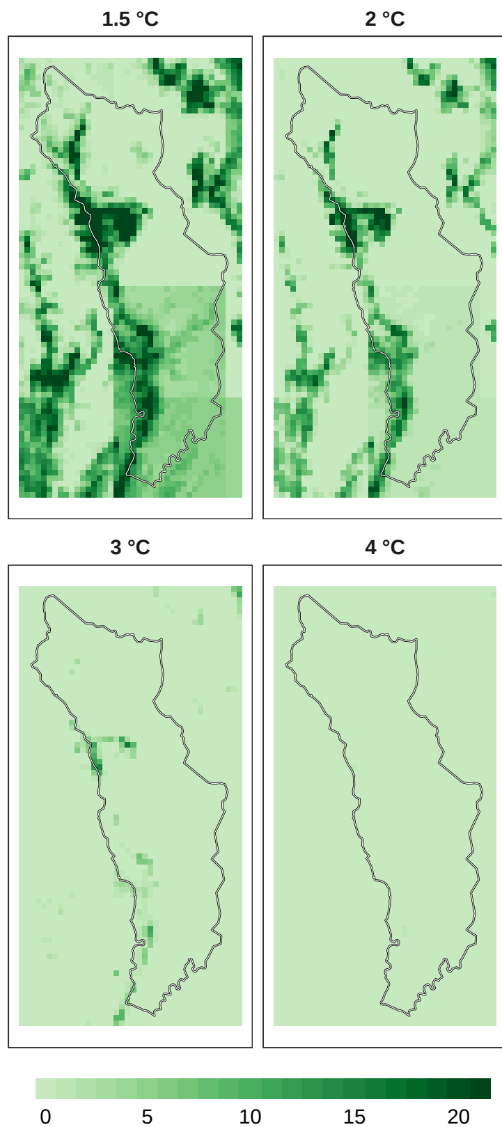
Figure 15: Number of models in agreement for reptile refugia at 1 km resolution.
