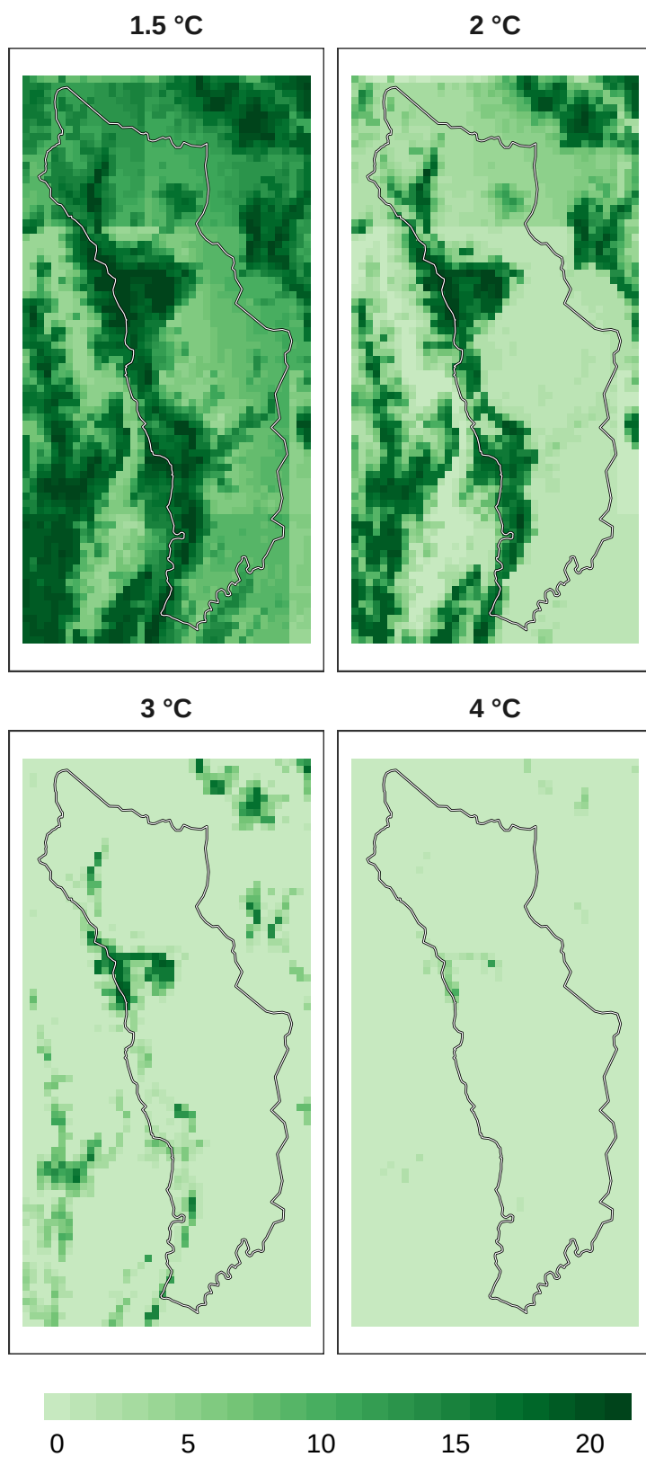
Figure 13: Number of models in agreement for bird refugia.
