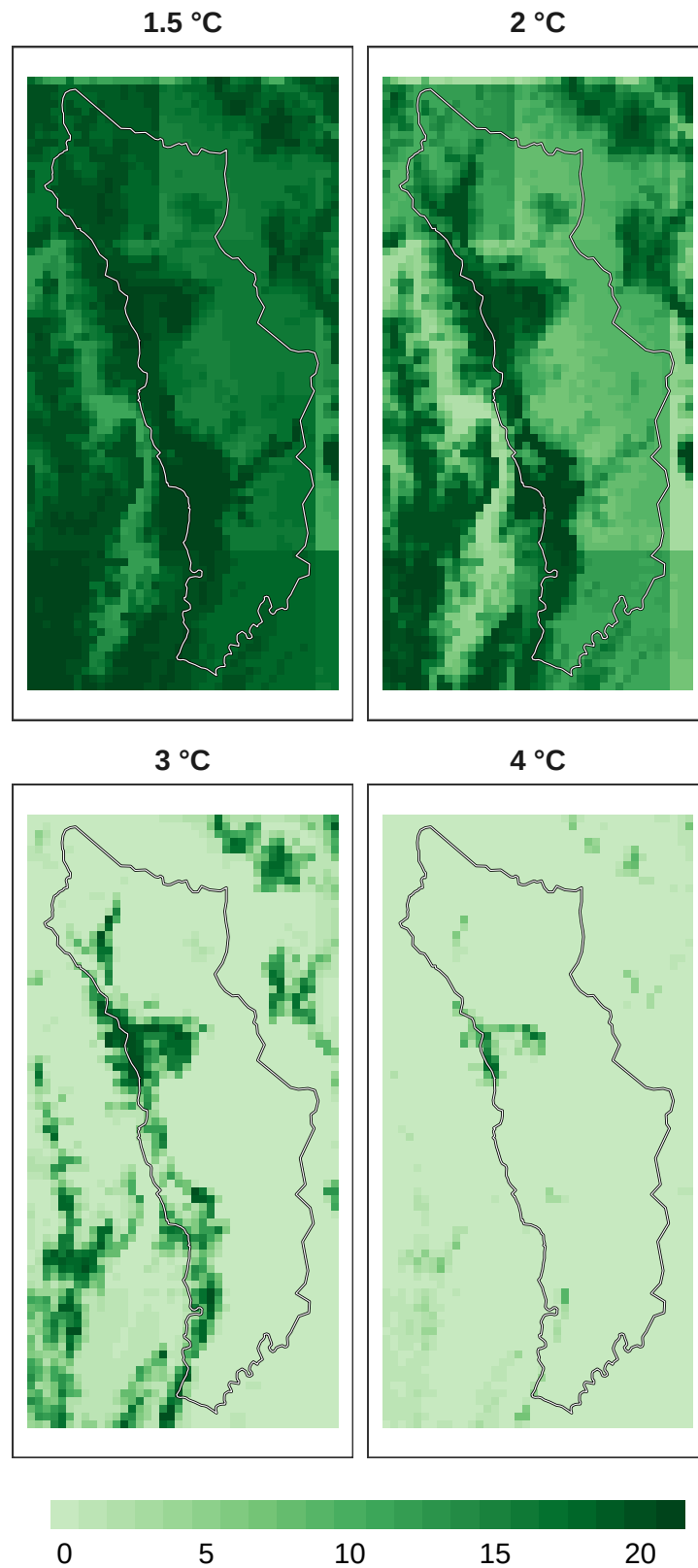
Figure 14: Number of models in agreement for mammal refugia at 1 km resolution.
