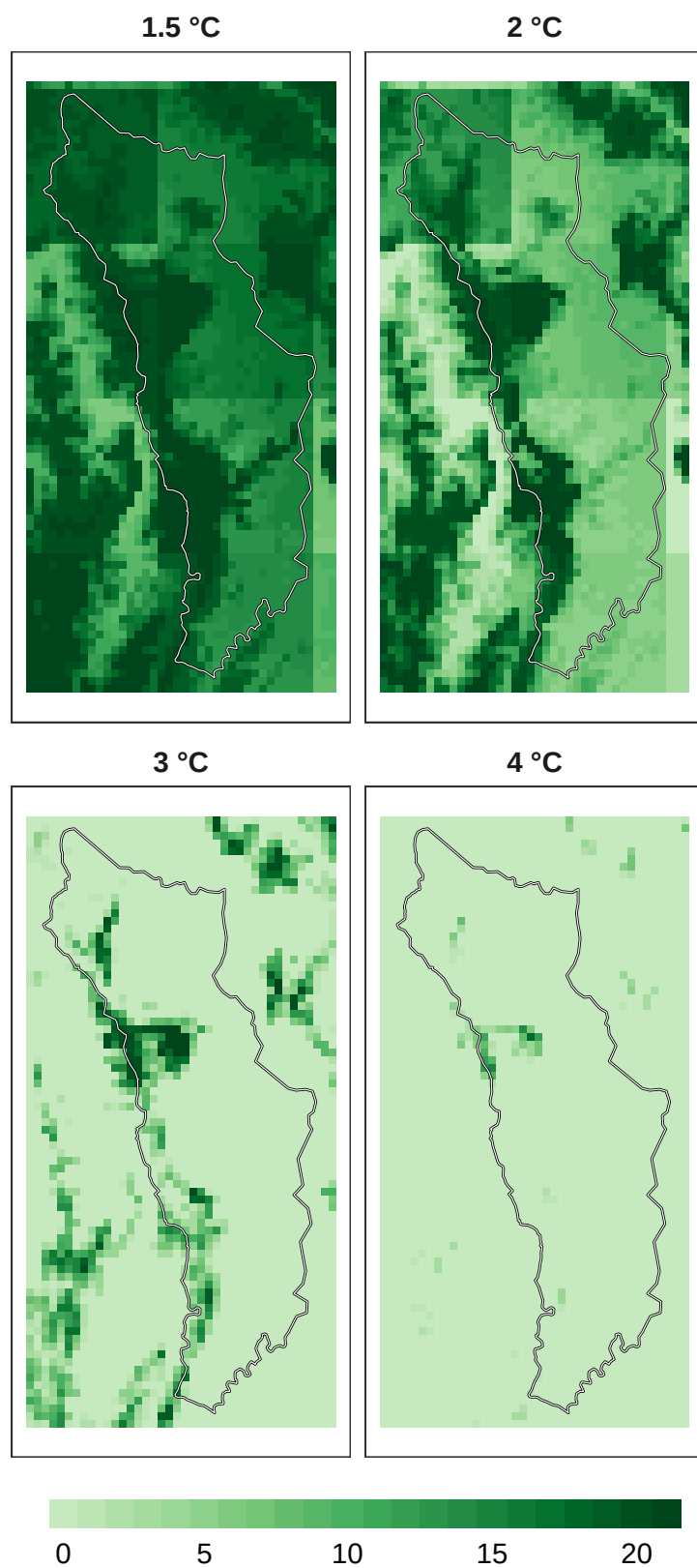
Figure 16: Number of models in agreement for insect refugia at 1 km resolution.
