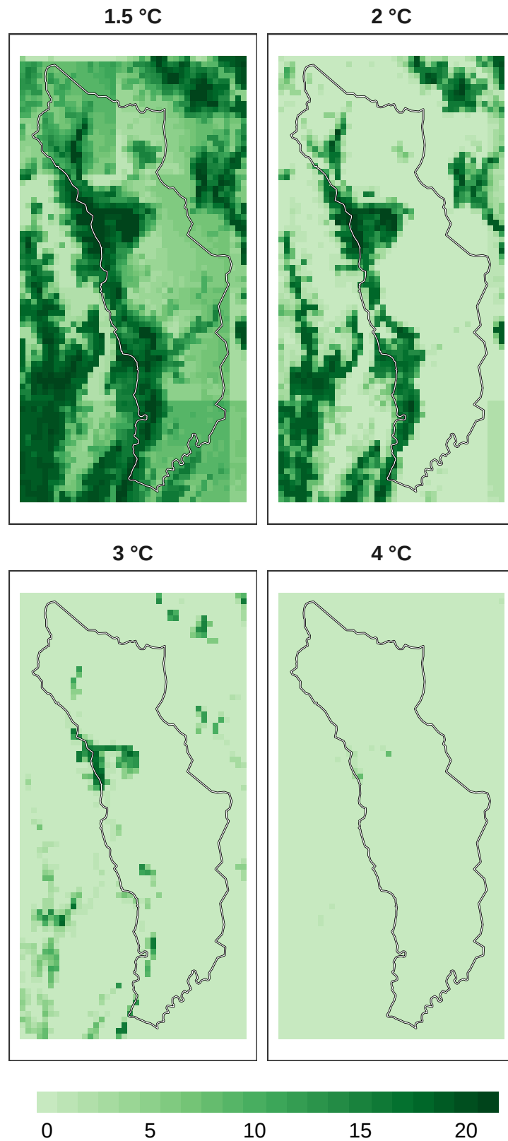
Figure 10: Number of models in agreement for overall biodiversity refugia at 1 km resolution.
