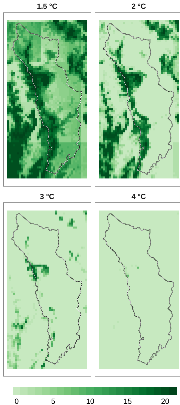
Figure 11: Number of models in agreement for plant refugia at 1 km resolution.
