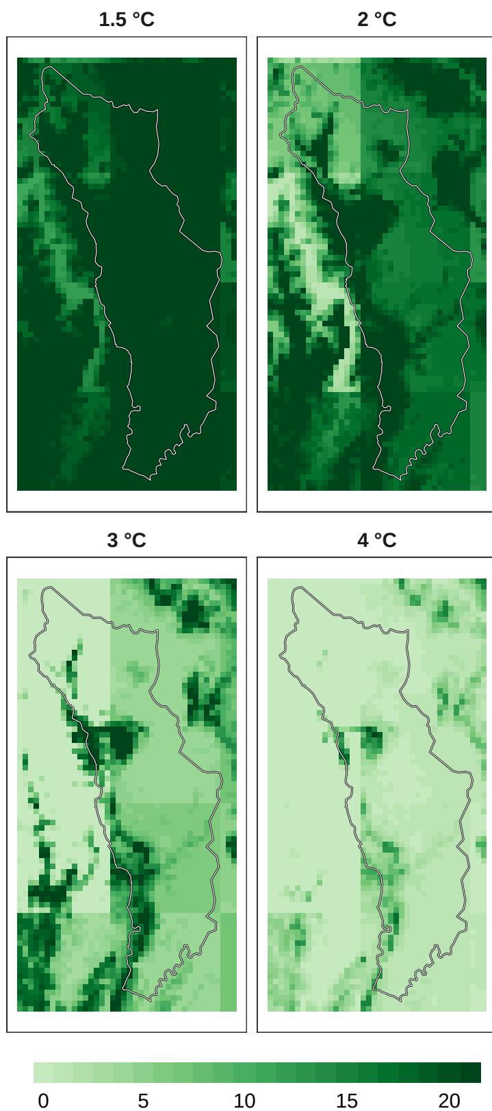
Figure 17: Number of models in agreement for pollinator refugia at 1 km resolution.
