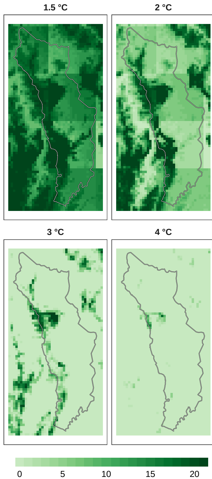
Figure 12: Number of models in agreement for amphibian refugia at 1 km resolution.
