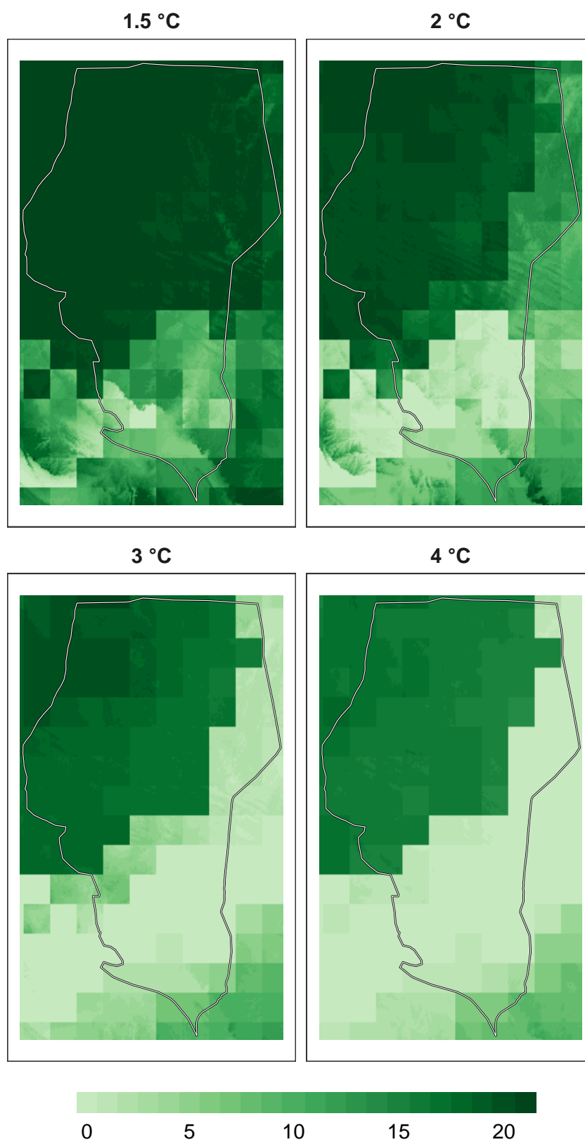
Figure 16: Number of models in agreement for pollinator refugia at 1 km resolution.
