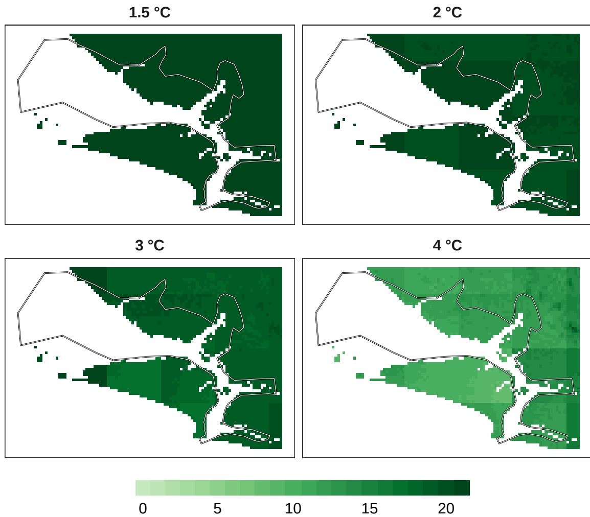
Figure 15: Number of models in agreement for insect refugia at 1 km resolution.
