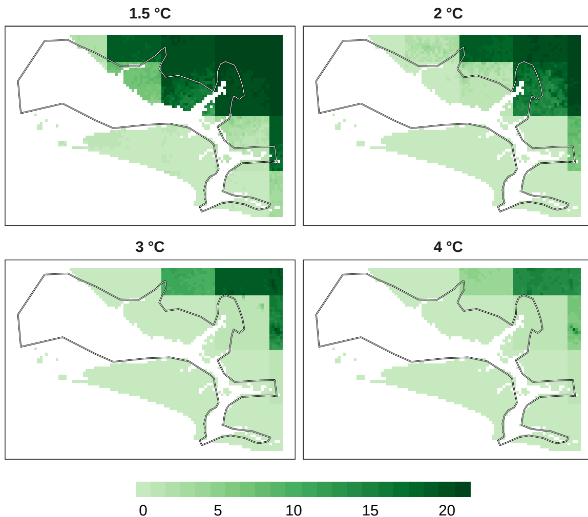
Figure 14: Number of models in agreement for reptile refugia at 1 km resolution.
