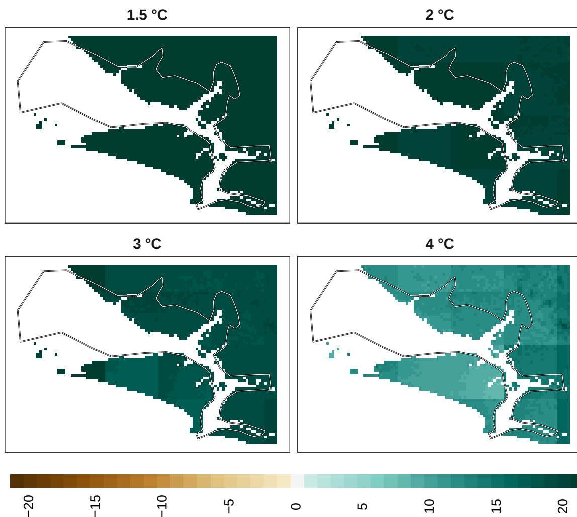
Figure 22: Adaptation effort for insects at 1 km resolution.
