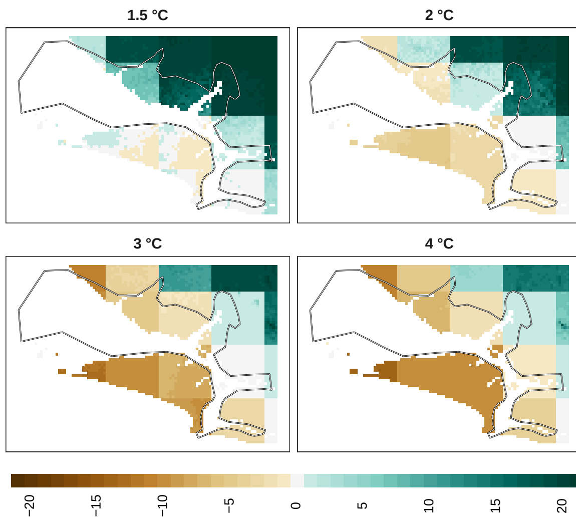
Figure 21: Adaptation effort for reptiles at 1 km resolution.
