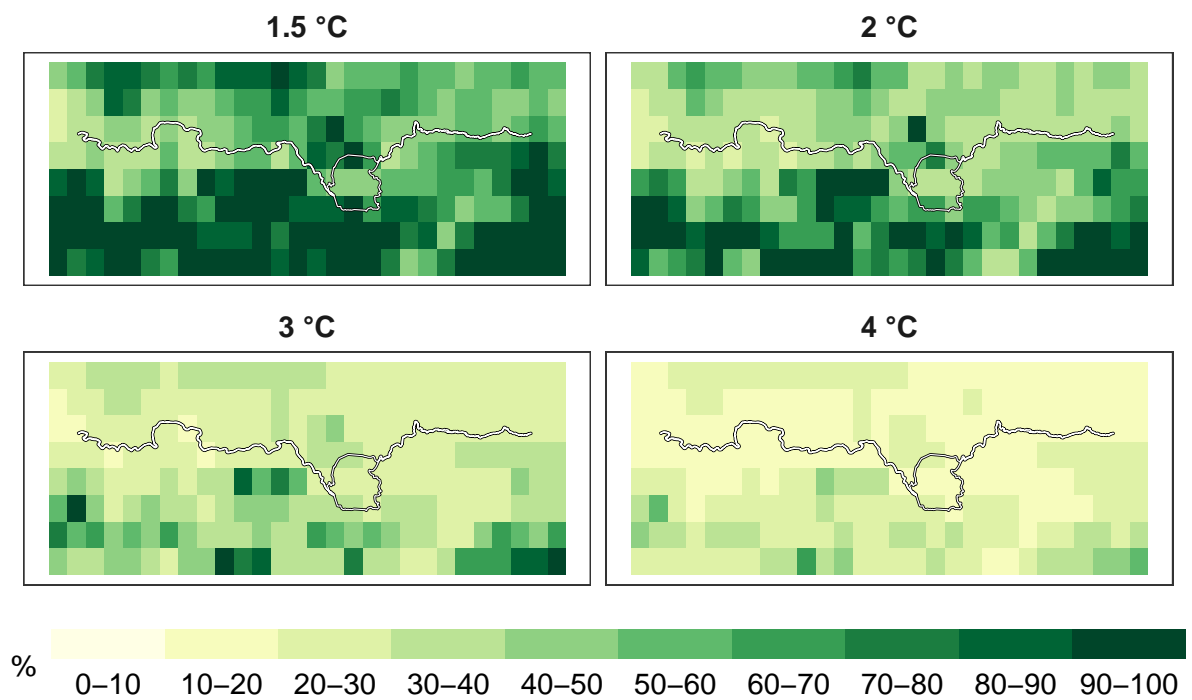
Figure 7: Percent insects remaining at 1 km resolution.
