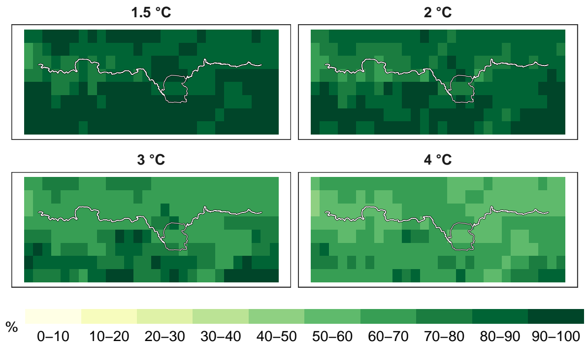
Figure 6: Percent reptiles remaining at 1 km resolution.
