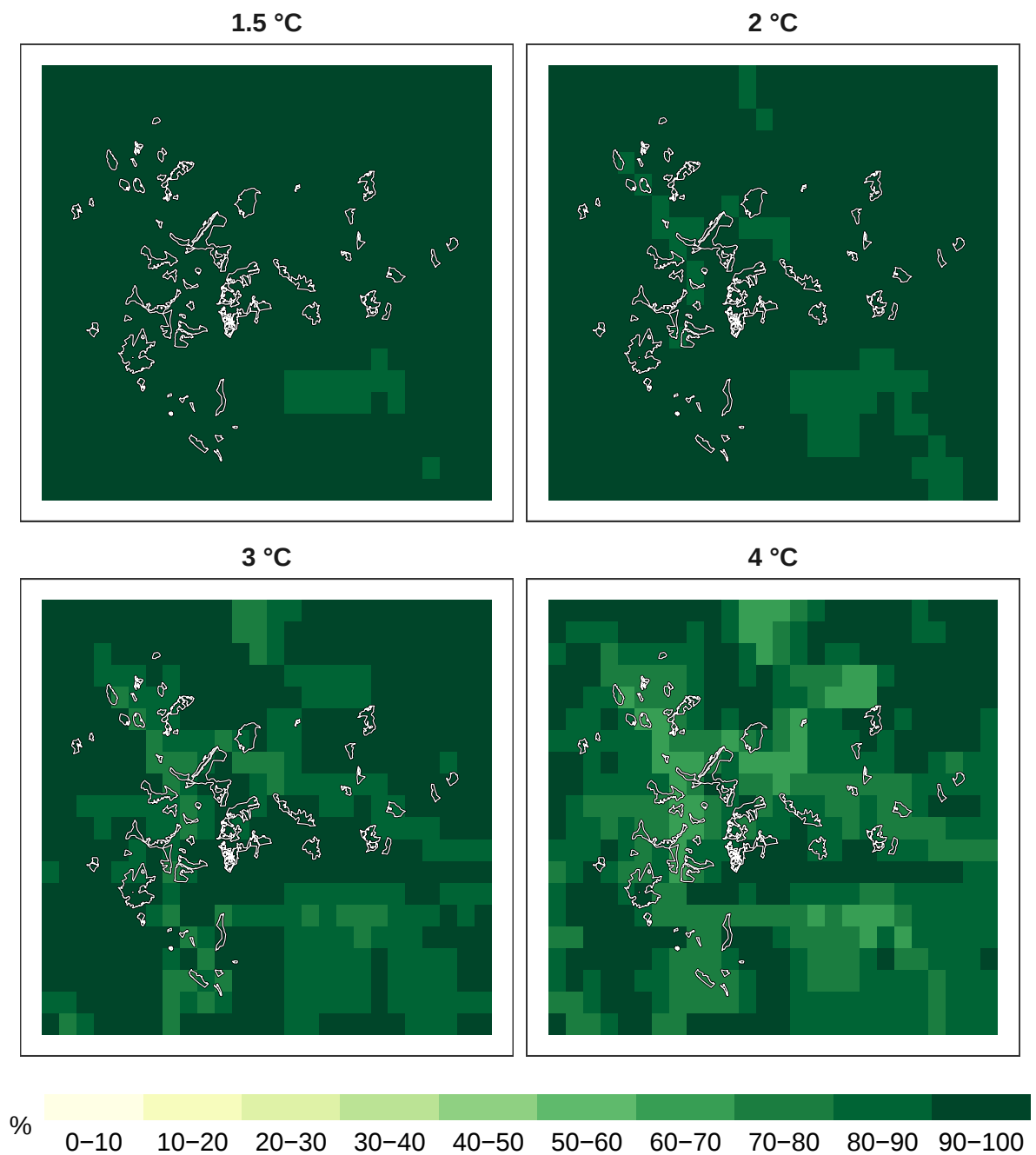
Figure 3: Percent amphibians remaining at 1 km resolution.
