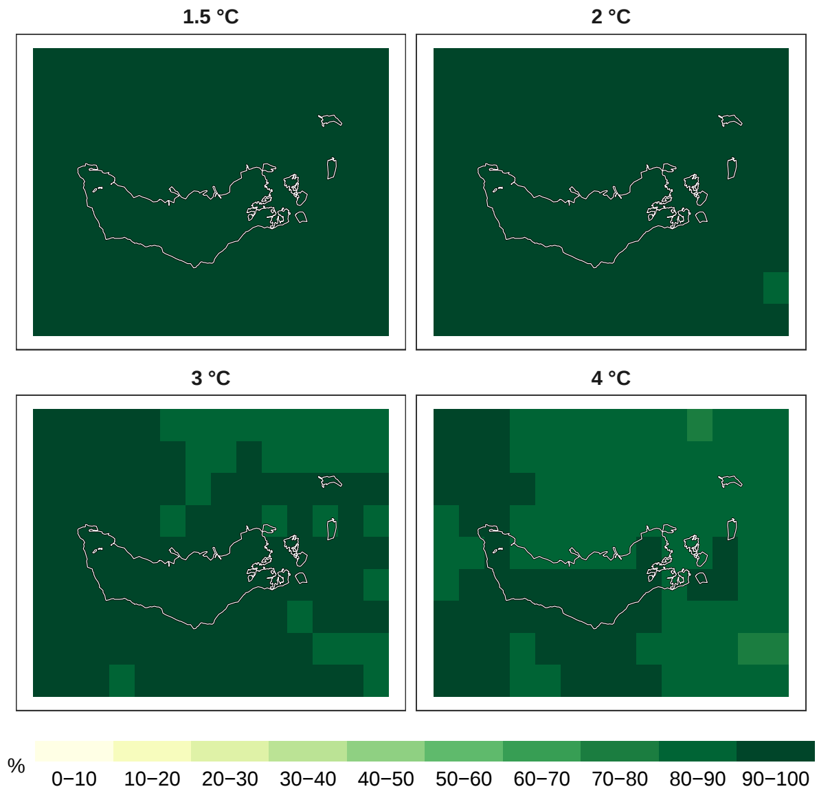
Figure 7: Percent insects remaining at 1 km resolution.
