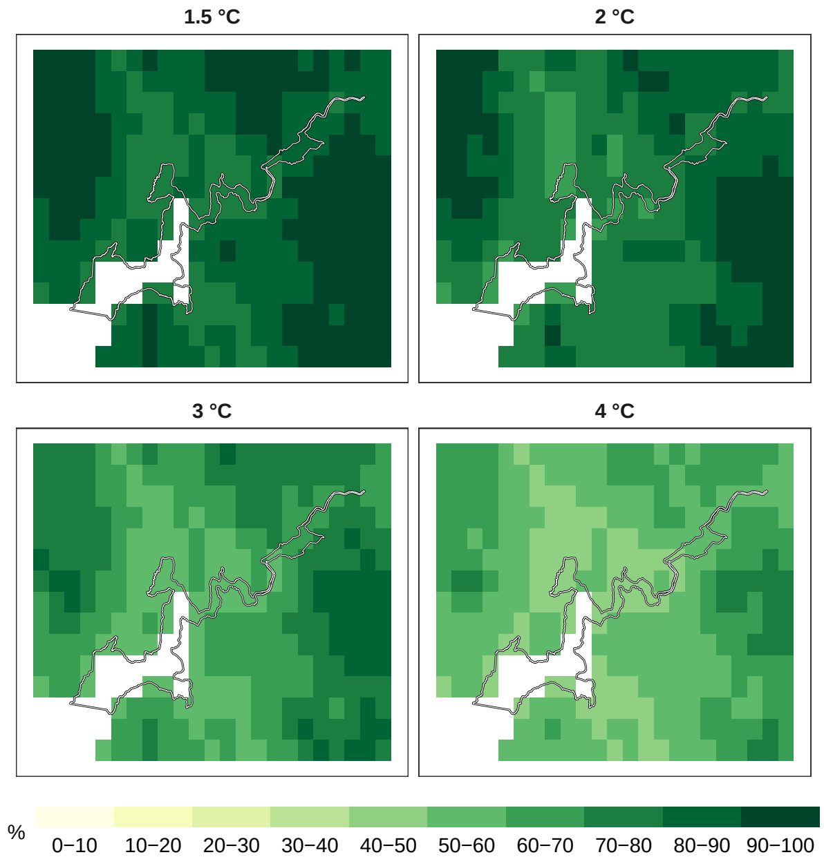
Figure 5: Percent mammals remaining at 1 km resolution.
