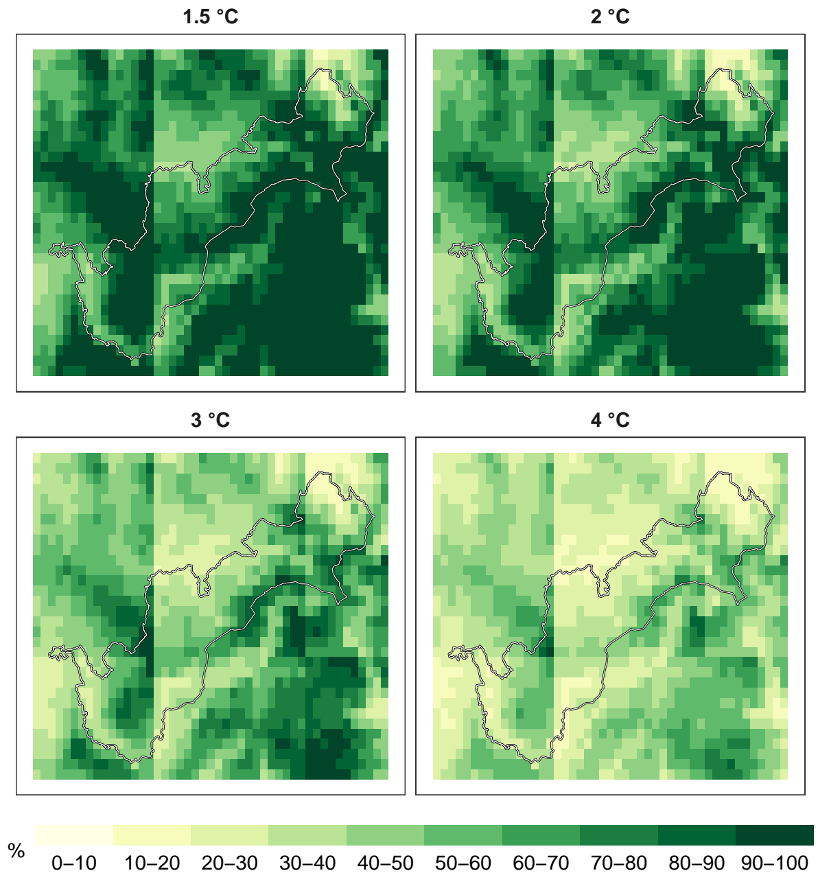
Figure 1: Percent overall biodiversity remaining at 1 km resolution.
