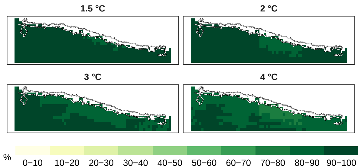
Figure 6: Percent reptiles remaining at 1 km resolution.
