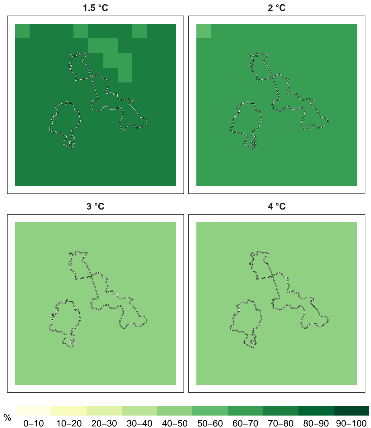
Figure 3: Percent birds remaining at 1 km resolution.
