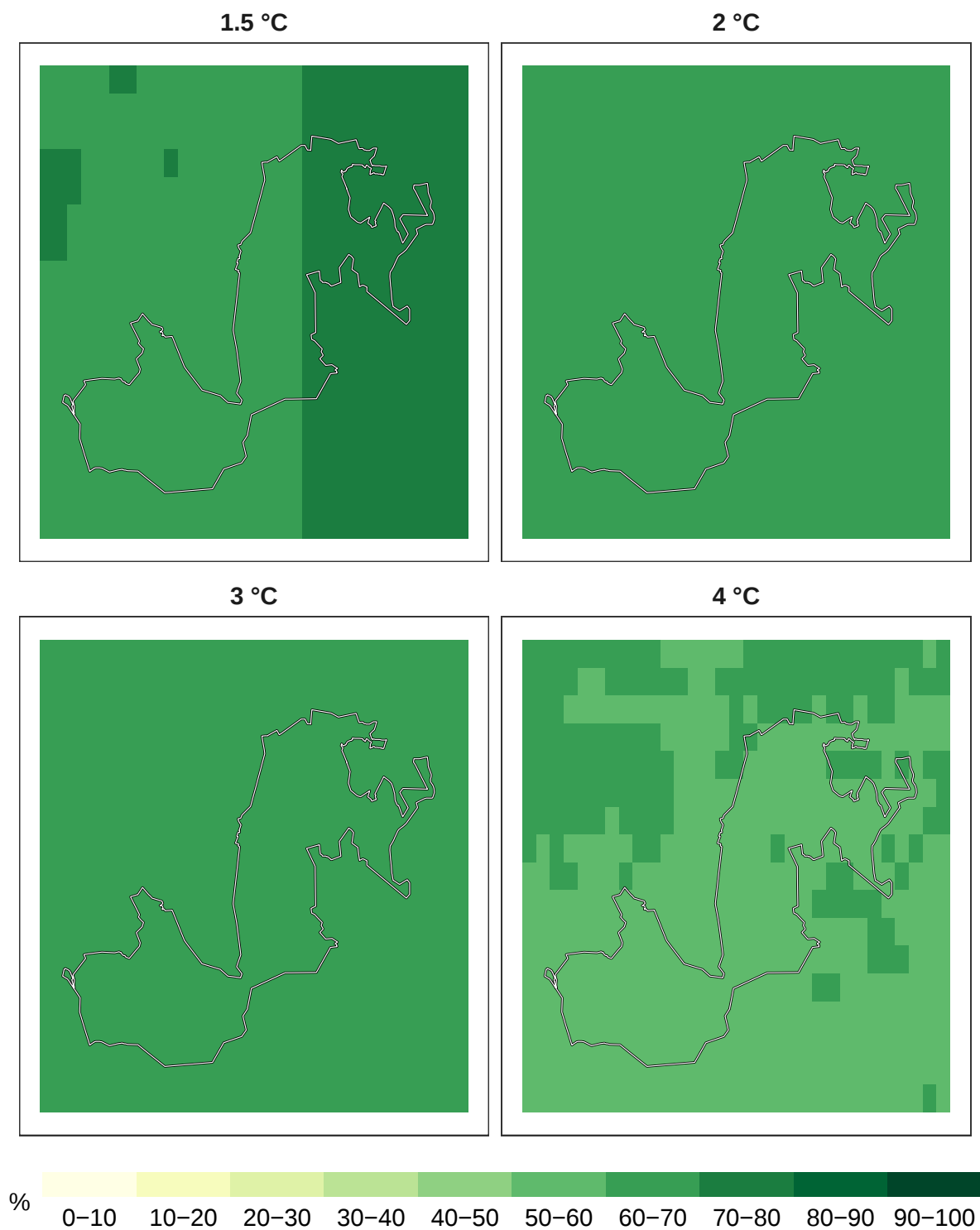
Figure 6: Percent reptiles remaining at 1 km resolution.
