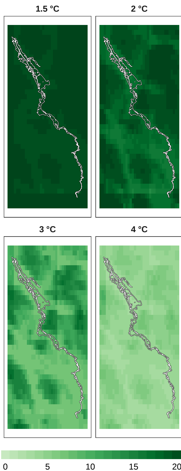
Figure 10: Number of models in agreement for plant refugia at 1 km resolution.
