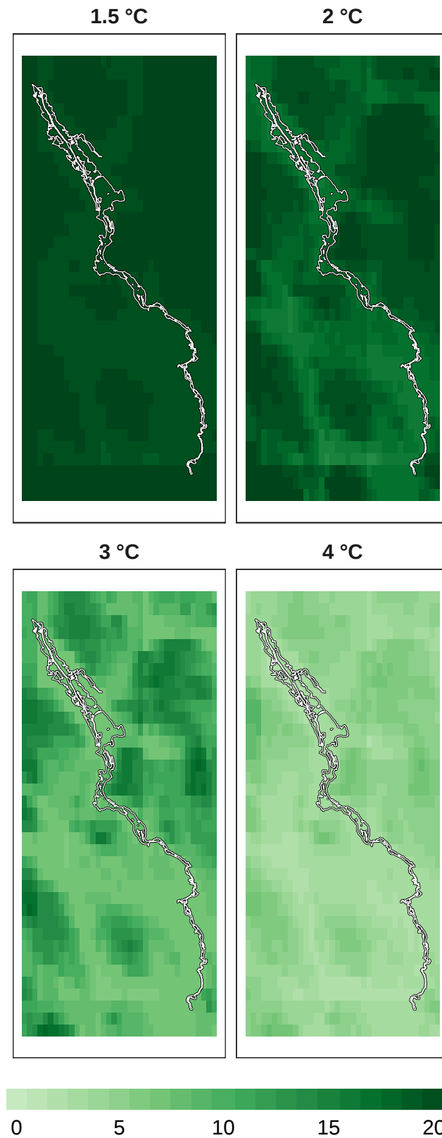
Figure 9: Number of models in agreement for overall biodiversity refugia at 1 km resolution.
