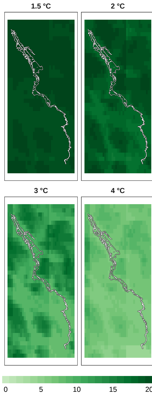
Figure 13: Number of models in agreement for reptile refugia at 1 km resolution.
