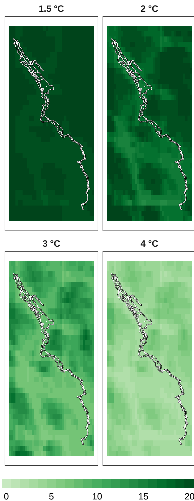
Figure 14: Number of models in agreement for insect refugia at 1 km resolution.
