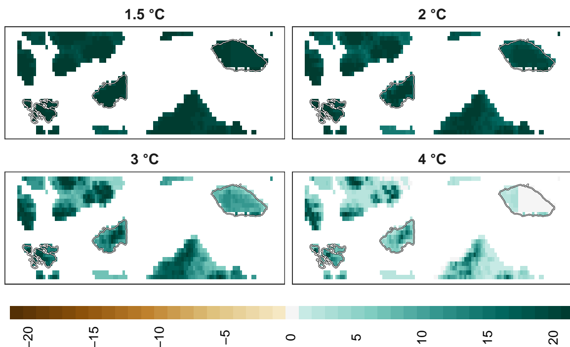
Figure 20: Adaptation effort for mammals at 1 km resolution.
