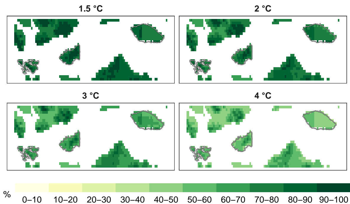
Figure 6: Percent insects remaining at 1 km resolution.
