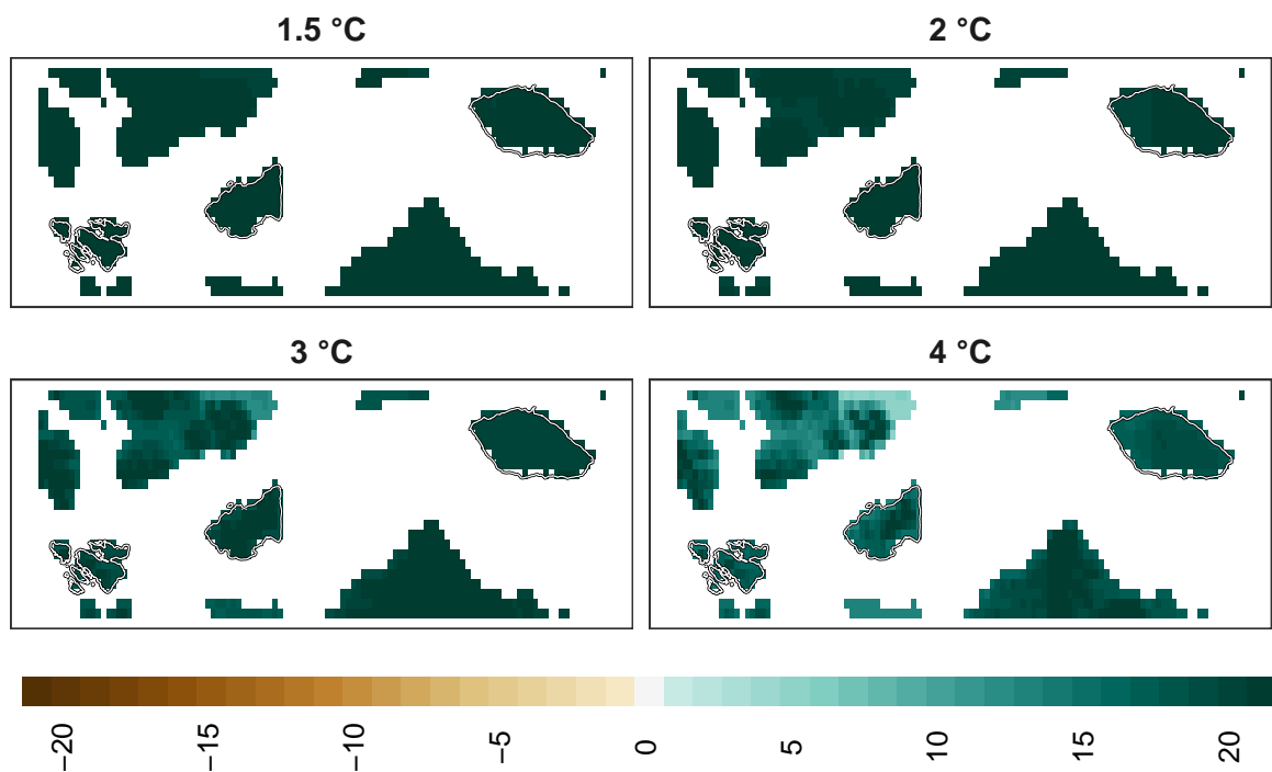
Figure 18: Adaptation effort for amphibians at 1 km resolution.
