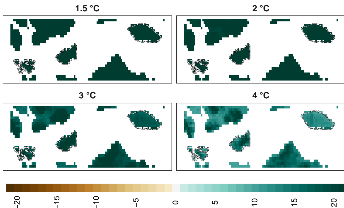
Figure 19: Adaptation effort for birds at 1 km resolution.
