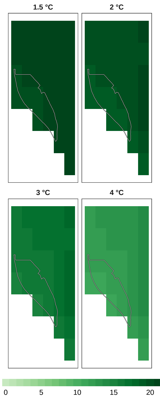
Figure 11: Number of models in agreement for amphibian refugia at 1 km resolution.
