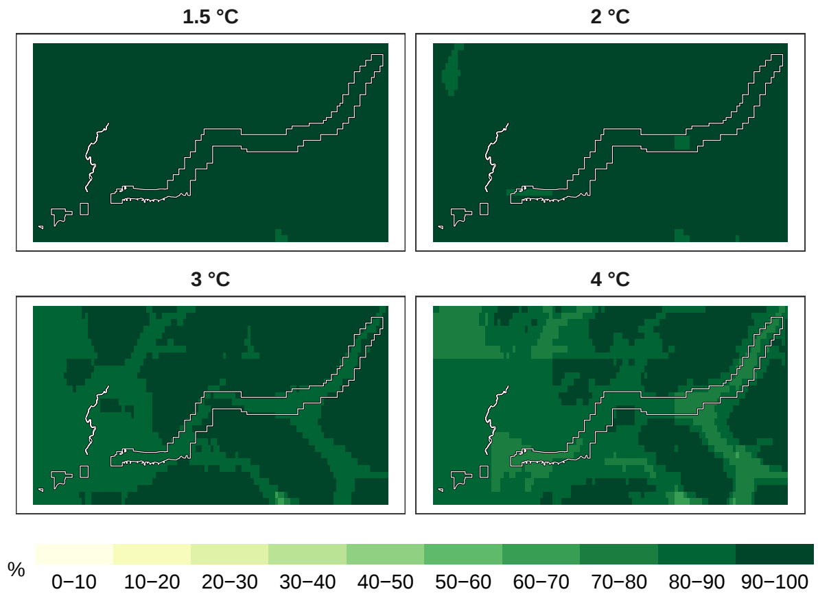
Figure 3: Percent birds remaining at 1 km resolution.
