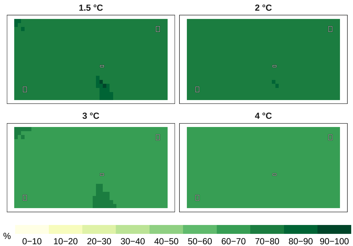
Figure 4: Percent birds remaining at 1 km resolution.
