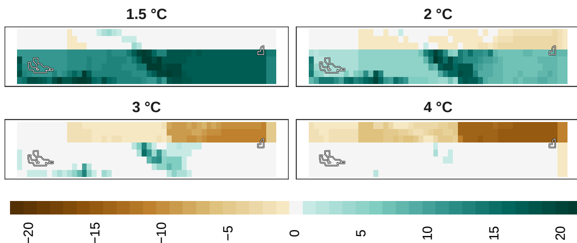
Figure 22: Adaptation effort for mammals at 1 km resolution.
