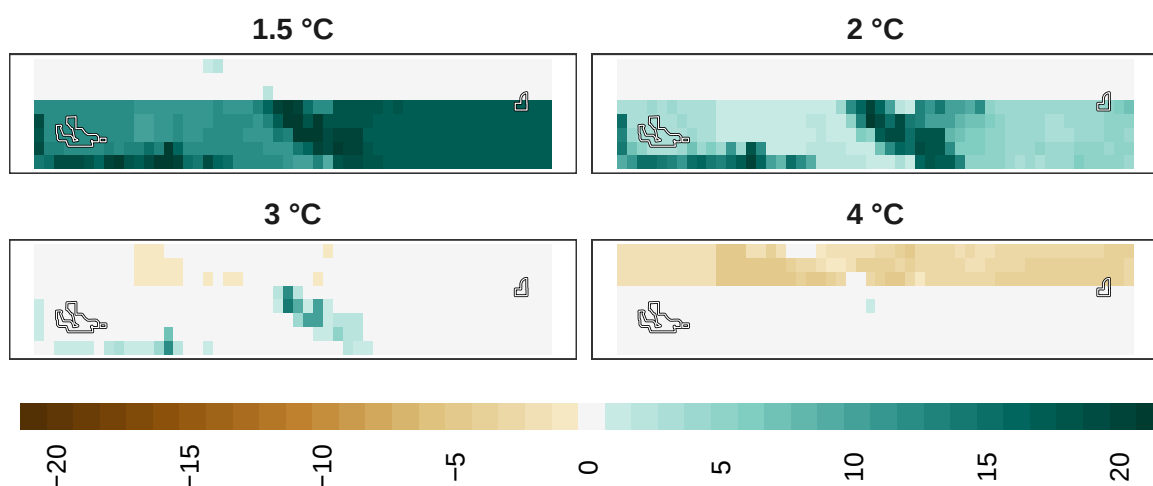
Figure 24: Adaptation effort for insects at 1 km resolution.
