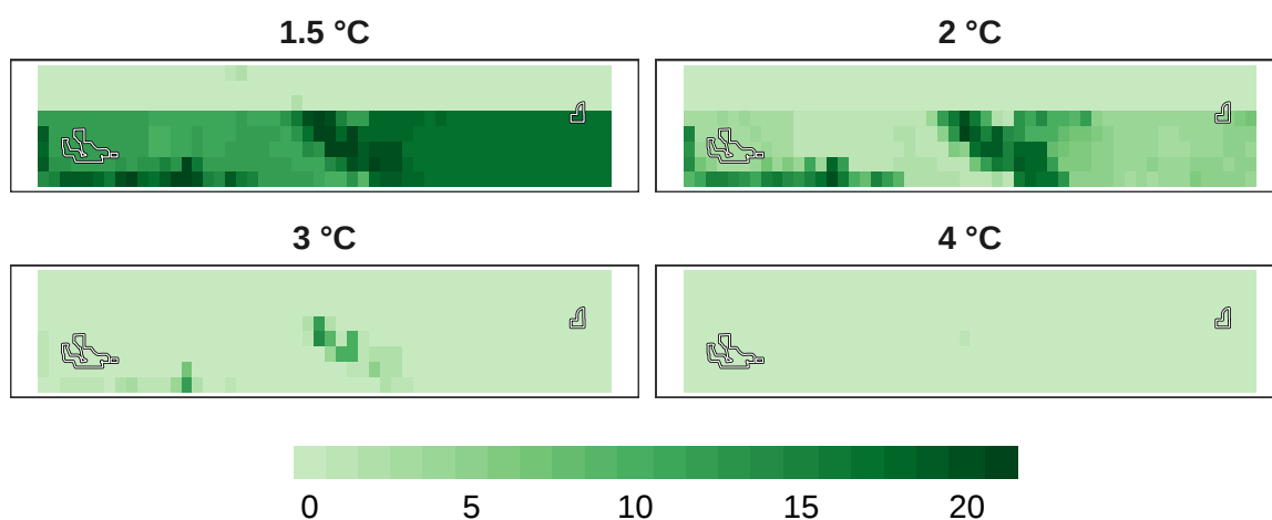
Figure 16: Number of models in agreement for insect refugia at 1 km resolution.
