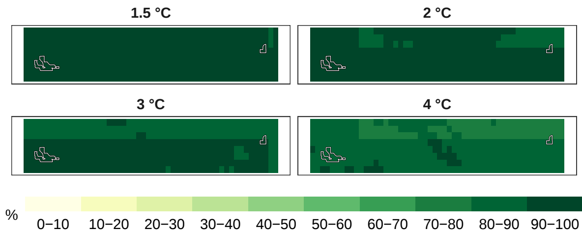
Figure 4: Percent birds remaining at 1 km resolution.
