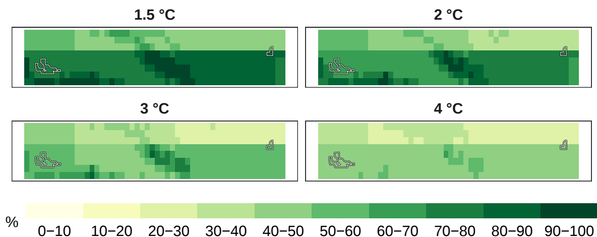
Figure 5: Percent mammals remaining at 1 km resolution.
