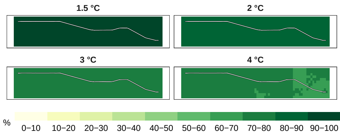
Figure 5: Percent mammals remaining at 1 km resolution.
