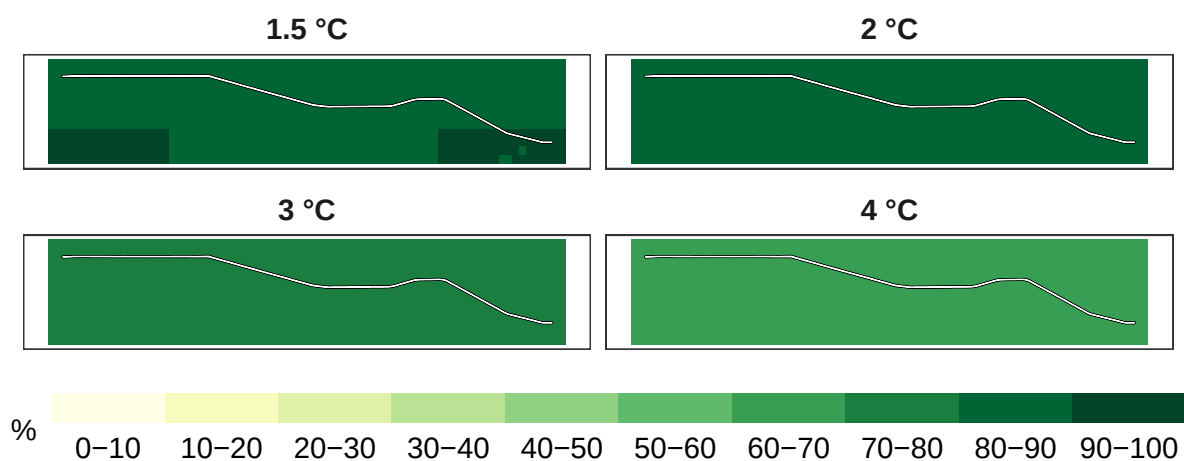
Figure 8: Percent pollinators remaining at 1 km resolution.
