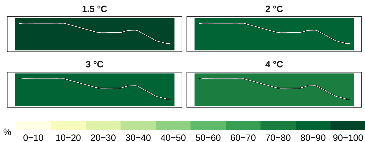
Figure 4: Percent birds remaining at 1 km resolution.
