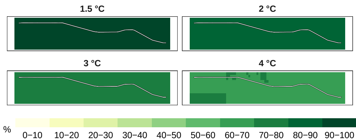
Figure 2: Percent plants remaining at 1 km resolution.
