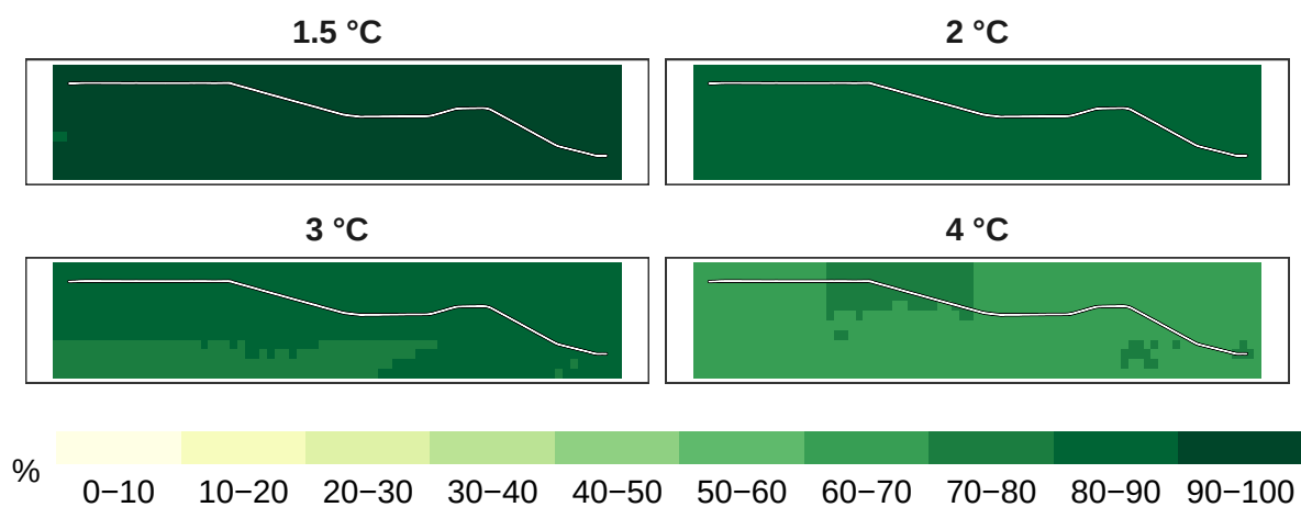
Figure 6: Percent reptiles remaining at 1 km resolution.
