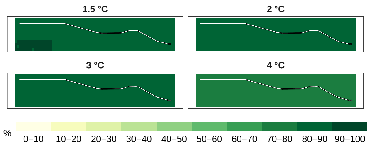
Figure 9: Percent timber species remaining at 1 km resolution.
