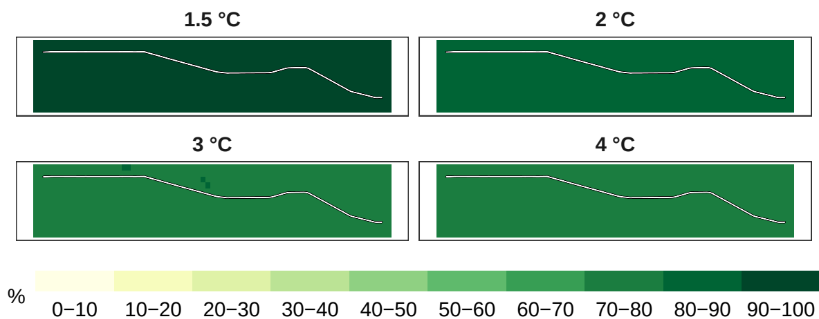
Figure 7: Percent insects remaining at 1 km resolution.
