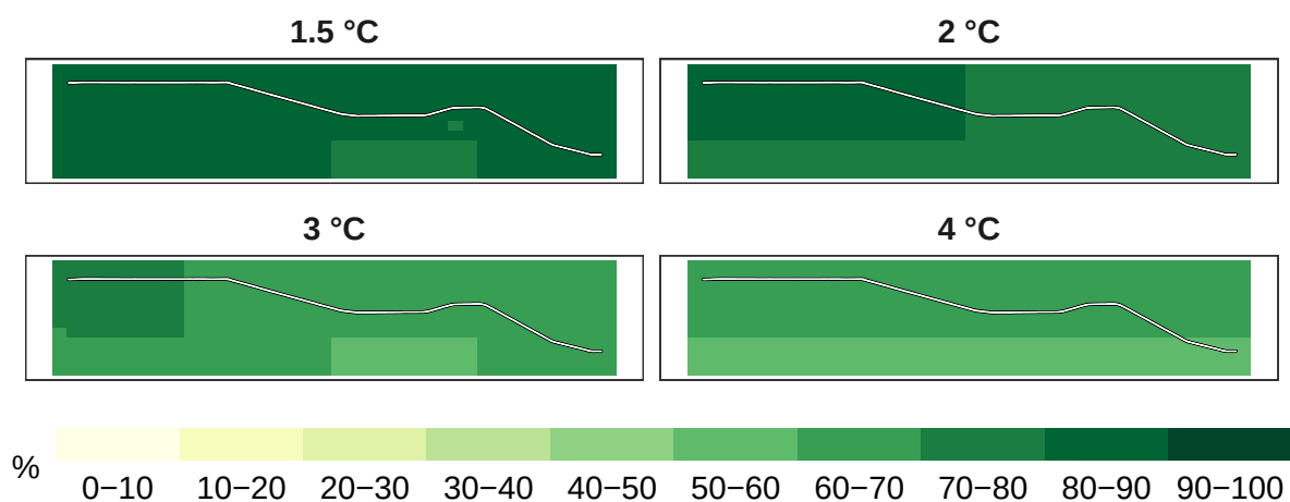
Figure 3: Percent amphibians remaining at 1 km resolution.
