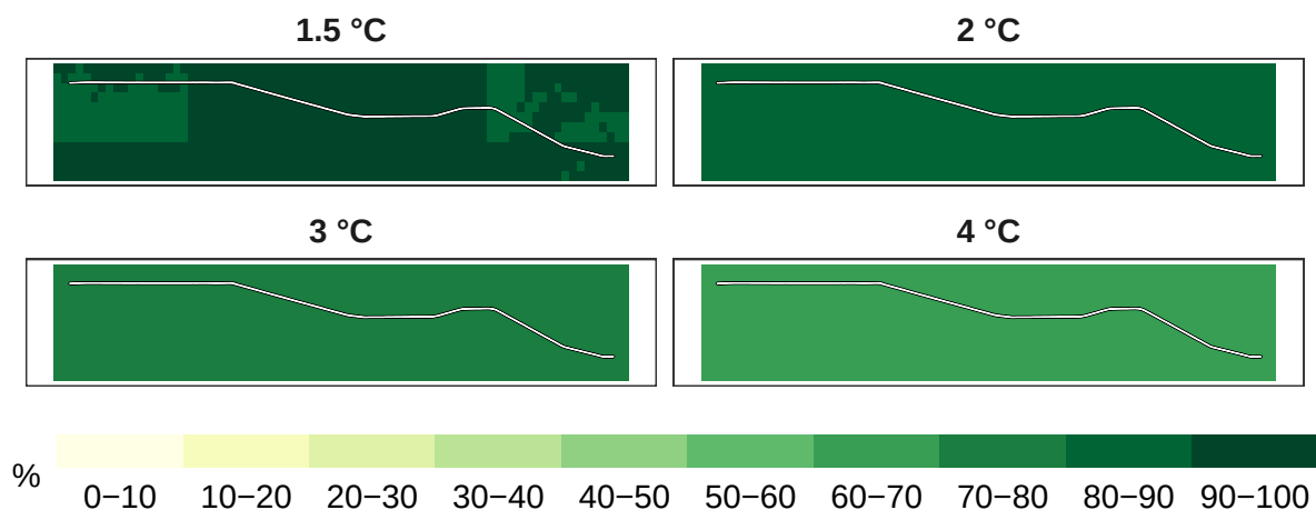
Figure 1: Percent overall biodiversity remaining at 1 km resolution.
