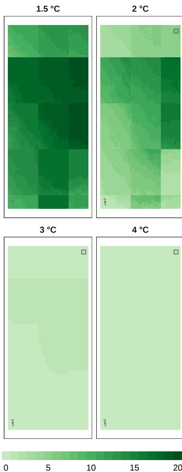
Figure 13: Number of models in agreement for mammal refugia at 1 km resolution.
