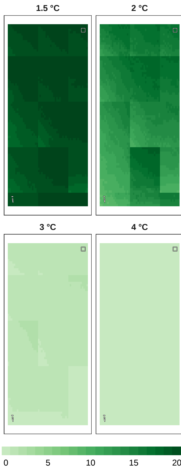
Figure 15: Number of models in agreement for pollinator refugia at 1 km resolution.
