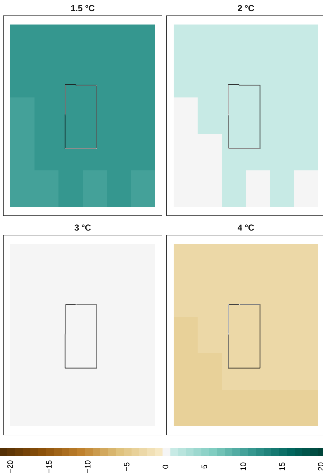
Figure 21: Adaptation effort for insects at 1 km resolution.
