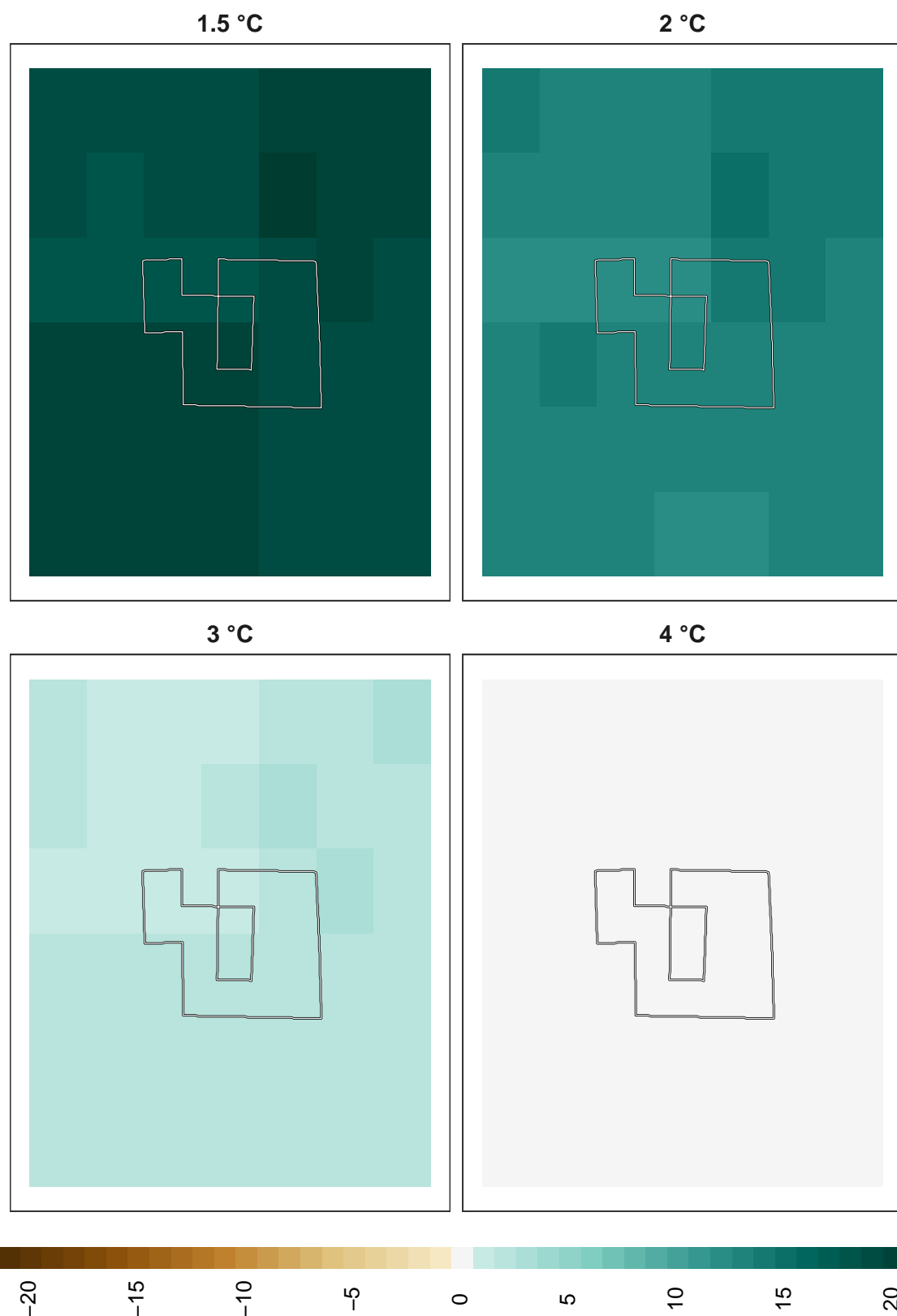
Figure 18: Adaptation effort for amphibians at 1 km resolution.
