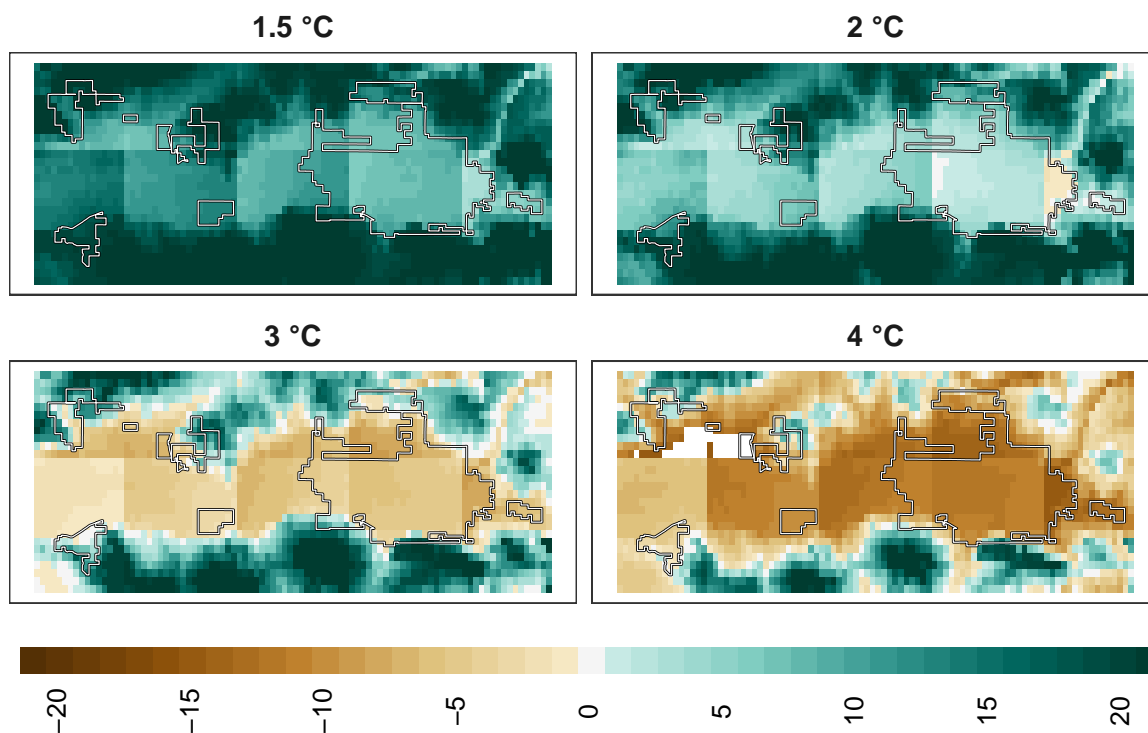
Figure 20: Adaptation effort for mammals at 1 km resolution.
