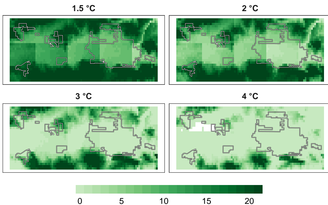
Figure 13: Number of models in agreement for mammal refugia at 1 km resolution.
