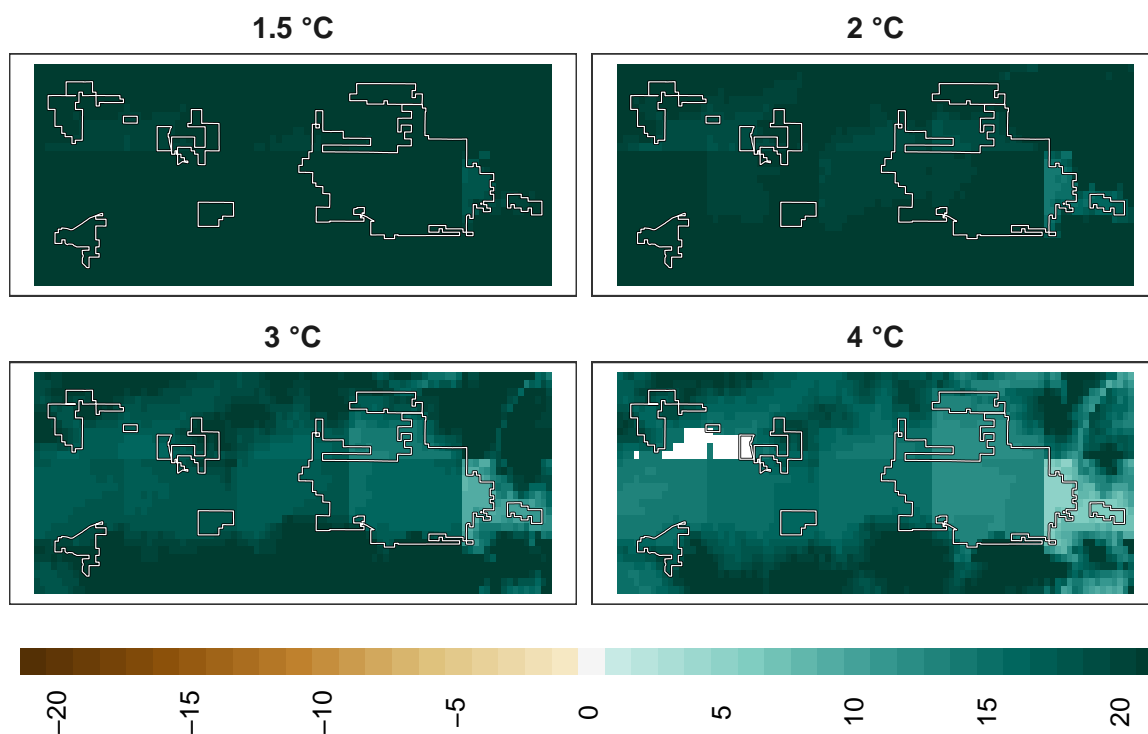
Figure 19: Adaptation effort for birds at 1 km resolution.
