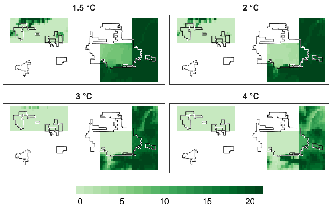
Figure 11: Number of models in agreement for amphibian refugia at 1 km resolution.
