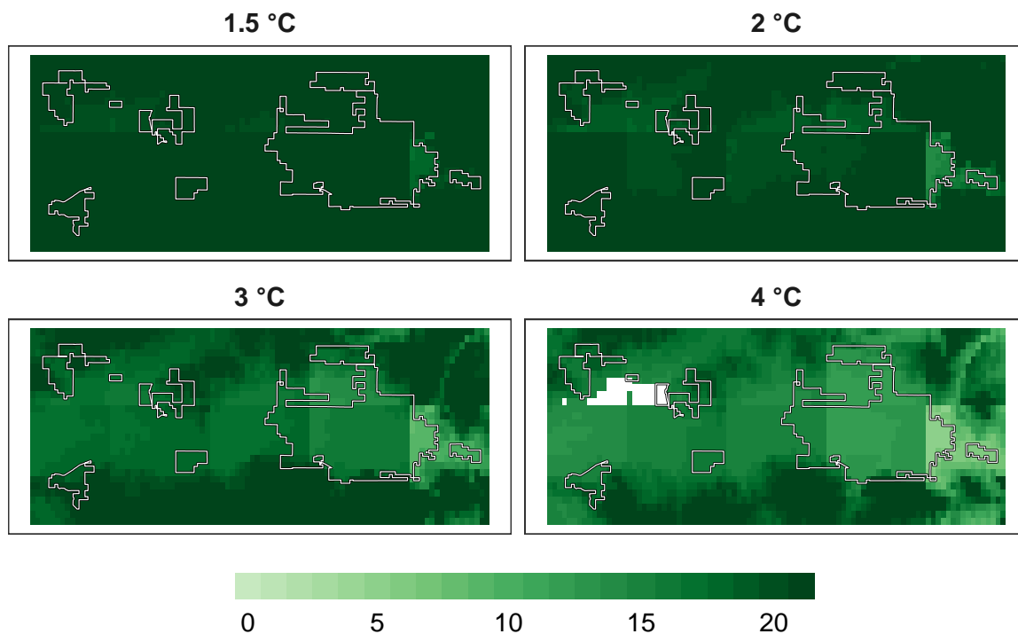
Figure 12: Number of models in agreement for bird refugia.
