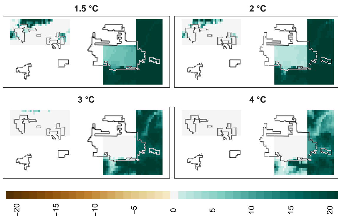
Figure 18: Adaptation effort for amphibians at 1 km resolution.
