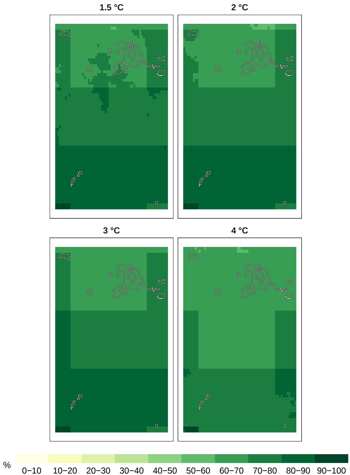
Figure 7: Percent pollinators remaining at 1 km resolution.
