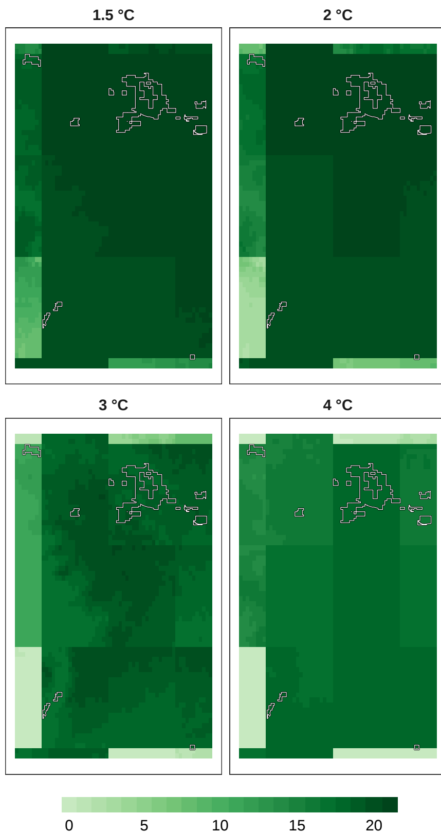
Figure 10: Number of models in agreement for amphibian refugia at 1 km resolution.
