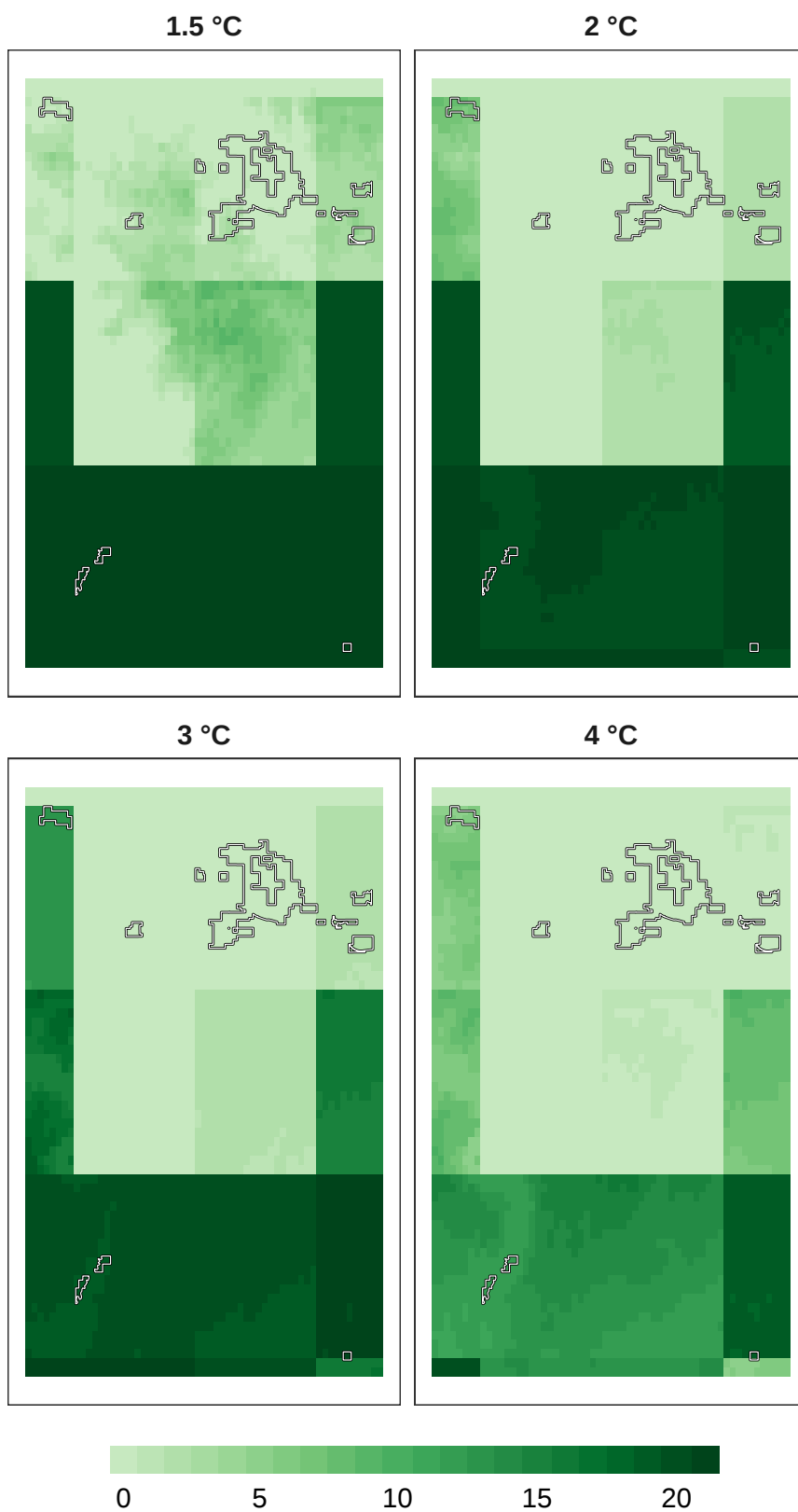
Figure 14: Number of models in agreement for pollinator refugia at 1 km resolution.
