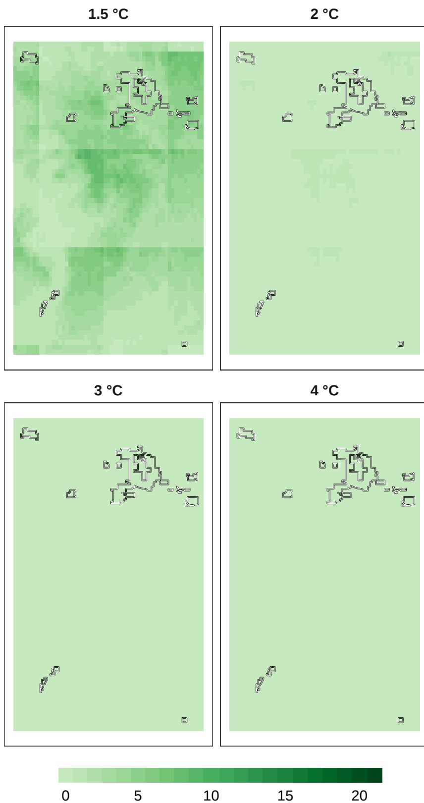
Figure 13: Number of models in agreement for insect refugia at 1 km resolution.
