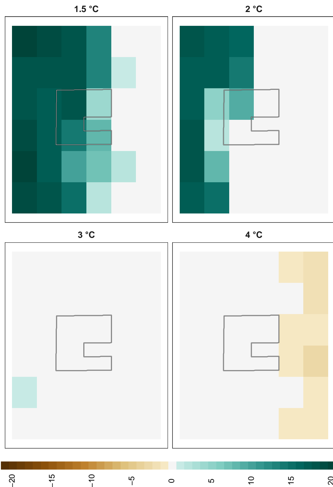
Figure 17: Adaptation effort for overall biodiversity at 1 km resolution.
