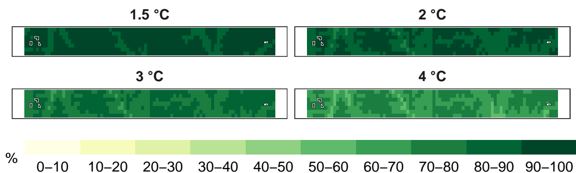
Figure 8: Percent pollinators remaining at 1 km resolution.
