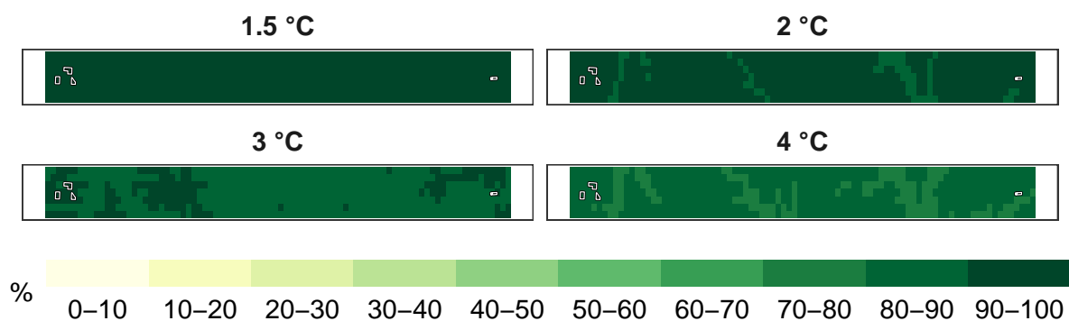
Figure 9: Percent timber species remaining at 1 km resolution.
