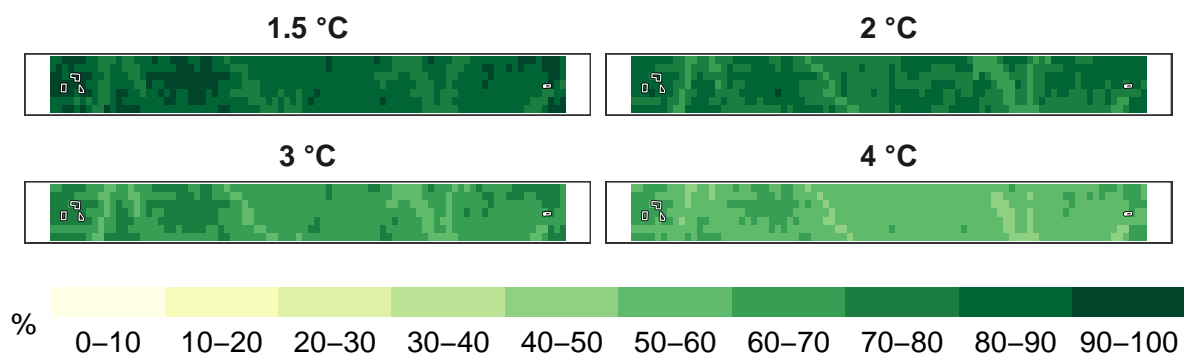
Figure 1: Percent overall biodiversity remaining at 1 km resolution.
