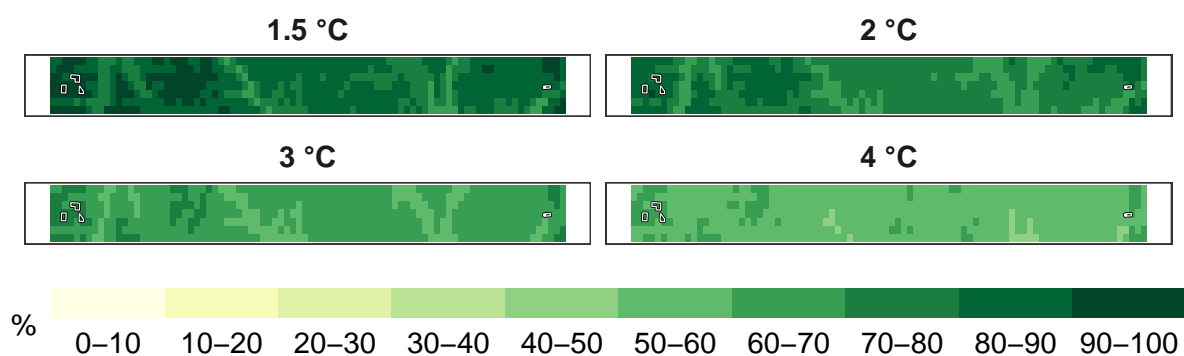
Figure 5: Percent mammals remaining at 1 km resolution.
