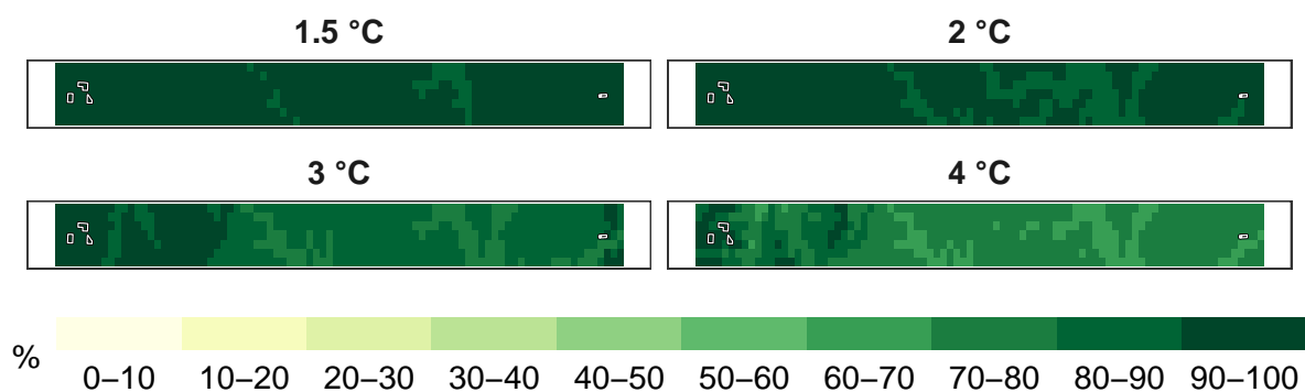
Figure 6: Percent reptiles remaining at 1 km resolution.
