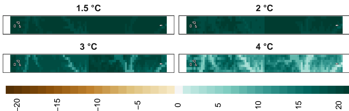
Figure 20: Adaptation effort for amphibians at 1 km resolution.
