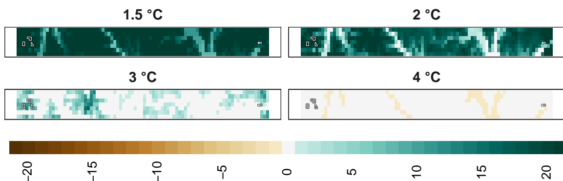
Figure 19: Adaptation effort for plants at 1 km resolution.
