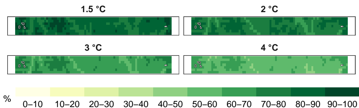
Figure 2: Percent plants remaining at 1 km resolution.
