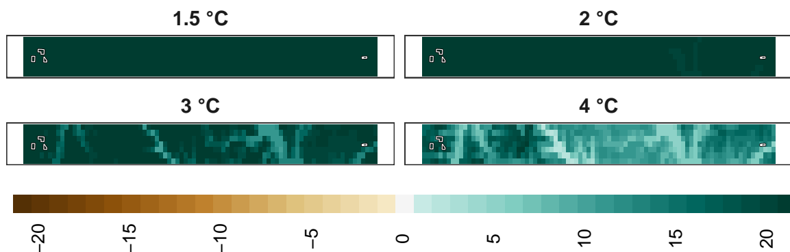
Figure 23: Adaptation effort for reptiles at 1 km resolution.
