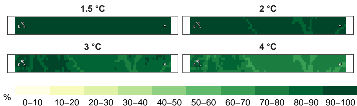
Figure 3: Percent amphibians remaining at 1 km resolution.
