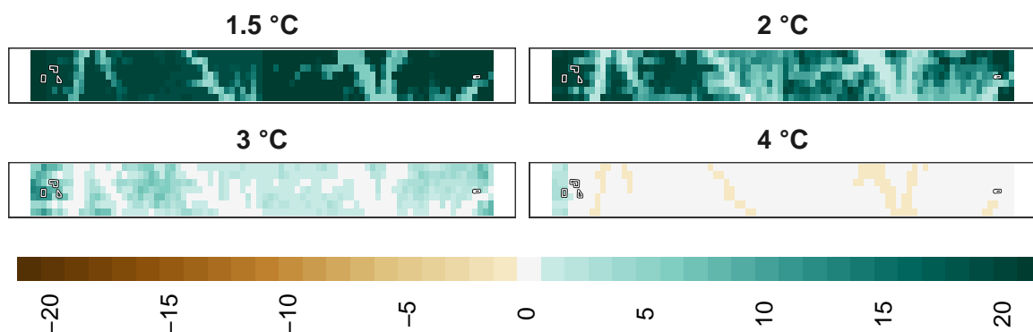
Figure 22: Adaptation effort for mammals at 1 km resolution.
