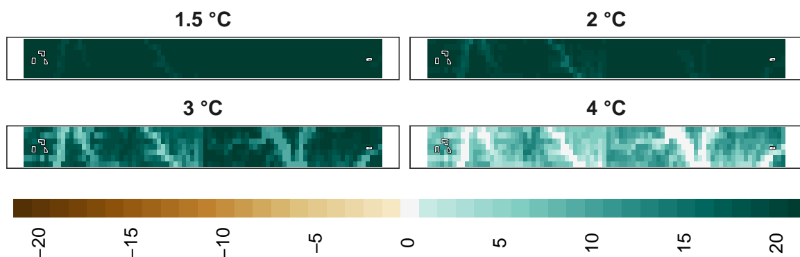
Figure 25: Adaptation effort for pollinators at 1 km resolution.
