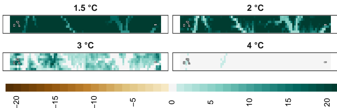
Figure 24: Adaptation effort for insects at 1 km resolution.
