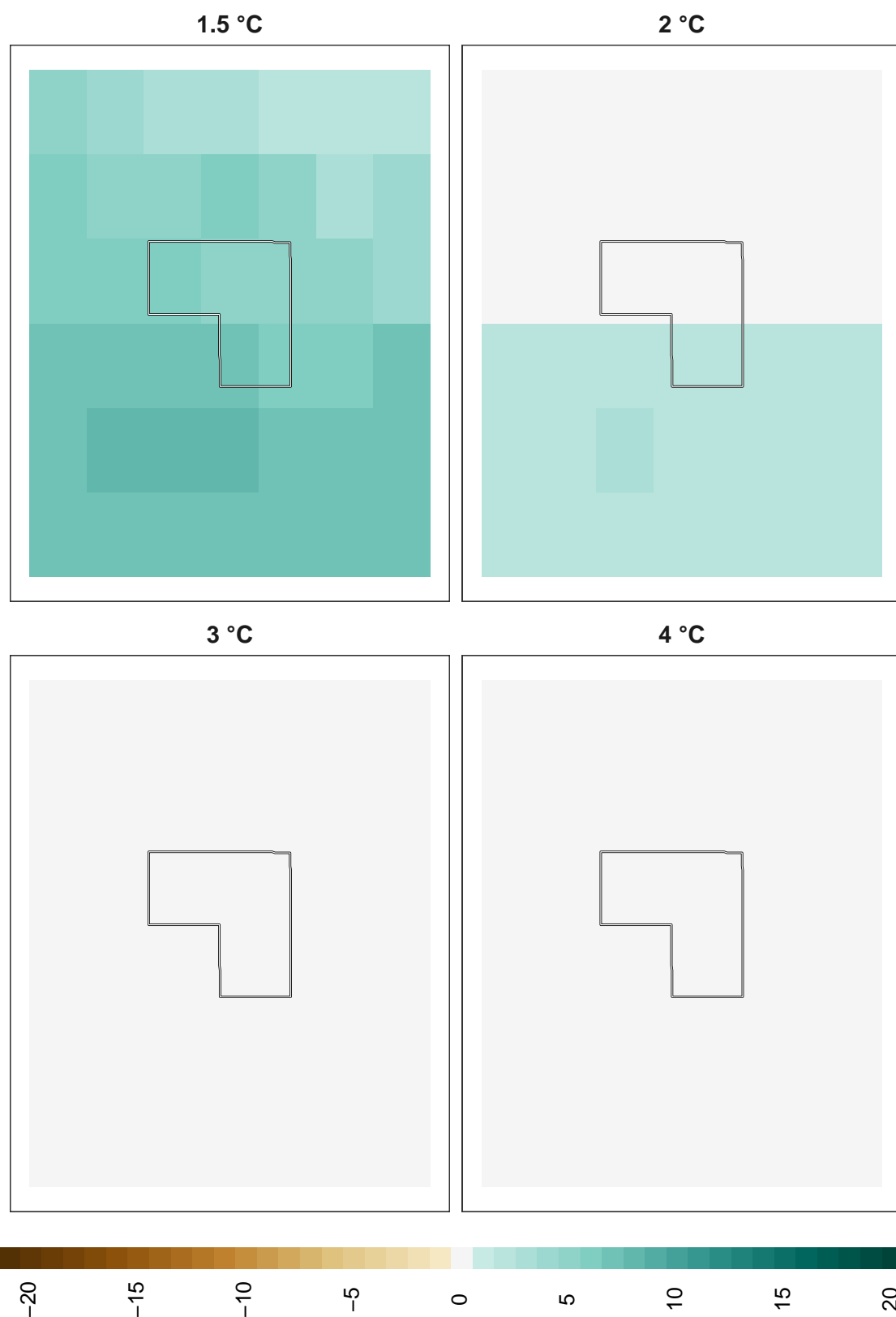
Figure 21: Adaptation effort for pollinators at 1 km resolution.
