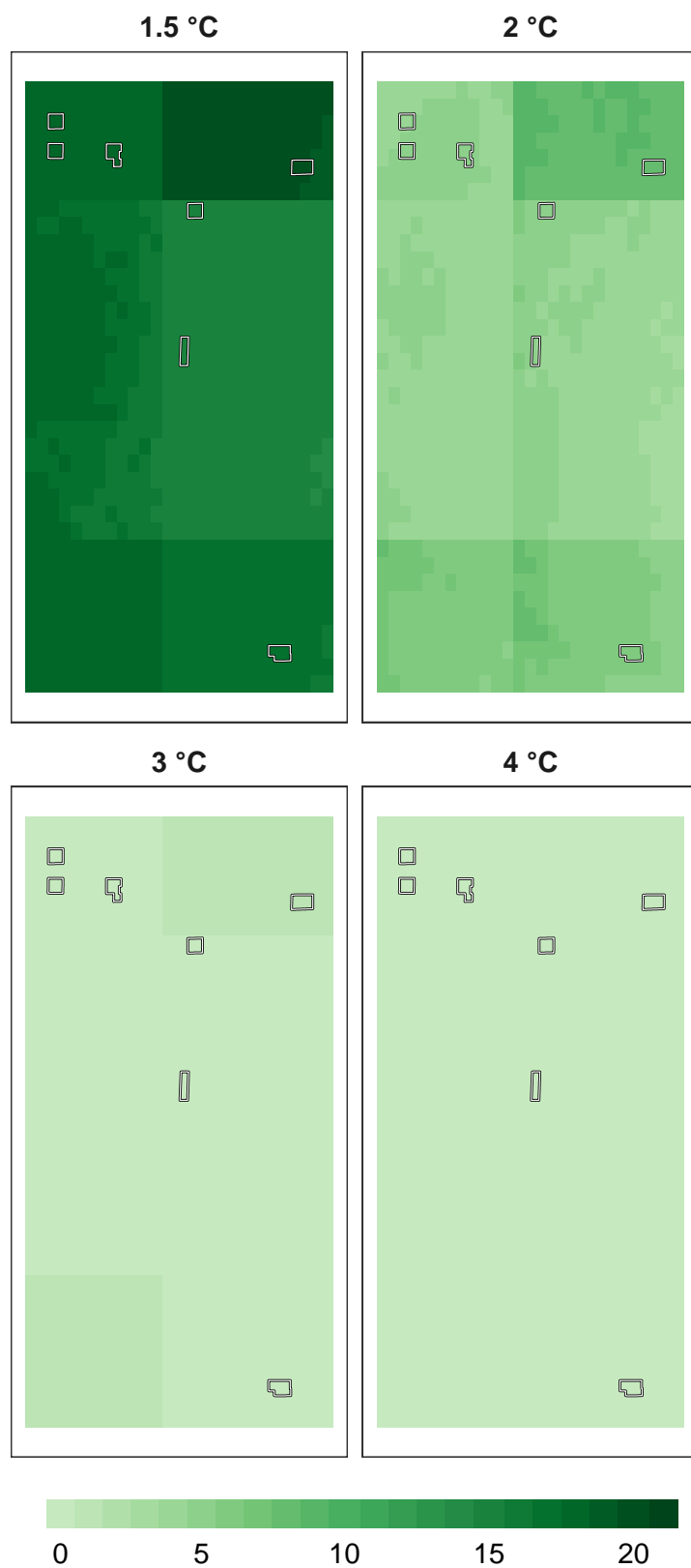
Figure 14: Number of models in agreement for pollinator refugia at 1 km resolution.
