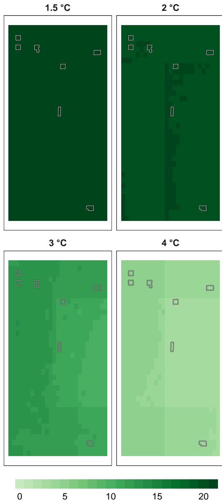
Figure 10: Number of models in agreement for amphibian refugia at 1 km resolution.
