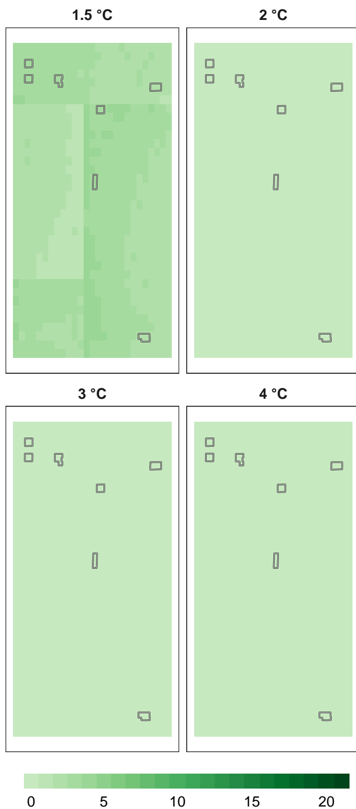
Figure 13: Number of models in agreement for insect refugia at 1 km resolution.
