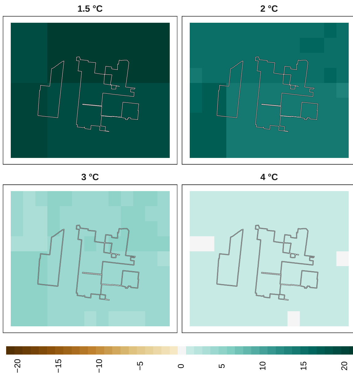
Figure 24: Adaptation effort for insects at 1 km resolution.
