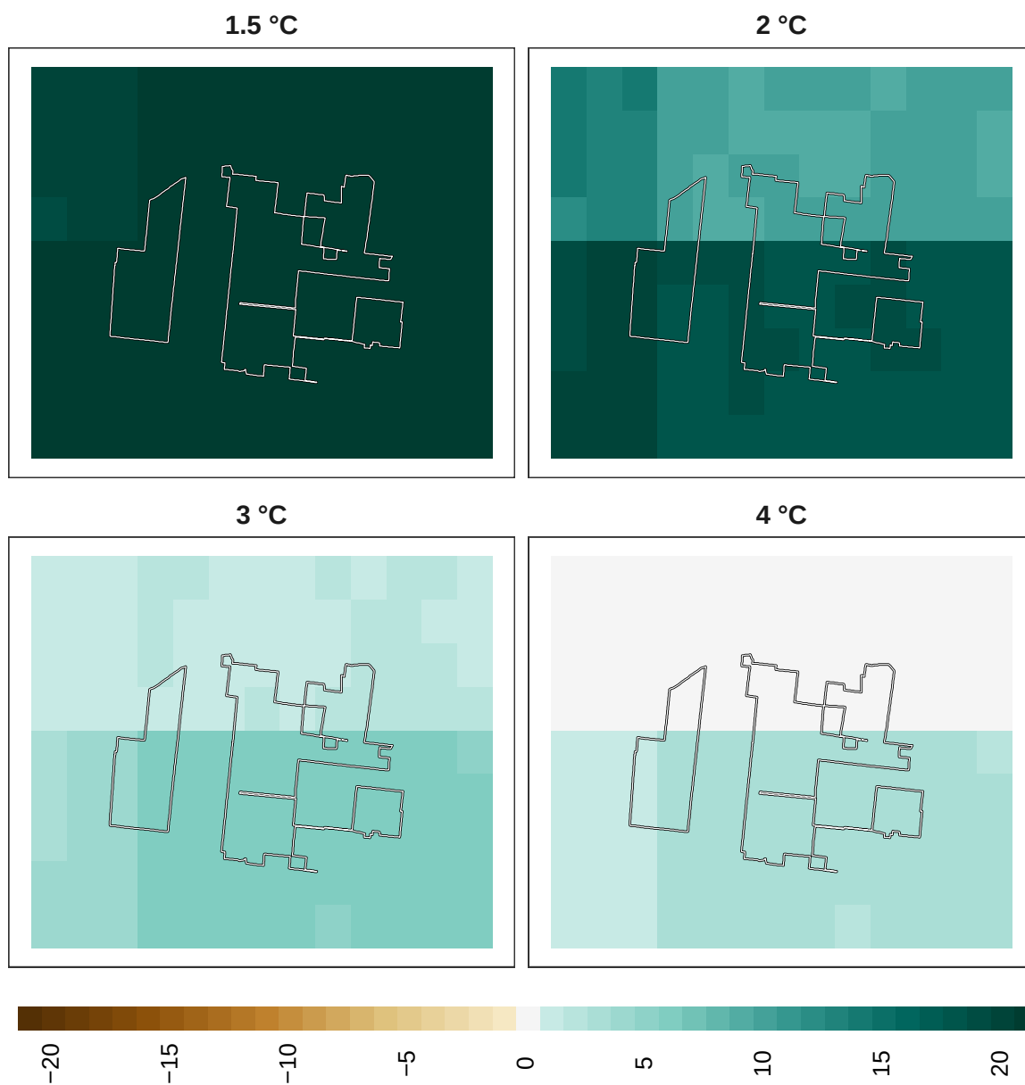
Figure 23: Adaptation effort for reptiles at 1 km resolution.
