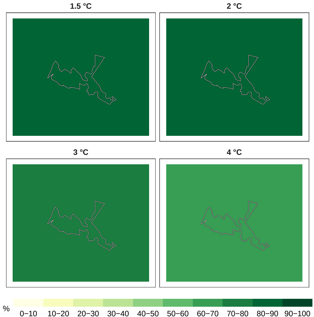
Figure 1: Percent overall biodiversity remaining at 1 km resolution.
