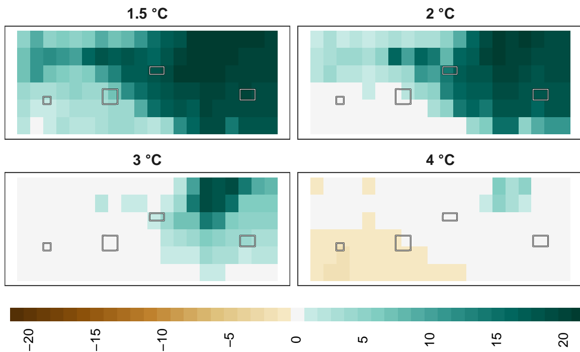
Figure 23: Adaptation effort for insects at 1 km resolution.
