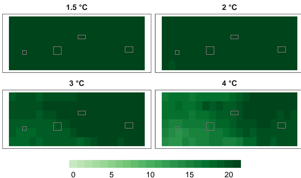
Figure 16: Number of models in agreement for pollinator refugia at 1 km resolution.
