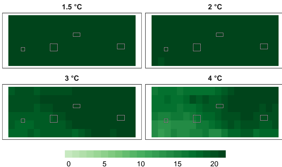
Figure 12: Number of models in agreement for bird refugia.
