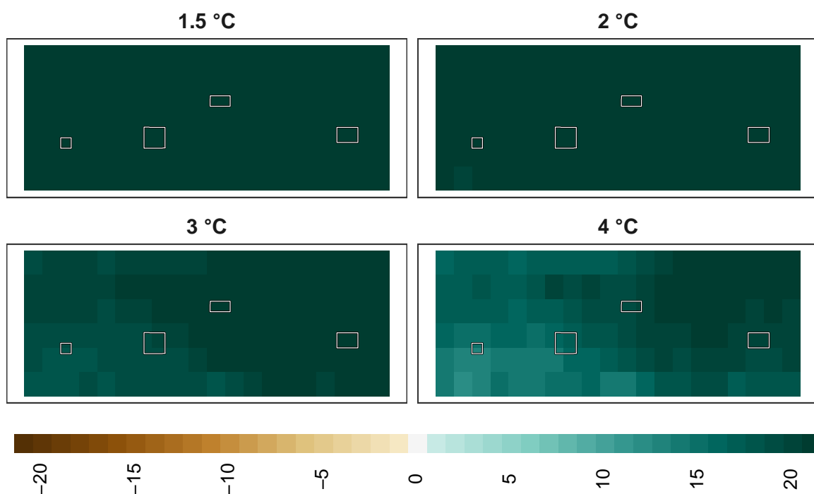
Figure 20: Adaptation effort for birds at 1 km resolution.
