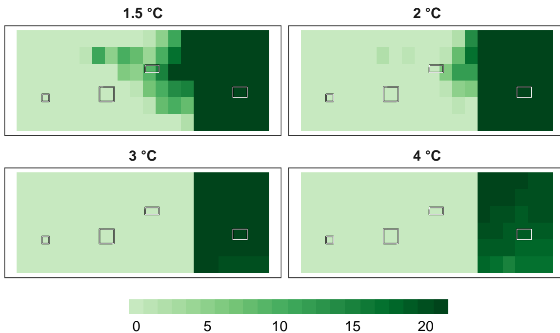
Figure 11: Number of models in agreement for amphibian refugia at 1 km resolution.
