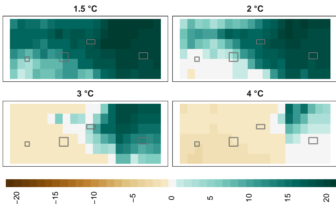
Figure 21: Adaptation effort for mammals at 1 km resolution.
