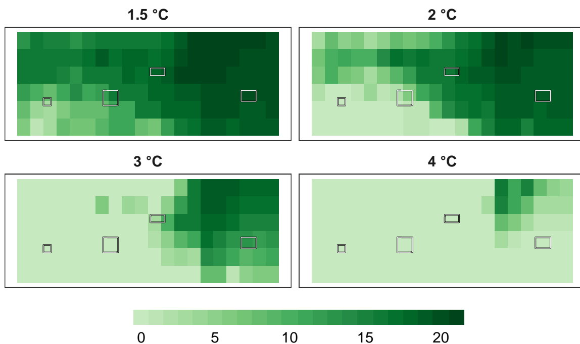
Figure 13: Number of models in agreement for mammal refugia at 1 km resolution.
