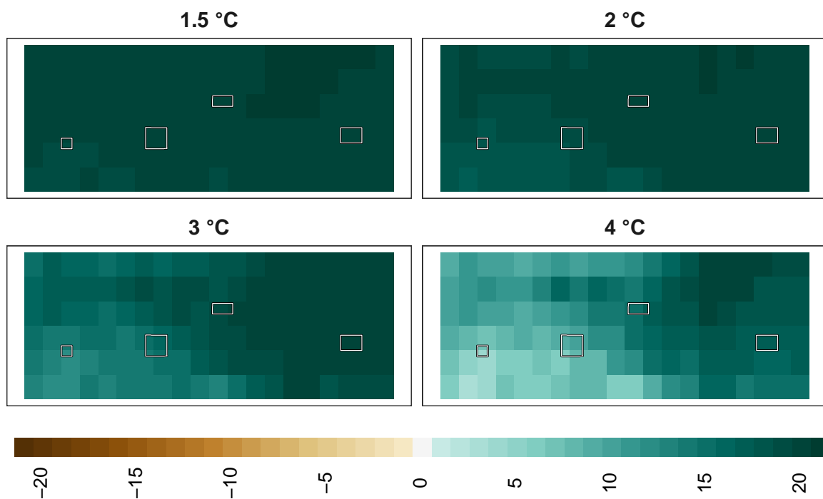
Figure 22: Adaptation effort for reptiles at 1 km resolution.
