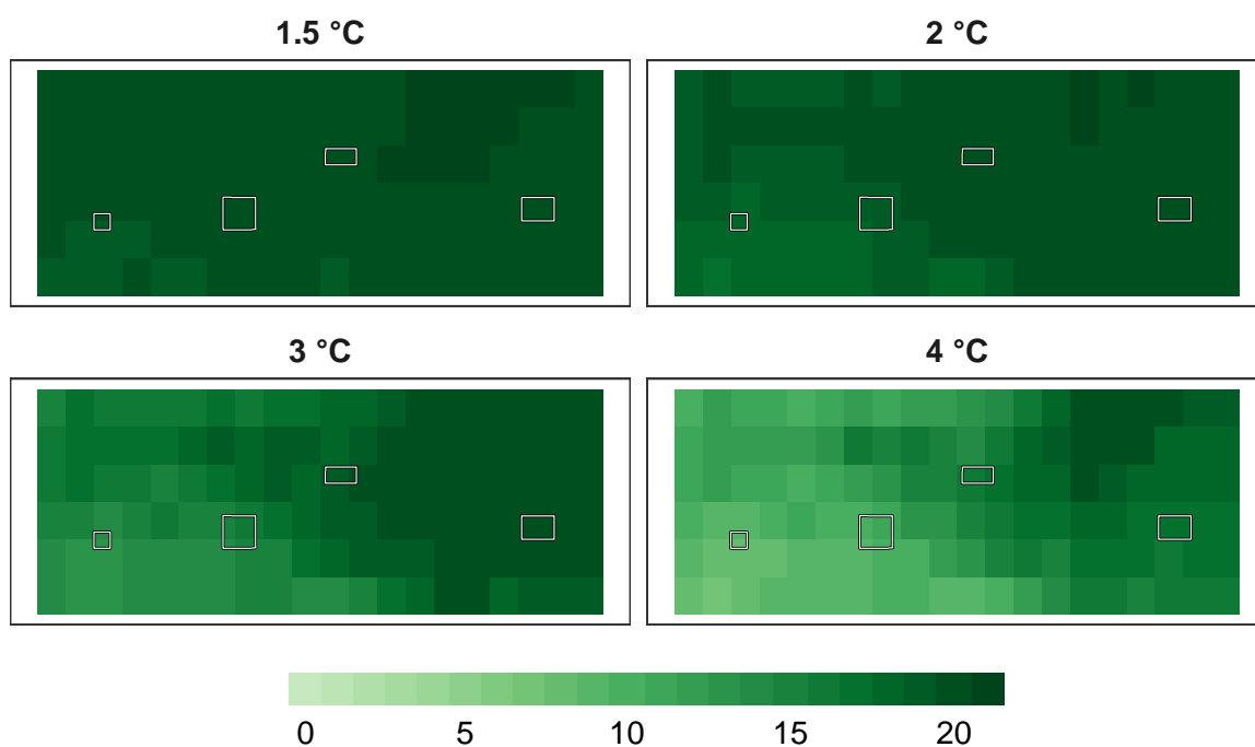
Figure 14: Number of models in agreement for reptile refugia at 1 km resolution.
