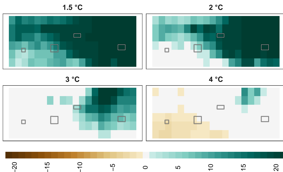
Figure 17: Adaptation effort for overall biodiversity at 1 km resolution.
