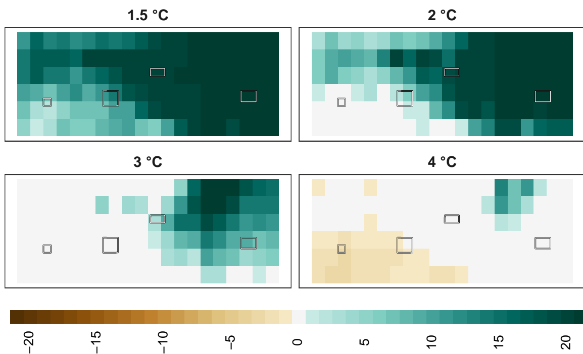
Figure 18: Adaptation effort for plants at 1 km resolution.
