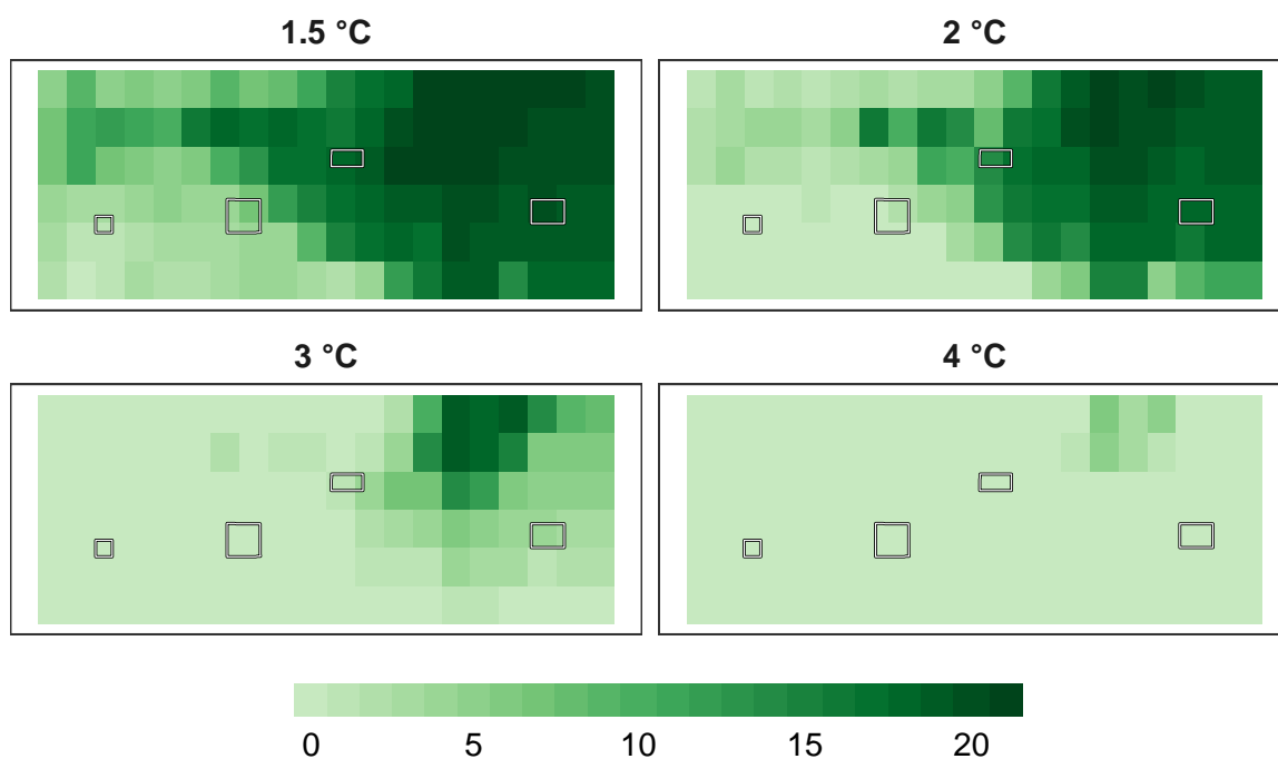
Figure 15: Number of models in agreement for insect refugia at 1 km resolution.
