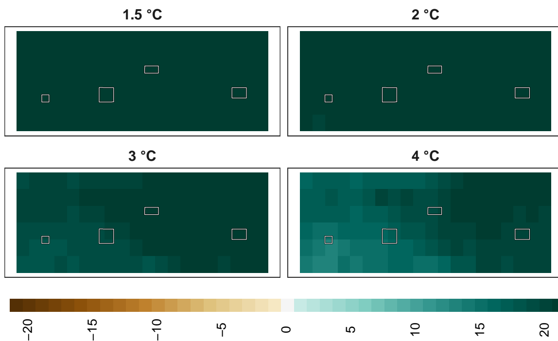
Figure 24: Adaptation effort for pollinators at 1 km resolution.
