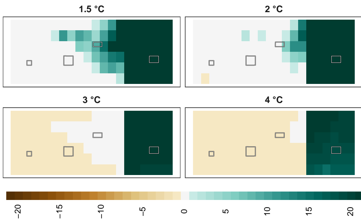
Figure 19: Adaptation effort for amphibians at 1 km resolution.
