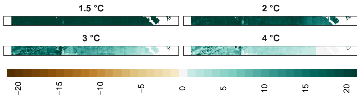
Figure 25: Adaptation effort for pollinators at 1 km resolution.
