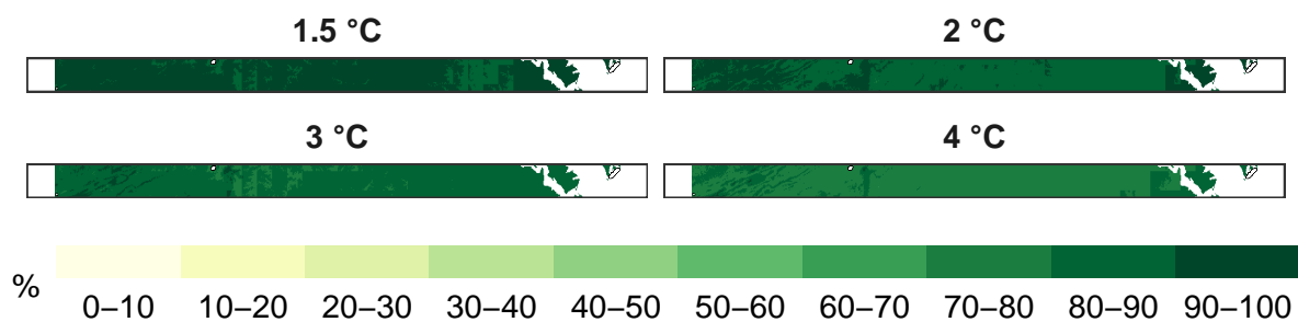
Figure 4: Percent birds remaining at 1 km resolution.
