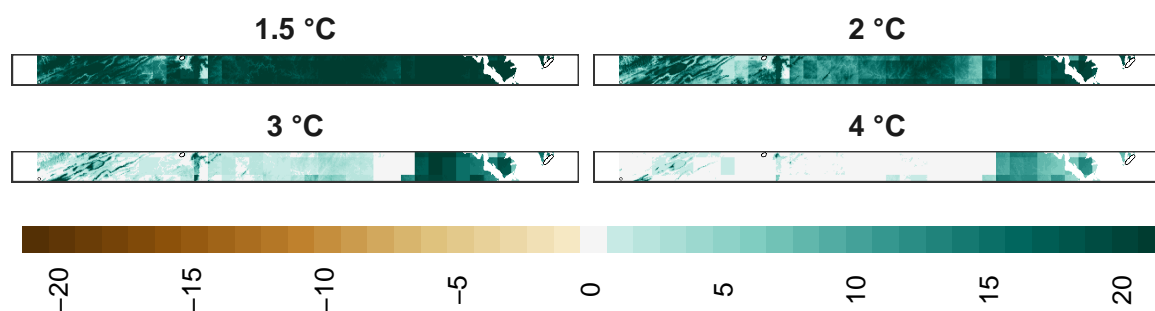
Figure 22: Adaptation effort for mammals at 1 km resolution.
