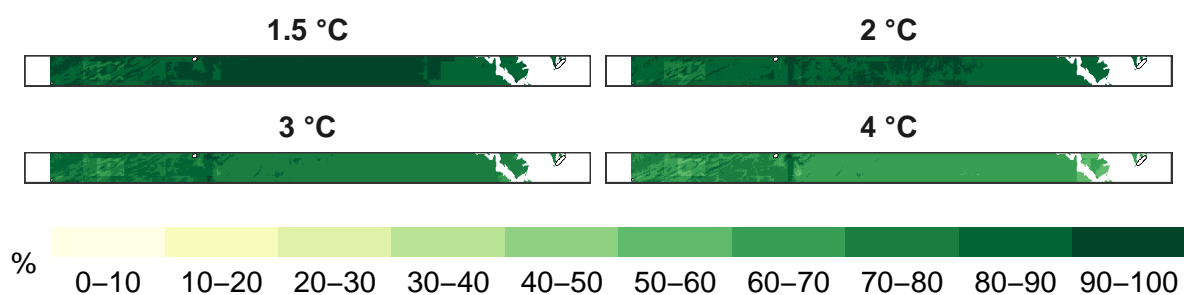
Figure 9: Percent timber species remaining at 1 km resolution.
