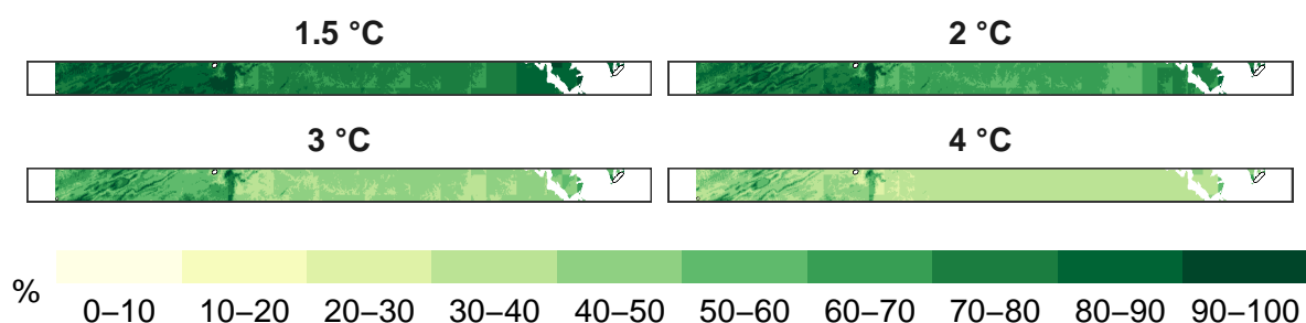
Figure 3: Percent amphibians remaining at 1 km resolution.
