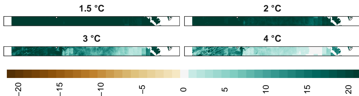
Figure 23: Adaptation effort for reptiles at 1 km resolution.
