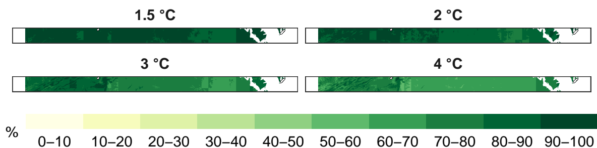
Figure 6: Percent reptiles remaining at 1 km resolution.
