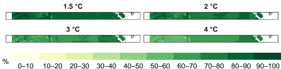
Figure 5: Percent mammals remaining at 1 km resolution.
