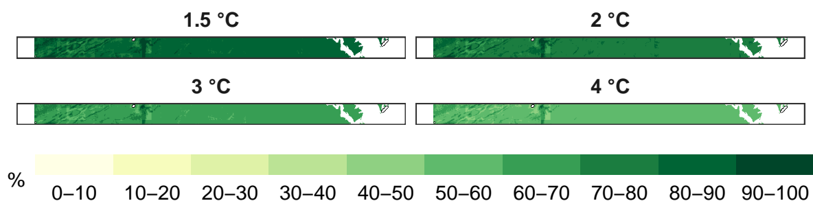
Figure 2: Percent plants remaining at 1 km resolution.
