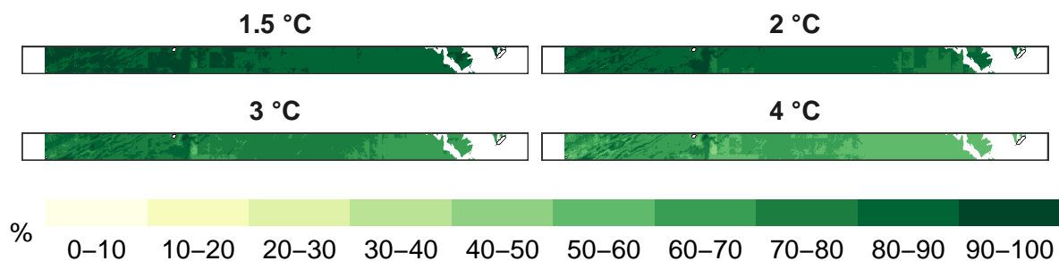
Figure 8: Percent pollinators remaining at 1 km resolution.
