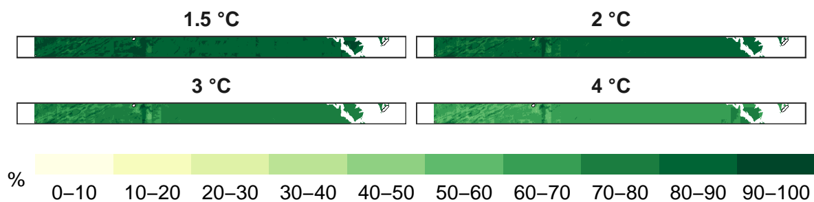
Figure 7: Percent insects remaining at 1 km resolution.
