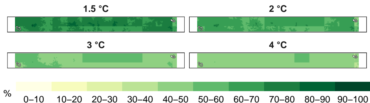
Figure 5: Percent mammals remaining at 1 km resolution.
