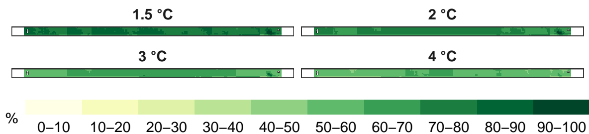
Figure 7: Percent insects remaining at 1 km resolution.
