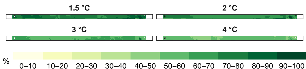
Figure 3: Percent amphibians remaining at 1 km resolution.
