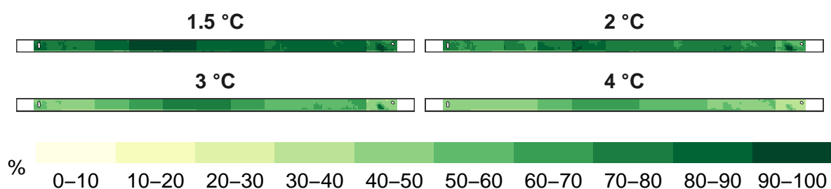
Figure 6: Percent reptiles remaining at 1 km resolution.
