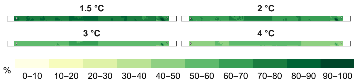
Figure 4: Percent birds remaining at 1 km resolution.
