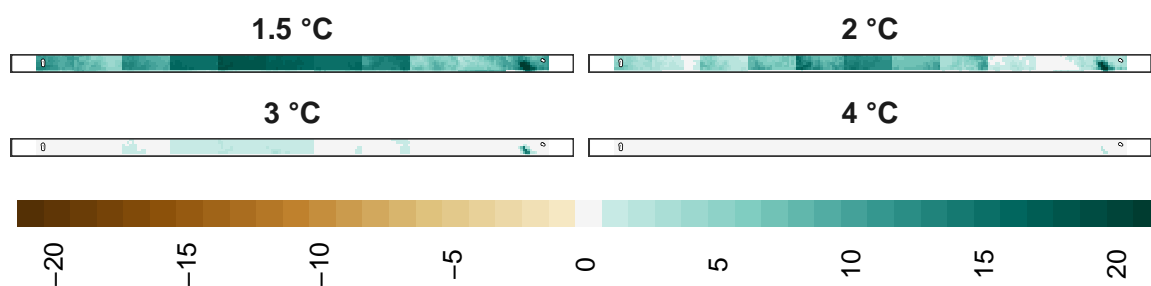
Figure 22: Adaptation effort for mammals at 1 km resolution.
