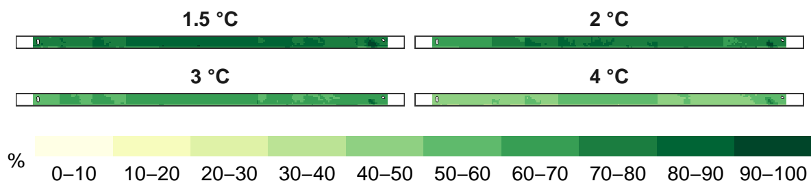
Figure 9: Percent timber species remaining at 1 km resolution.
