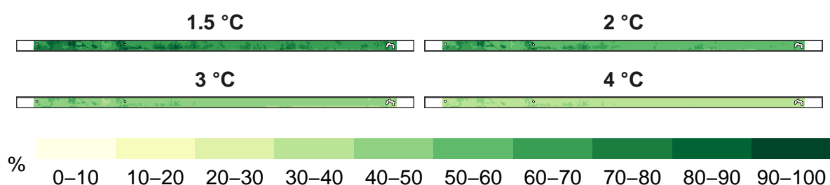
Figure ES1: Percent overall biodiversity remaining at 1 km resolution.
