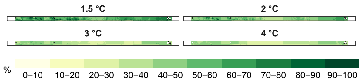
Figure 6: Percent reptiles remaining at 1 km resolution.
