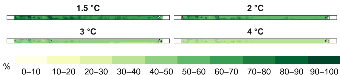
Figure 1: Percent overall biodiversity remaining at 1 km resolution.
