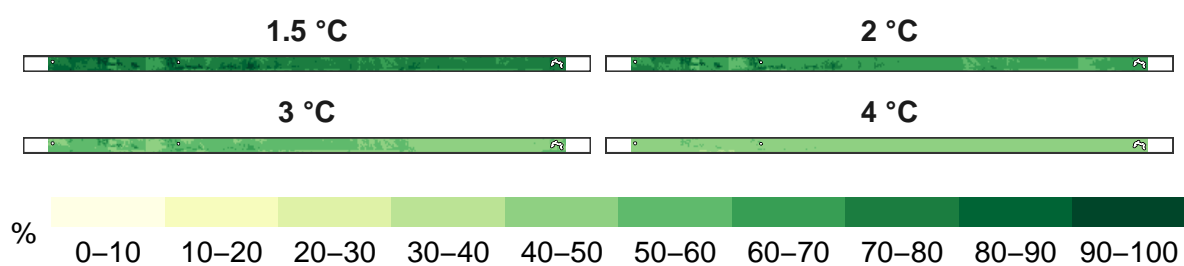
Figure 5: Percent mammals remaining at 1 km resolution.
