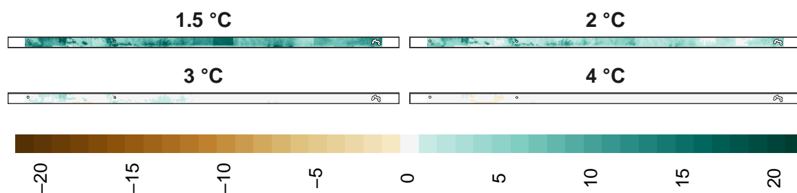
Figure 20: Adaptation effort for amphibians at 1 km resolution.
