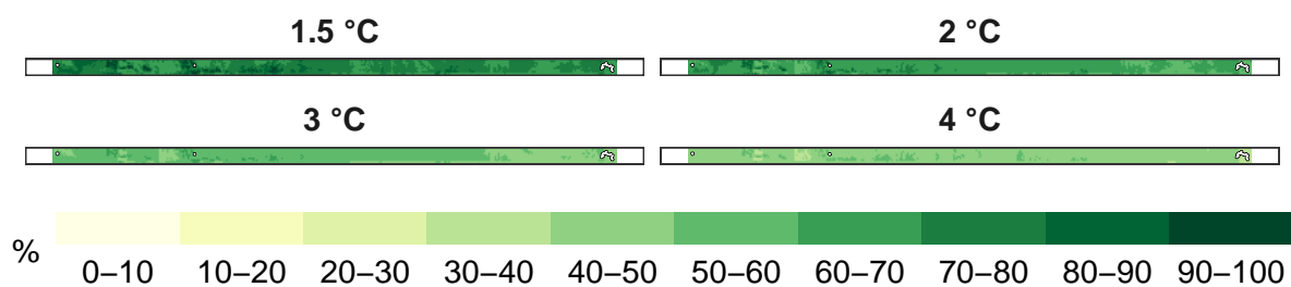
Figure 4: Percent birds remaining at 1 km resolution.
