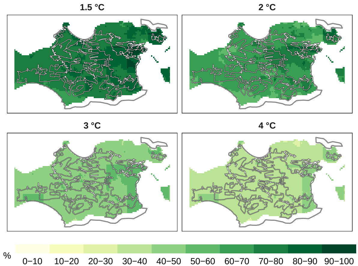
Figure 5: Percent mammals remaining at 1 km resolution.
