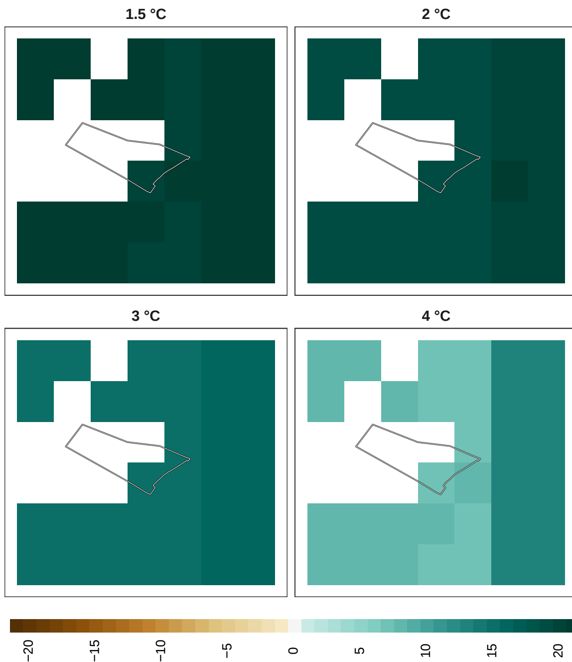
Figure 22: Adaptation effort for reptiles at 1 km resolution.
