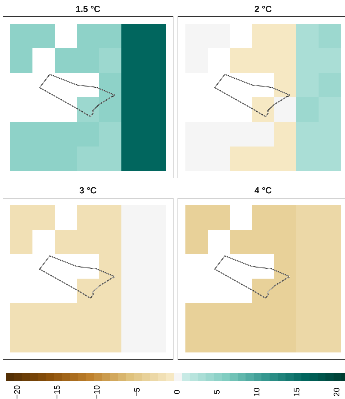
Figure 18: Adaptation effort for plants at 1 km resolution.
