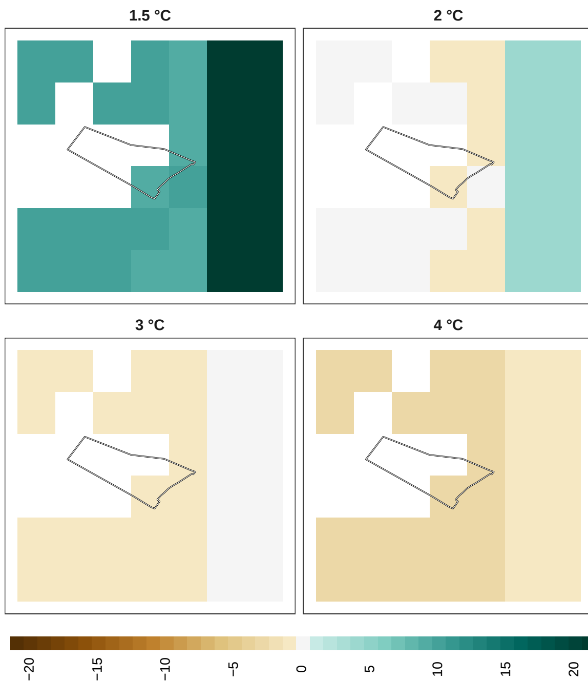
Figure 20: Adaptation effort for birds at 1 km resolution.
