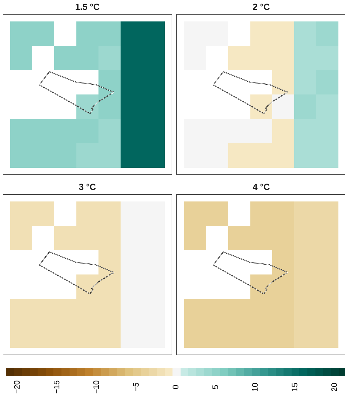
Figure 17: Adaptation effort for overall biodiversity at 1 km resolution.
