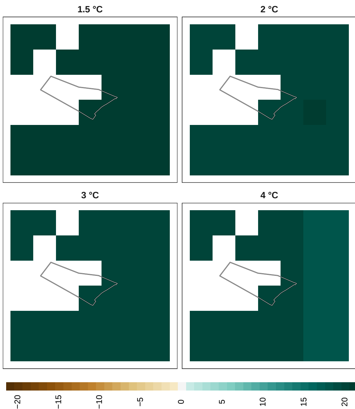
Figure 24: Adaptation effort for pollinators at 1 km resolution.
