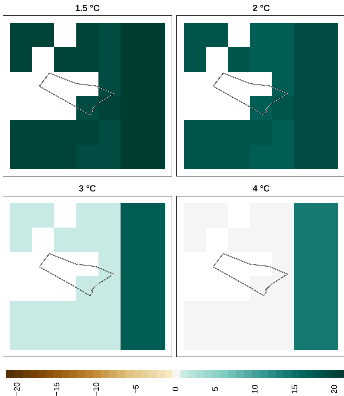
Figure 21: Adaptation effort for mammals at 1 km resolution.
