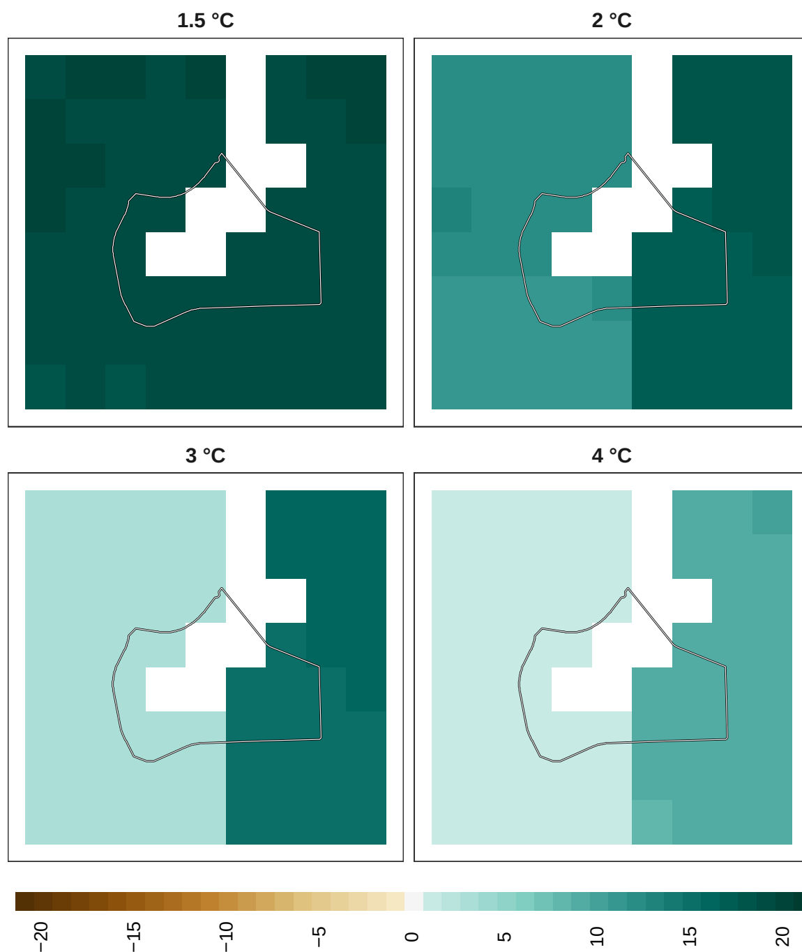
Figure 21: Adaptation effort for mammals at 1 km resolution.
