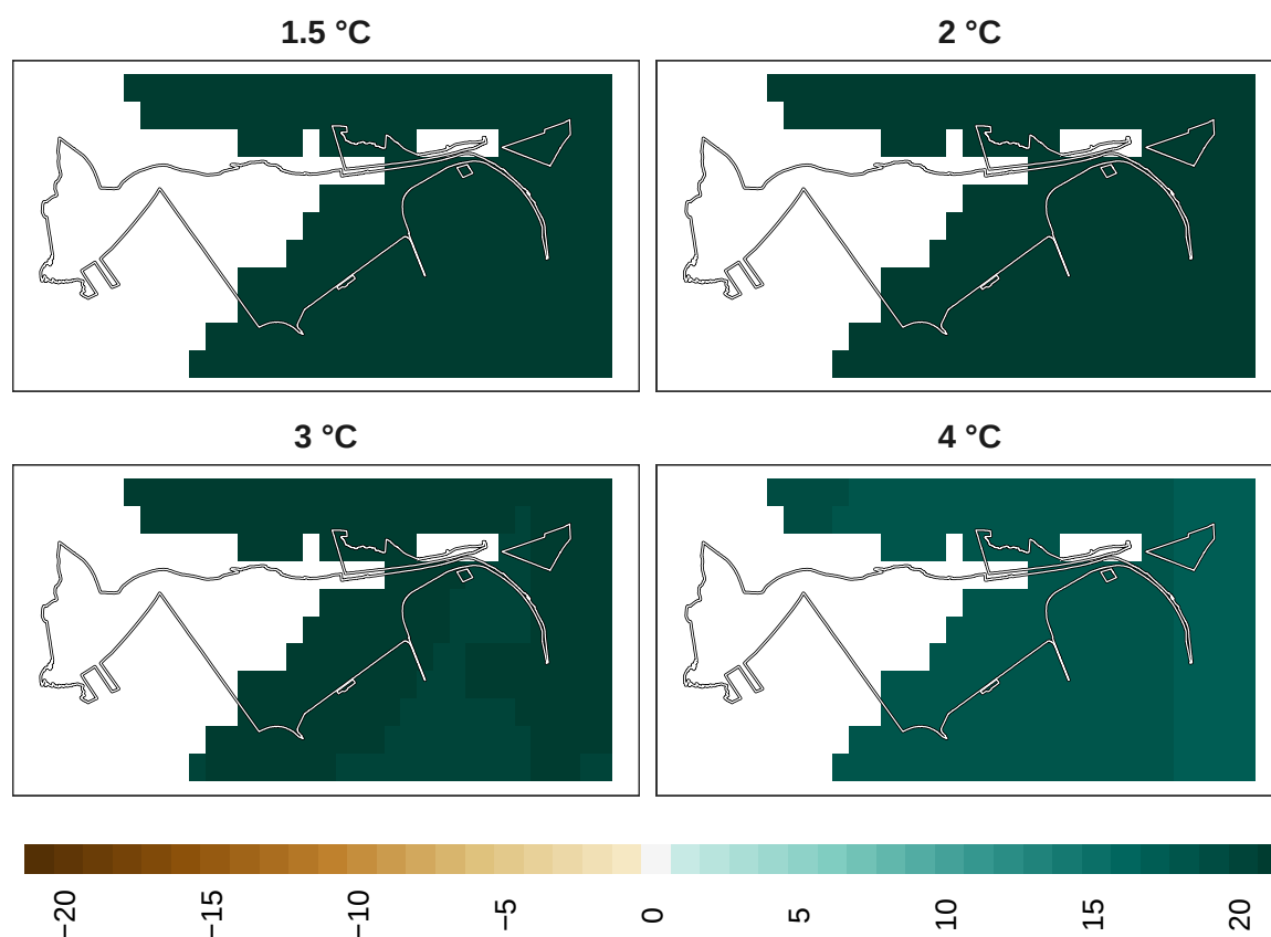
Figure 21: Adaptation effort for birds at 1 km resolution.
