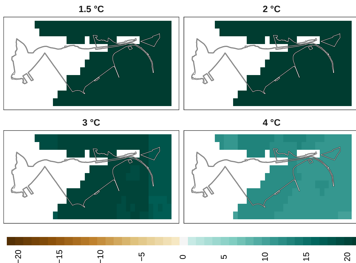
Figure 22: Adaptation effort for mammals at 1 km resolution.
