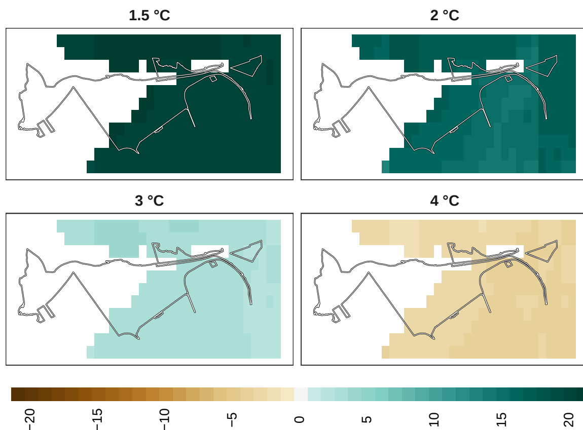
Figure 18: Adaptation effort for overall biodiversity at 1 km resolution.
