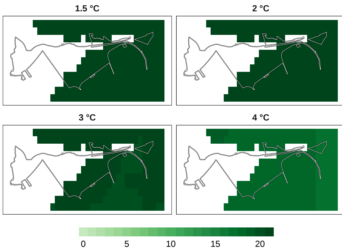
Figure 13: Number of models in agreement for bird refugia.
