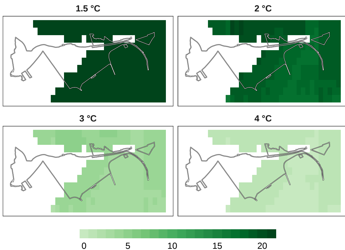
Figure 17: Number of models in agreement for pollinator refugia at 1 km resolution.
