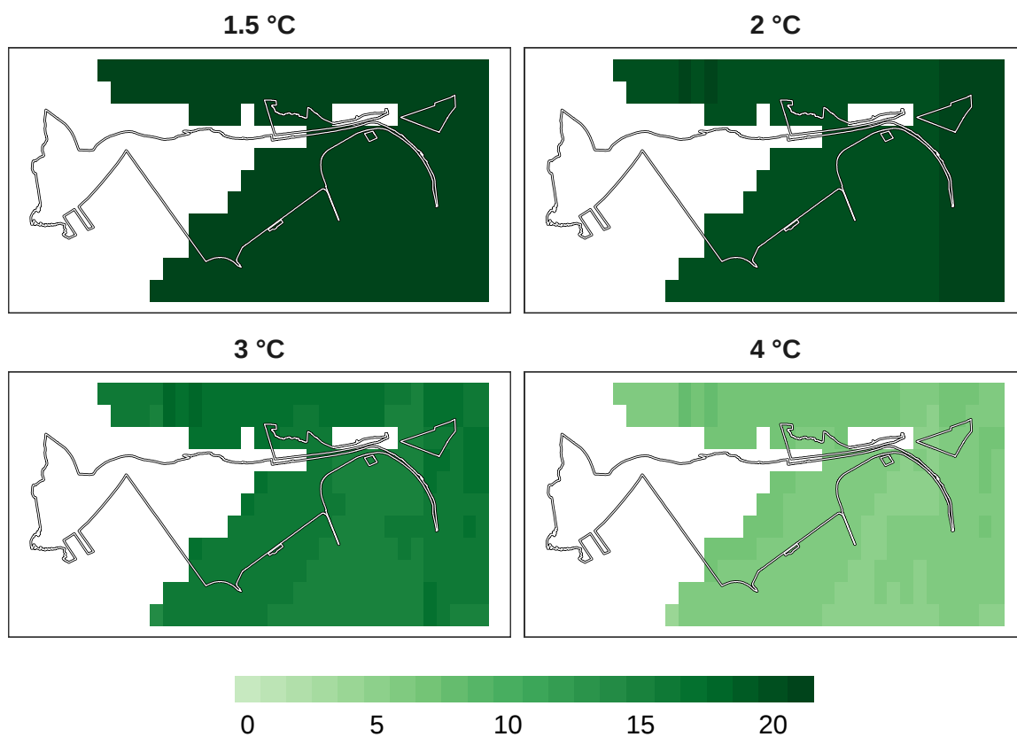
Figure 11: Number of models in agreement for plant refugia at 1 km resolution.
