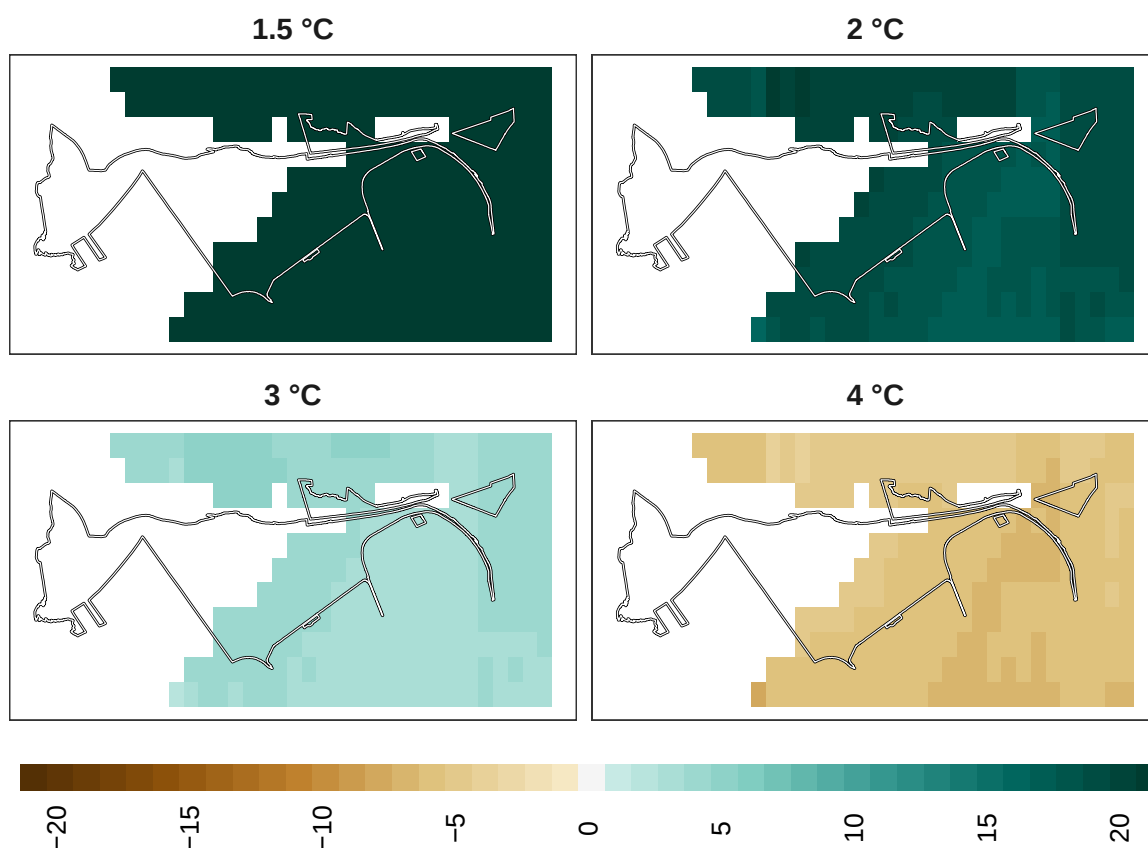
Figure 25: Adaptation effort for pollinators at 1 km resolution.
