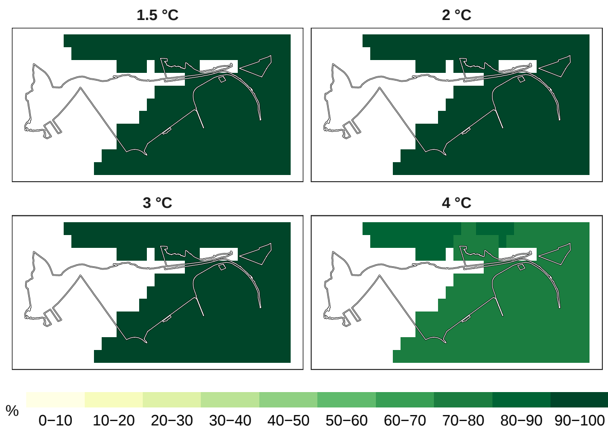
Figure 9: Percent timber species remaining at 1 km resolution.
