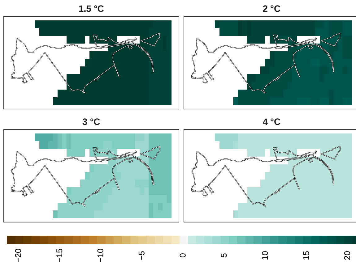
Figure 20: Adaptation effort for amphibians at 1 km resolution.
