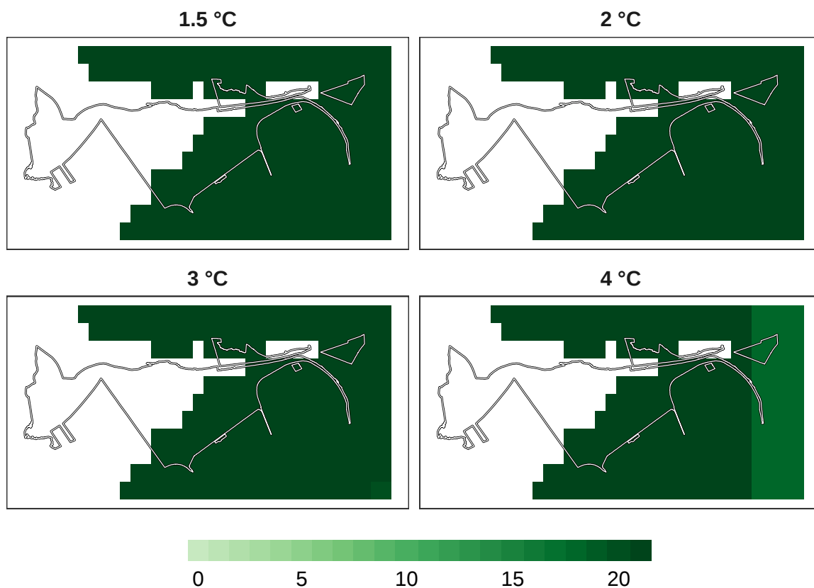
Figure 15: Number of models in agreement for reptile refugia at 1 km resolution.
