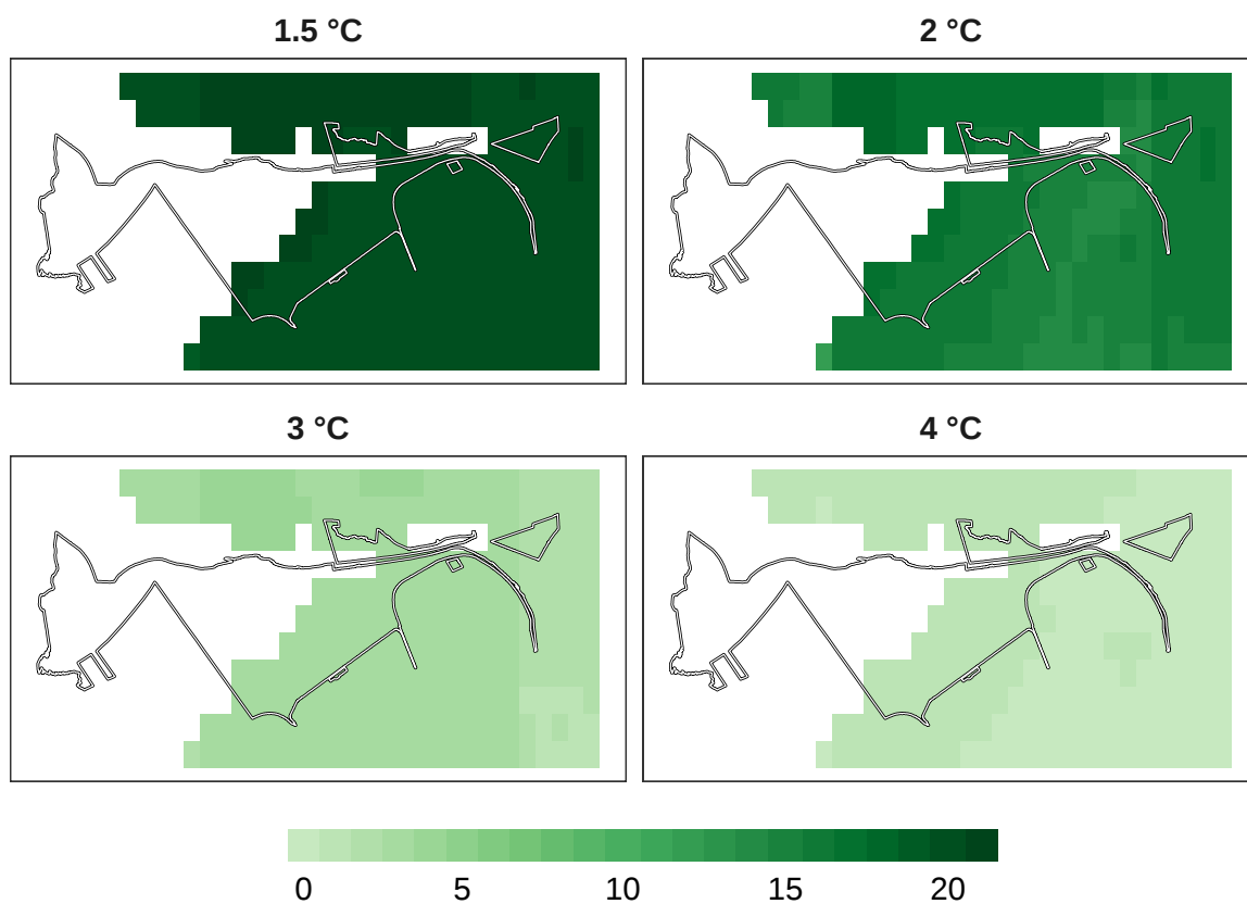
Figure 16: Number of models in agreement for insect refugia at 1 km resolution.
