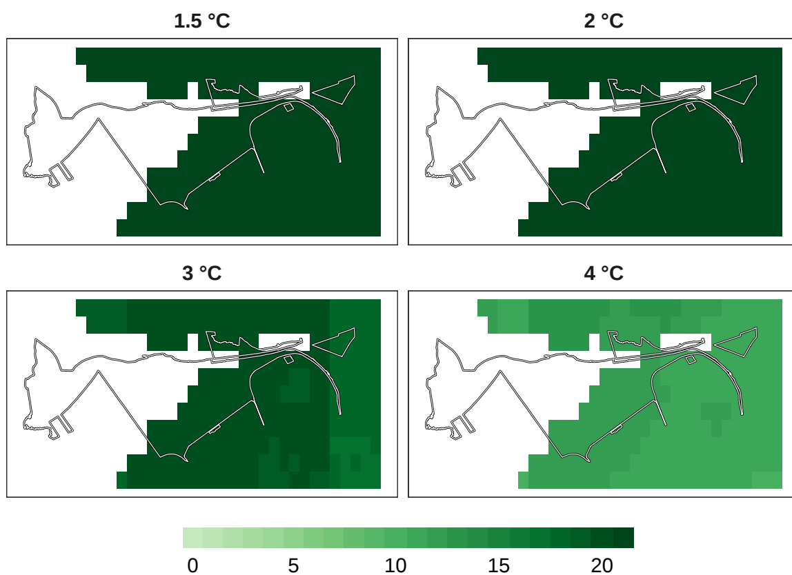
Figure 14: Number of models in agreement for mammal refugia at 1 km resolution.
