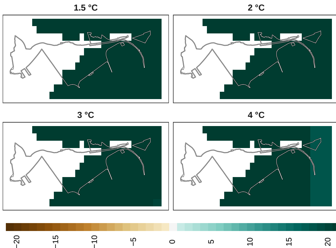
Figure 23: Adaptation effort for reptiles at 1 km resolution.
