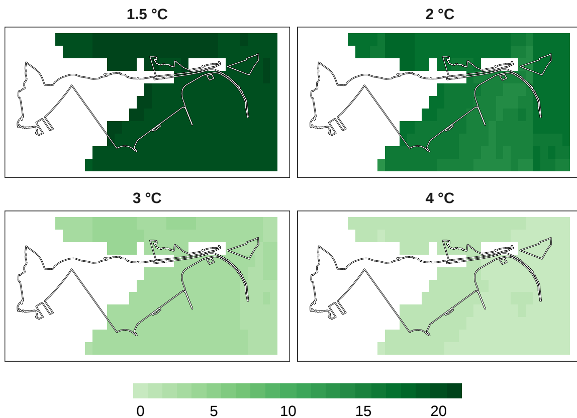
Figure 10: Number of models in agreement for overall biodiversity refugia at 1 km resolution.
