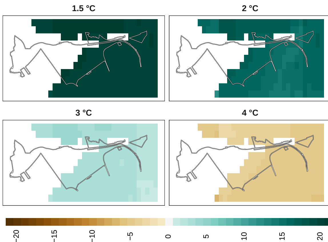
Figure 24: Adaptation effort for insects at 1 km resolution.
