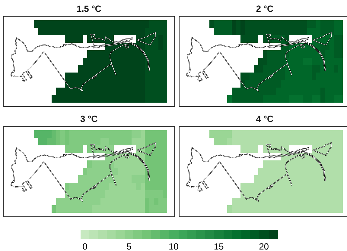
Figure 12: Number of models in agreement for amphibian refugia at 1 km resolution.
