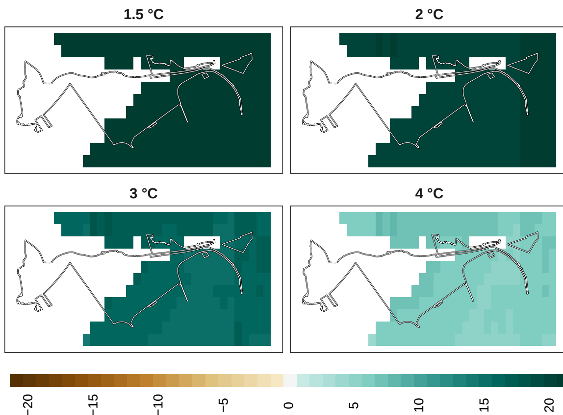
Figure 19: Adaptation effort for plants at 1 km resolution.
