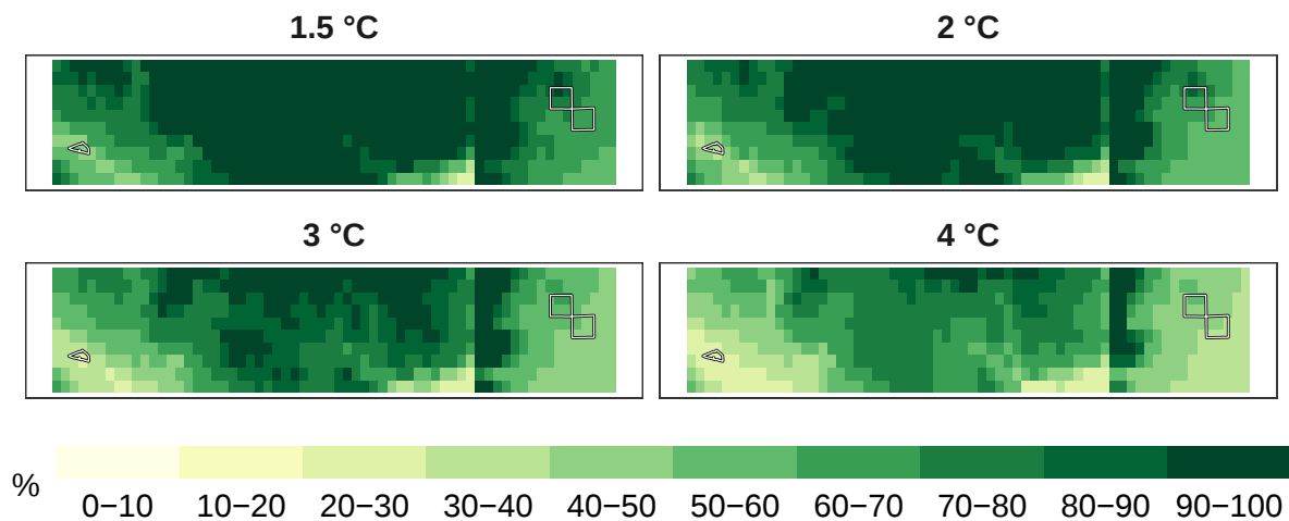
Figure 1: Percent overall biodiversity remaining at 1 km resolution.
